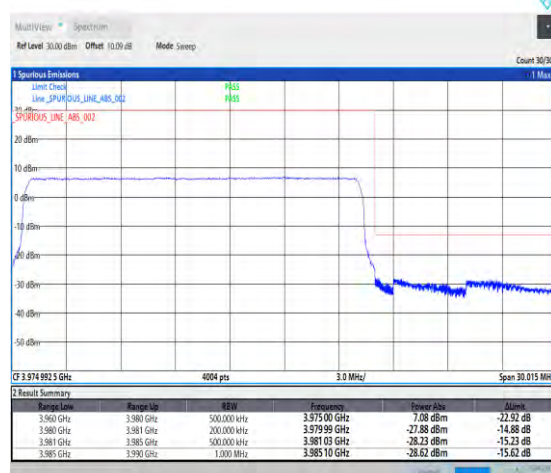
1-N77-3700-3980--30-20-H-6-CP-QPSK-Outer_Fu ll-51@0-Ant2-PASS-see graph
