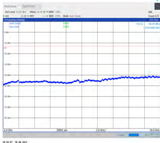
1-N77-3700-3980--30-100-M-1-DFT-QPSK-Edge_1R B_Left-1@0-6000-26000-Ant2--40.28--13-PASS
