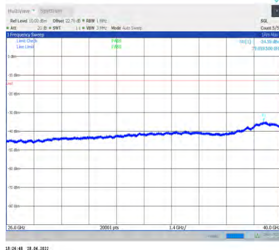
1-N77-3700-3980--30-100-M-1-DFT-QPSK-Edge_1R B_Left-1@0-26000-40000-Ant2--34.58--13-PASS
