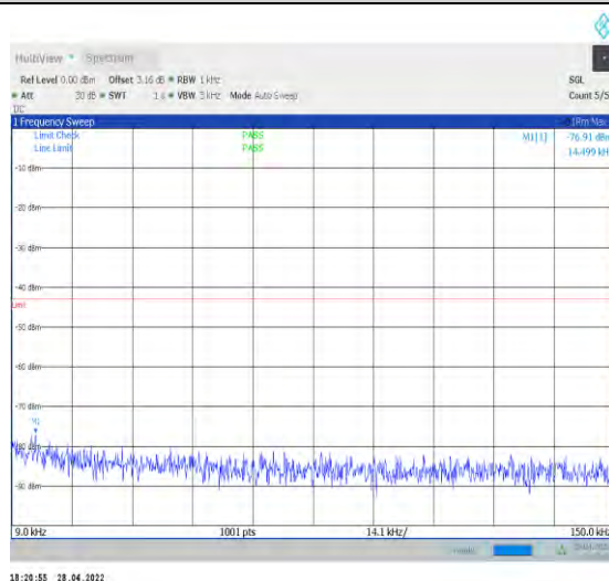
1-N77-3700-3980--30-100-M-1-DFT-QPSK-Edge_1R B_Left-1@0-0.009-0.15-Ant1--76.91--43-PASS
