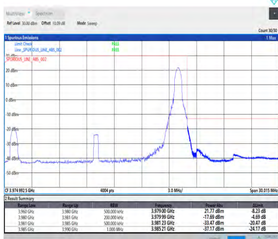
1-N77-3700-3980--30-20-H-5-CP-QPSK-Edge_1RB_Ri ght-1@50-Ant2-PASS-see graph
