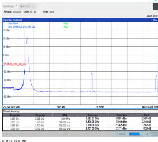
1-N77-3700-3980--30-60-L-4-CP-QPSK-Edge_1RB_Le ft-1@0-Ant2-PASS-see graph
