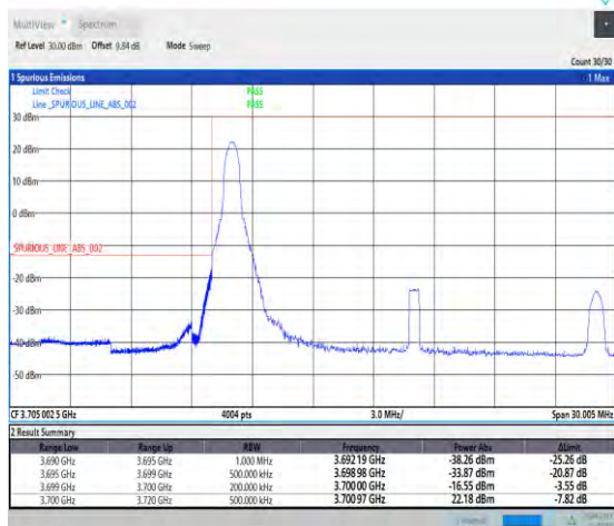
1-N77-3700-3980--30-20-L-4-CP-QPSK-Edge_1RB_Le ft-1@0-Ant2-PASS-see graph
