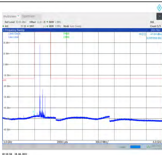
1-N77-3700-3980--30-100-L-1-DFT-QPSK-Edge_1R B_Left-1@0-3000-6000-Ant1--47.04--13-PASS
