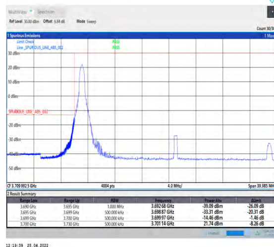
1-N77-3700-3980--30-30-L-4-CP-QPSK-Edge_1RB_Left-1@0-Ant1-PASS-see graph
