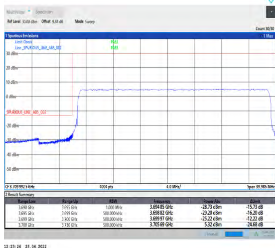
1-N77-3700-3980--30-30-L-6-CP-QPSK-Outer_Full-78@0-Ant1-PASS-see graph
