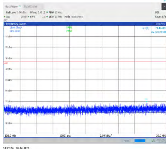
1-N77-3700-3980--30-100-H-1-DFT-QPSK-Edge_1R B_Left-1@0-0.15-30-Ant2--71.15--33-PASS
