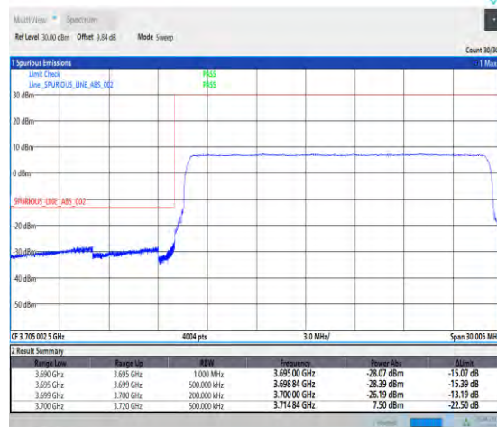
1-N77-3700-3980--30-20-L-6-CP-QPSK-Outer_Ful I-51@0-Ant2-PASS-see graph
