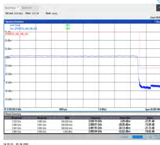
1-N77-3700-3980--30-60-H-6-CP-QPSK-Outer_Fu ll-162@0-Ant2-PASS-see graph
