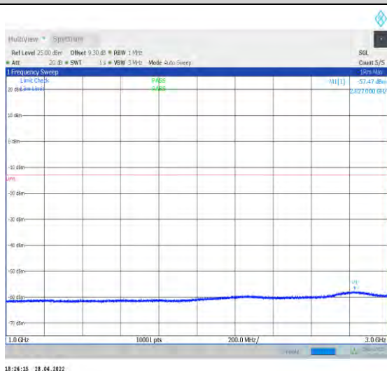
1-N77-3700-3980--30-100-M-1-DFT-QPSK-Edge_1R B_Left-1@0-1000-3000-Ant2--57.47--13-PASS
