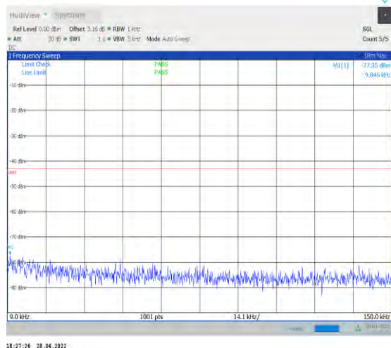
1-N77-3700-3980--30-100-H-1-DFT-QPSK-Edge_1R B_Left-1@0-0.009-0.15-Ant2--77.35--43-PASS
