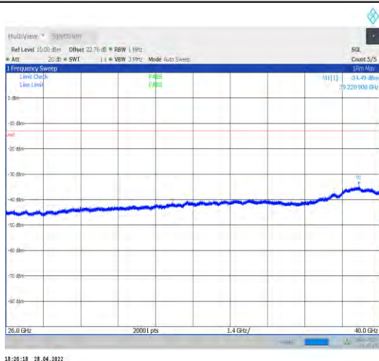
1-N77-3700-3980--30-100-L-1-DFT-QPSK-Edge_1R B_Left-1@0-26000-40000-Ant1--34.49--13-PASS
