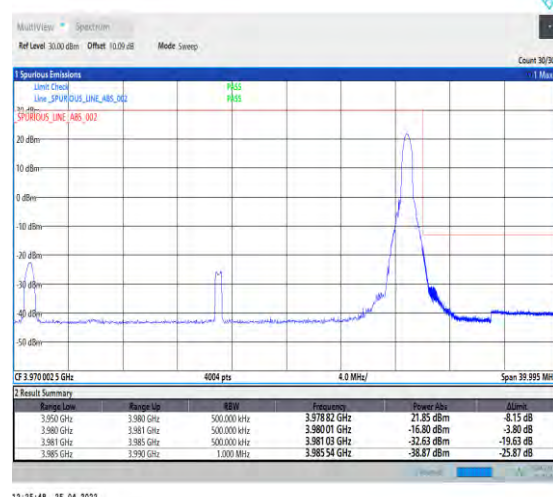
1-N77-3700-3980--30-30-H-5-CP-QPSK-Edge_1RB_Right-1@77-Ant1-PASS-see graph
