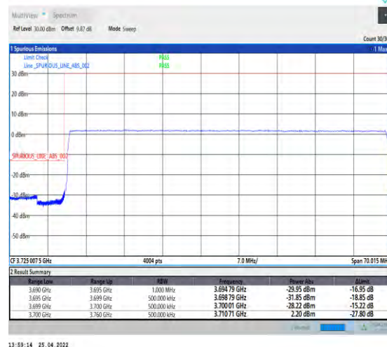
1-N77-3700-3980--30-60-L-6-CP-QPSK-Outer_Ful I-162@0-Ant2-PASS-see graph
