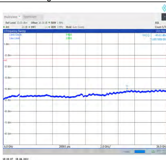
1-N77-3700-3980--30-100-L-1-DFT-QPSK-Edge_1R B_Left-1@0-6000-26000-Ant1--40.61--13-PASS
