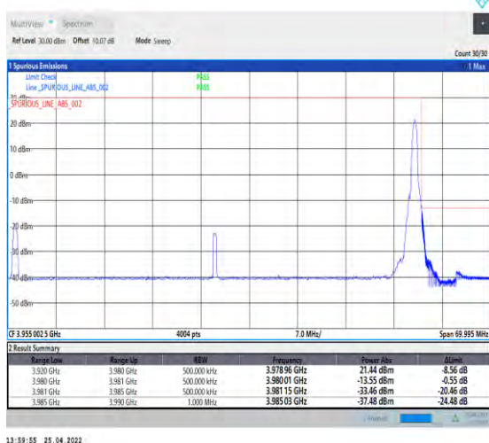
1-N77-3700-3980--30-60-H-5-CP-QPSK-Edge_1RB_Ri ght-1@161-Ant2-PASS-see graph
