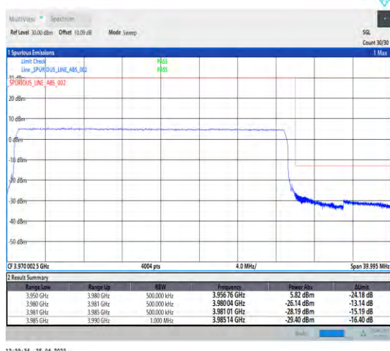
1-N77-3700-3980--30-30-H-6-CP-QPSK-Outer_Full-78@0-Ant1-PASS-see graph
