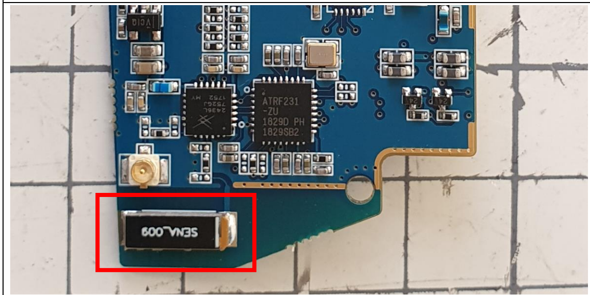
MESH Antenna 1 (M/N: SENA_009)
