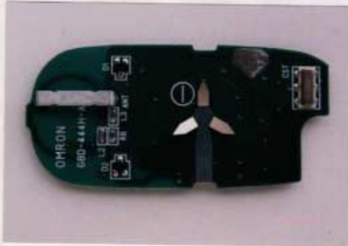
Figure 8.4 PCB assy (back view)
