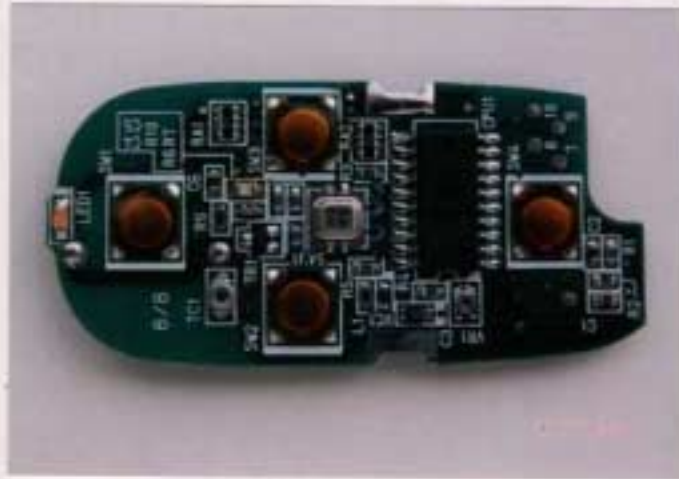
Figure 8.3 PCB map (front view)
