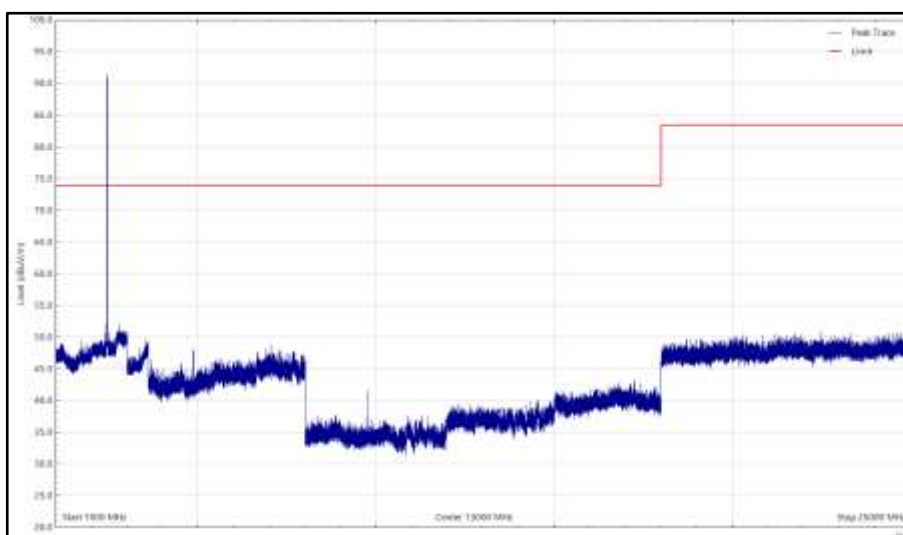
Figure 48 - 802.11b - X, 2437 MHz, 1 GHz to 25 GHz, Horizontal (Peak)
