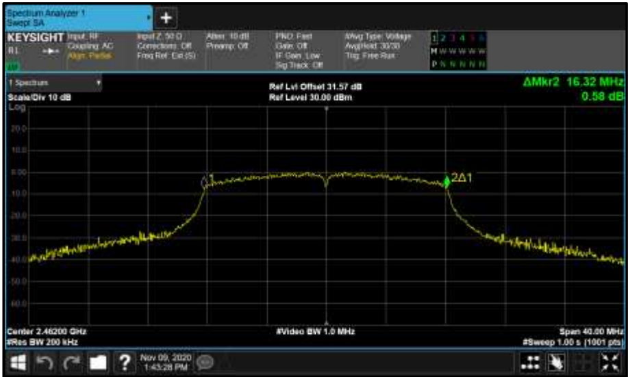
Figure 22 - Core 0 (A) 2462 MHz (CH11) 99% Bandwidth
