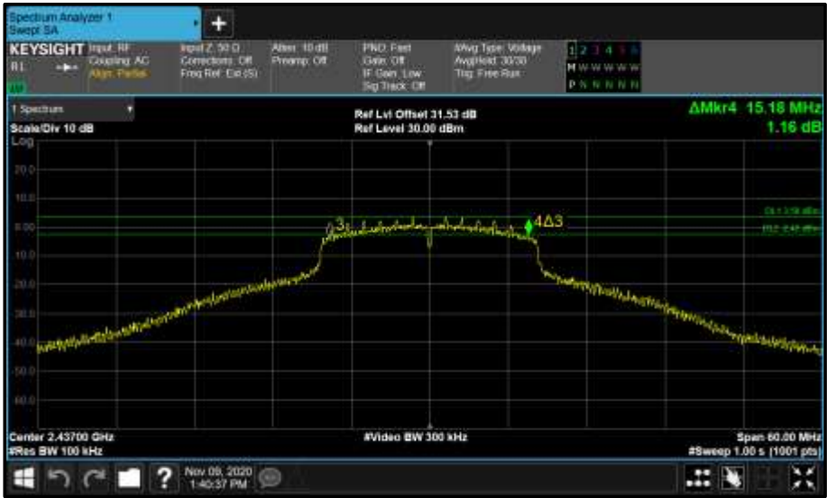
Figure 21 - Core 0 (A) 2437 MHz (CH6) 6 dB Bandwidth
