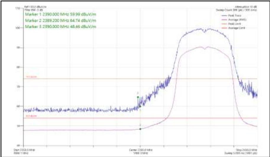
Figure 5 - 802.11n HT20 2412 MHz, Band Edge Frequency 2390 MHz
