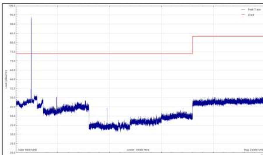
Figure 156 - 802.11b - Z, 2437 MHz, 1 GHz to 25 GHz, Horizontal (Peak)
