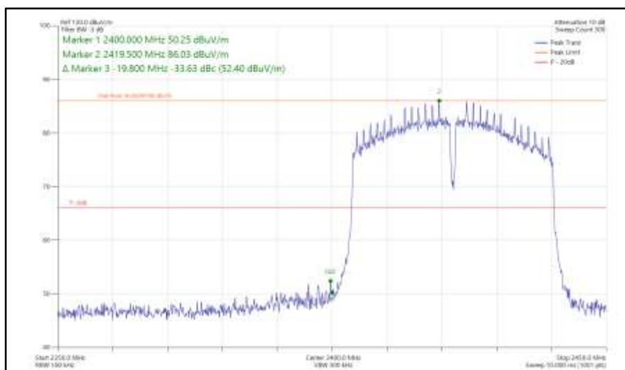
Figure 39 - 802.11n HT40 Core 0 - 2422 MHz Band Edge Frequency 2400 MHz
