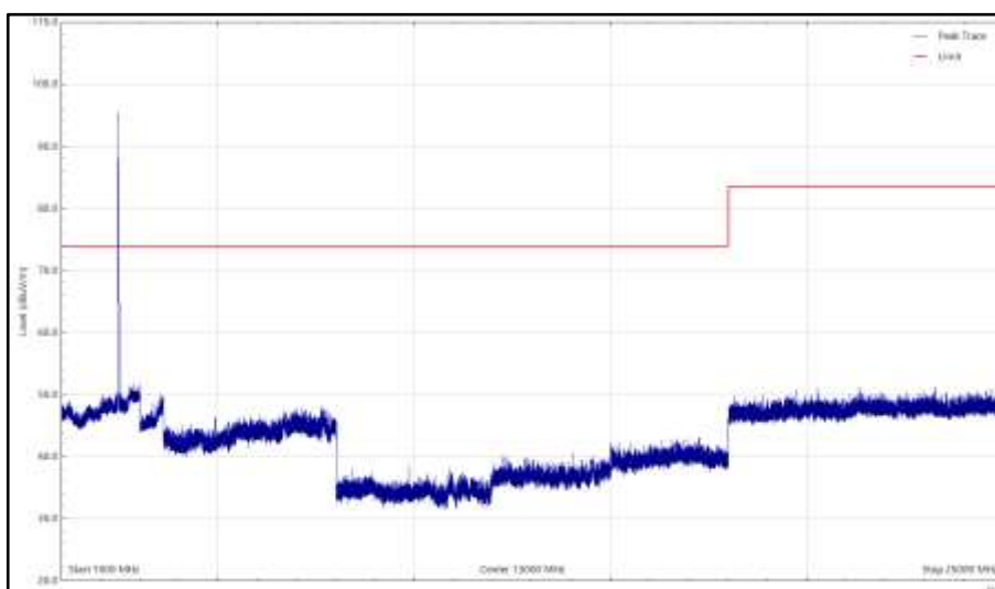
Figure 108 - 802.11b - Y, 2462 MHz, 1 GHz to 25 GHz, Horizontal (Peak)
