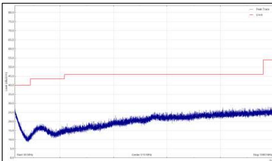
Figure 65 - 802.11g - X, 2437 MHz, 30 MHz to 1 GHz, Horizontal (Peak)
