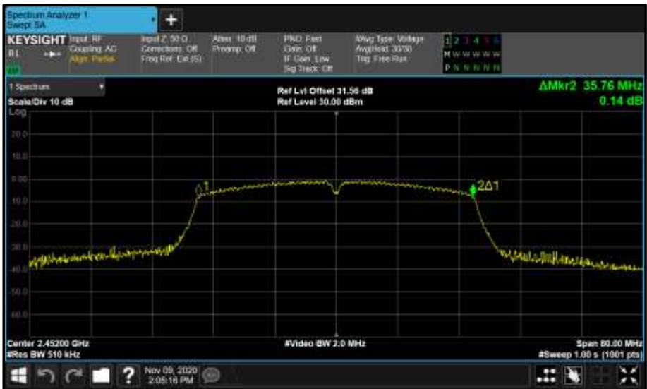
Figure 34 - Core 0 (A) 2452 MHz (CH9) 99% Bandwidth
