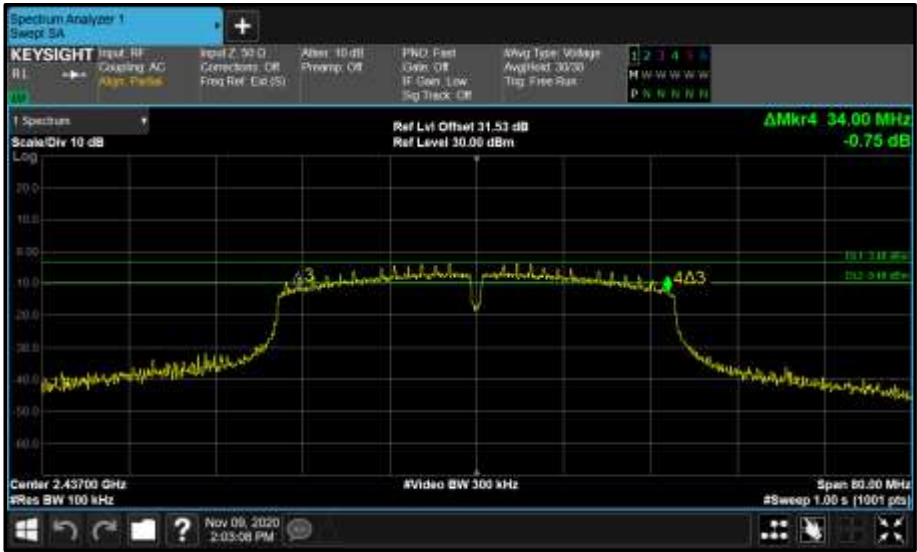
Figure 33 - Core 0 (A) 2437 MHz (CH6) 6 dB Bandwidth
