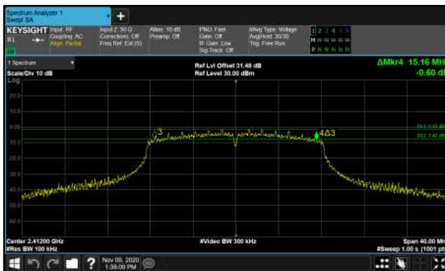
Figure 19 - Core 0 (A) 2412 MHz (CH1) 6 dB Bandwidth
