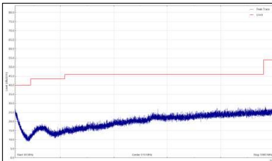
Figure 185 - 802.11n20 - Z, 2412 MHz, 30 MHz to 1 GHz, Horizontal (Peak)
