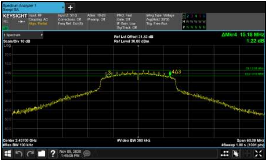
Figure 27 - Core 0 (A) 2437 MHz (CH6) 6 dB Bandwidth
