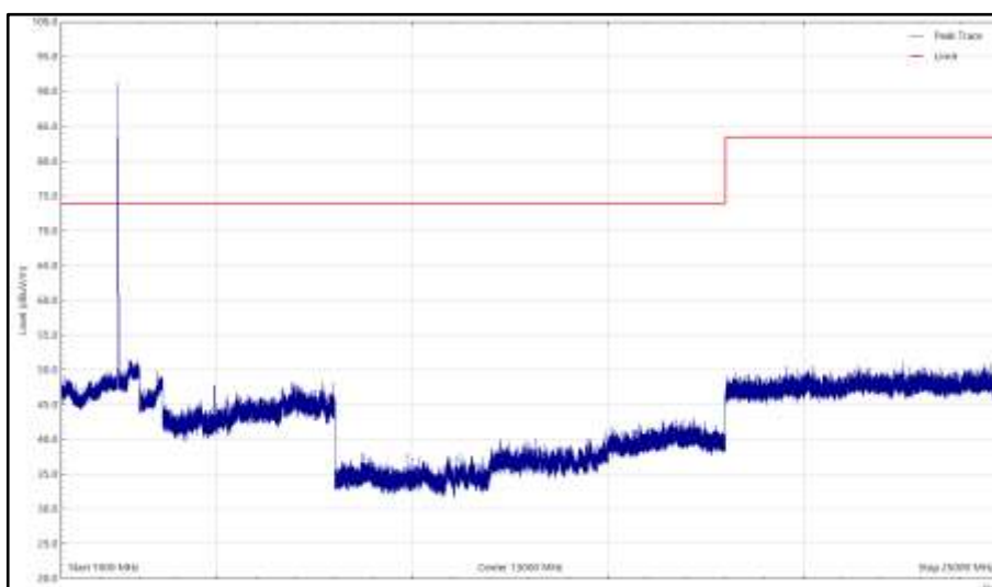
Figure 54 - 802.11b - X, 2462 MHz, 1 GHz to 25 GHz, Horizontal (Peak)
