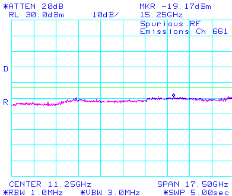
Figure 4: PCS, Spurious Conducted Emissions, Middle Channel
