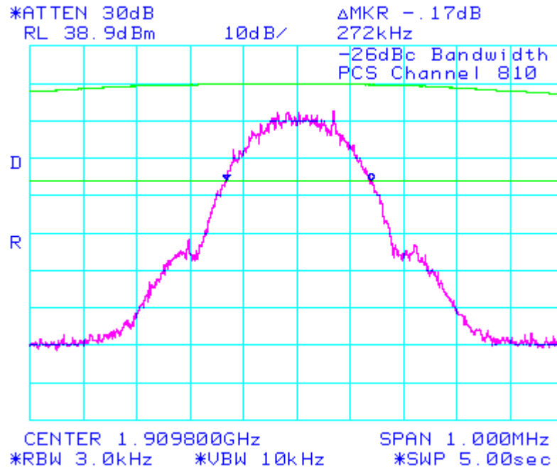
Figure 11: -26dBc bandwidth, PCS High Channel
