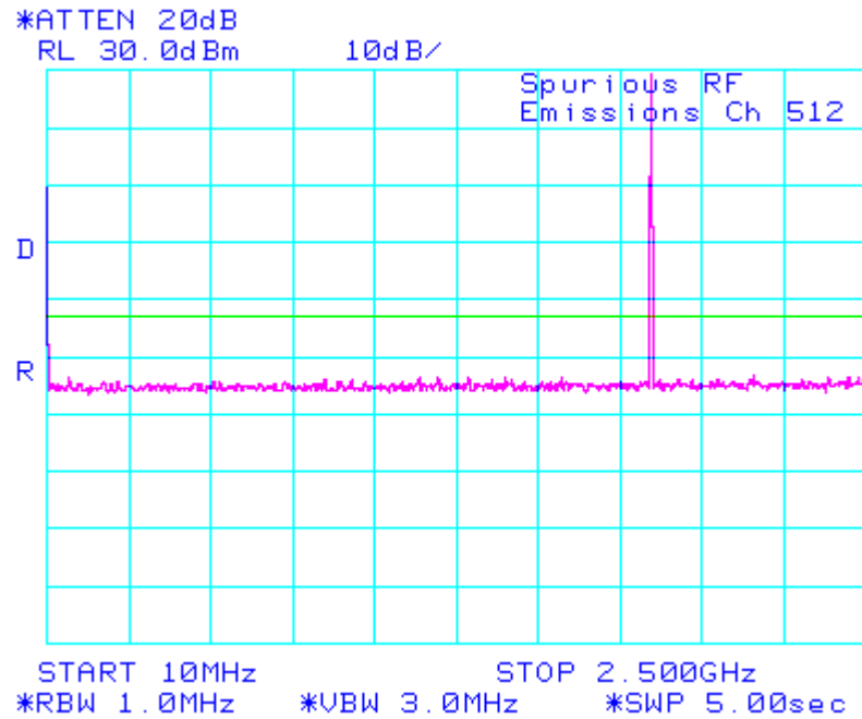
Figure 1: PCS, Spurious Conducted Emissions, Low channel
