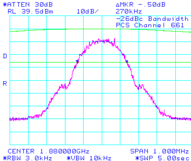
Figure 9: -26dBc bandwidth, PCS Middle Channel
