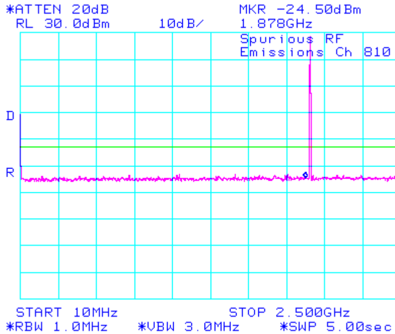
Figure 5: PCS, Spurious Conducted Emissions, High Channel
