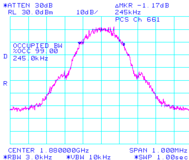
Figure 10: Occupied Bandwidth, PCS Middle Channel
