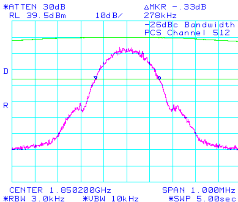
Figure 7: -26dBc bandwidth, PCS Low Channel
