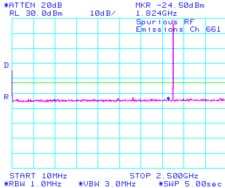
Figure 3: PCS, Spurious Conducted Emissions, Middle Channel
