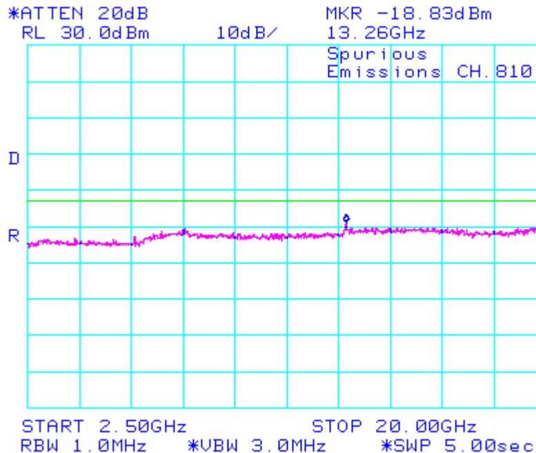
Figure 6: PCS, Spurious Conducted Emissions, High Channel
