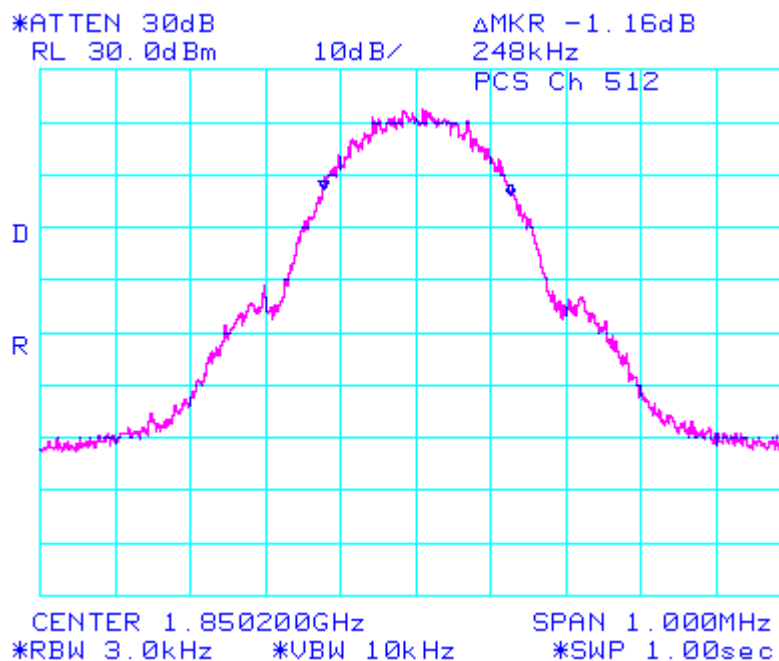
Figure 8: Occupied Bandwidth, PCS Low Channel
