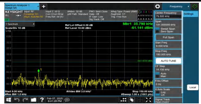
Band4-5MHz-QPSK-19975-1RB#24-0.009~0.15-PASS
