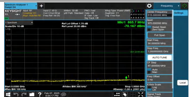
Band4-10MHz-QPSK-20350-1RB#49-30~1000-PASS
