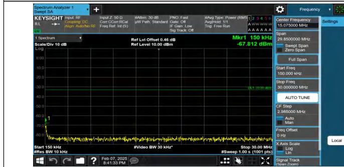
Band4-5MHz-QPSK-19975-1RB#24-0.15~30-PASS
