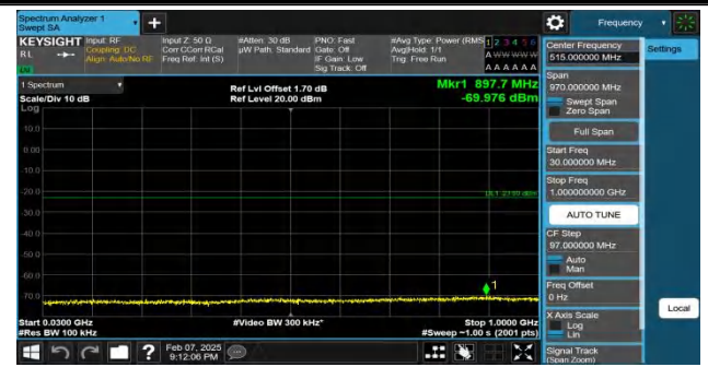
Band4-20MHz-QPSK-20300-1RB#99-30~1000-PASS
