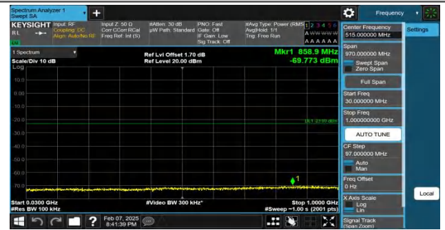
Band4-5MHz-QPSK-19975-1RB#24-30~1000-PASS
