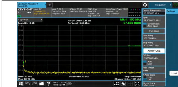
Band4-15MHz-QPSK-20325-1RB#74-0.15~30-PASS
