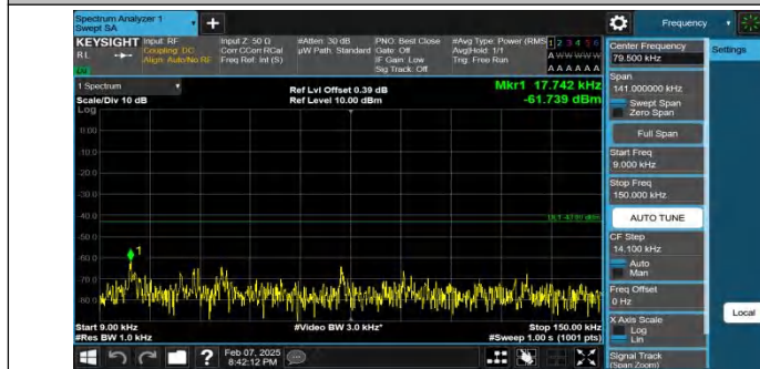
Band4-5MHz-QPSK-20175-1RB#0-0.009~0.15-PASS
