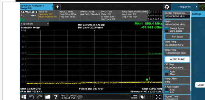
Band4-20MHz-QPSK-20050-1RB#0-30~1000-PASS
