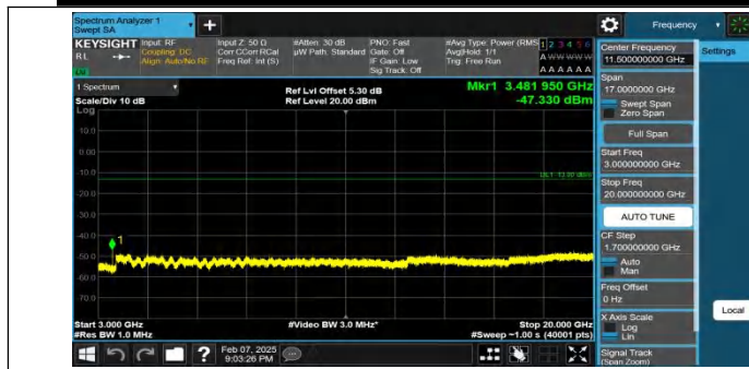
Band4-15MHz-QPSK-20325-1RB#0-3000~20000-PASS
