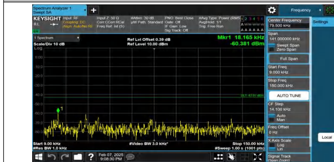
Band4-20MHz-QPSK-20050-1RB#0-0.009~0.15-PASS
