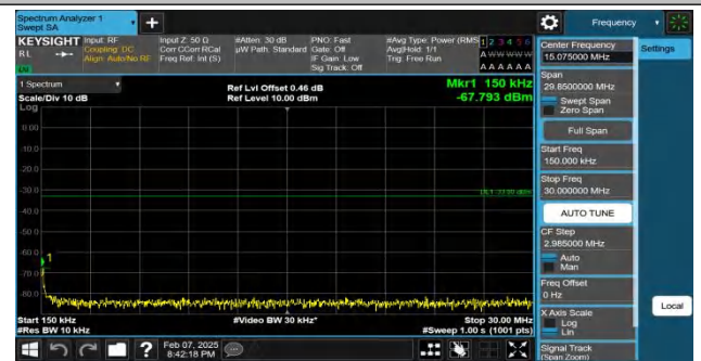
Band4-5MHz-QPSK-20175-1RB#0-0.15~30-PASS
