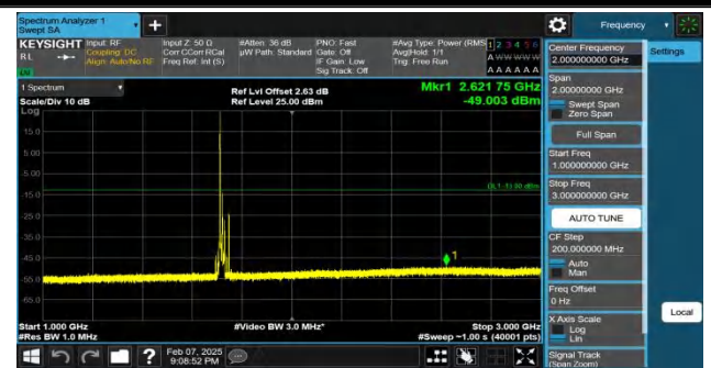
Band4-20MHz-QPSK-20050-1RB#0-1000~3000-PASS
