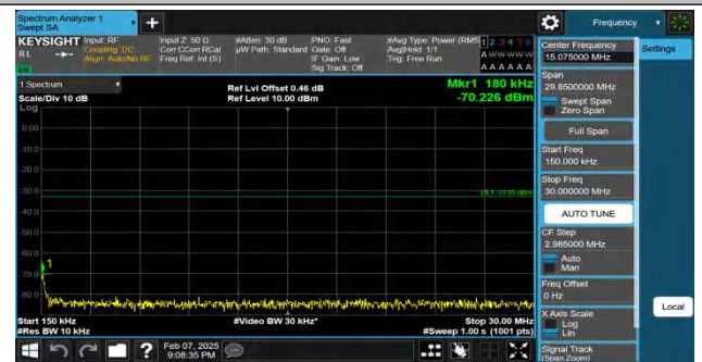
Band4-20MHz-QPSK-20050-1RB#0-0.15~30-PASS
