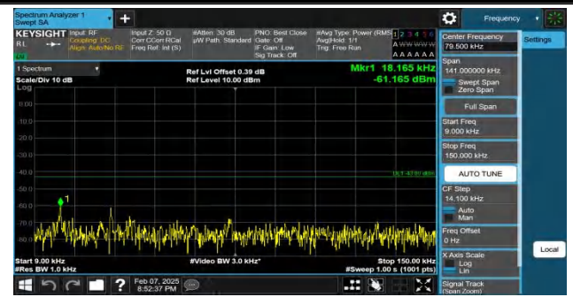
Band4-10MHz-QPSK-20175-1RB#49-0.009~0.15-PASS
