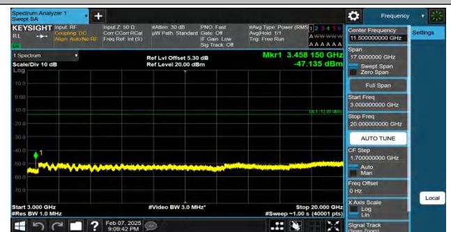
Band4-20MHz-QPSK-20050-1RB#99-3000~20000-PASS
