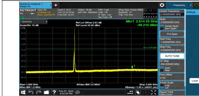
Band4-10MHz-QPSK-20175-1RB#49-1000~3000-PASS
