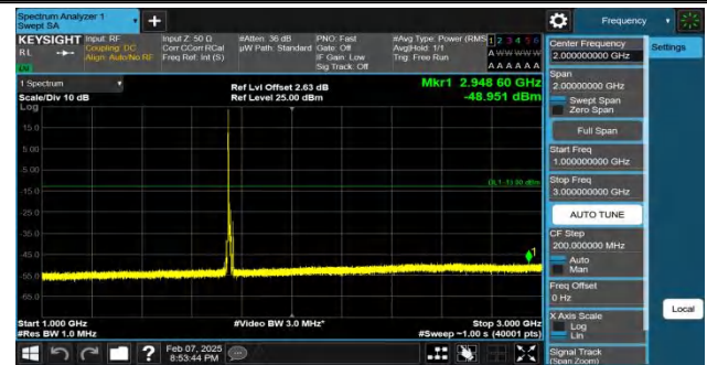
Band4-10MHz-QPSK-20350-1RB#0-1000~3000-PASS
