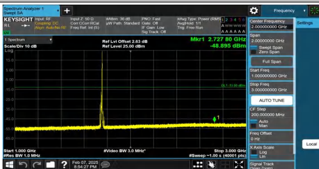
Band4-10MHz-QPSK-20350-1RB#49-1000~3000-PASS
