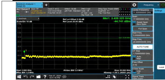
Band4-5MHz-QPSK-19975-1RB#0-3000~20000-PASS
