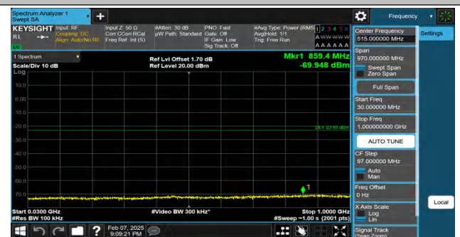
Band4-20MHz-QPSK-20050-1RB#99-30~1000-PASS
