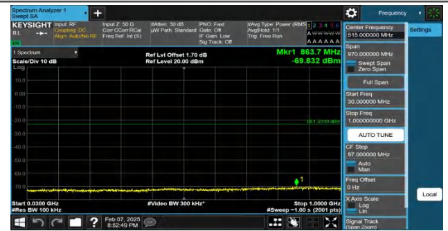
Band4-10MHz-QPSK-20175-1RB#49-30~1000-PASS
