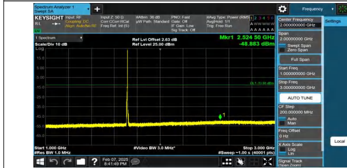
Band4-5MHz-QPSK-19975-1RB#24-1000~3000-PASS
