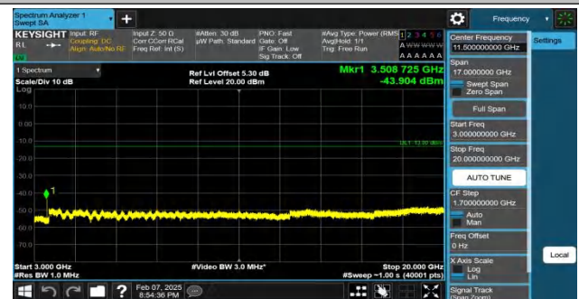
Band4-10MHz-QPSK-20350-1RB#49-3000~20000-PASS
