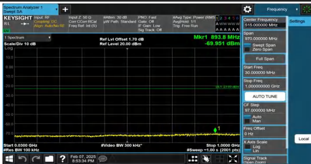
Band4-10MHz-QPSK-20350-1RB#0-30~1000-PASS
