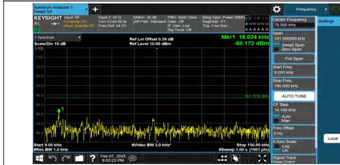
Band4-10MHz-QPSK-20350-1RB#0-0.009~0.15-PASS
