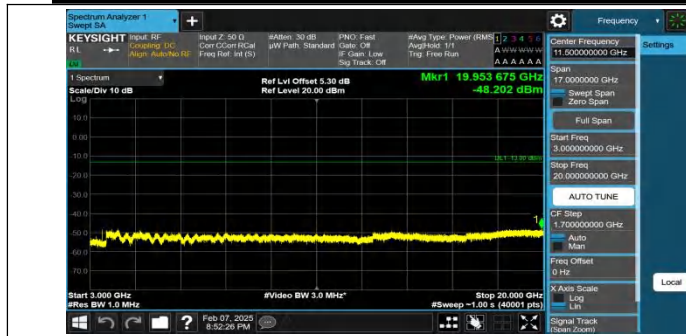
Band4-10MHz-QPSK-20175-1RB#0-3000~20000-PASS
