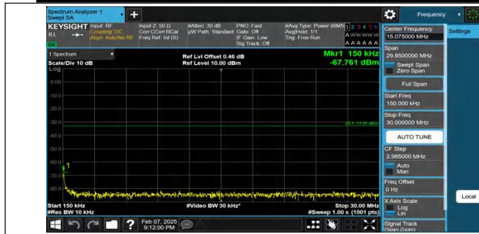
Band4-20MHz-QPSK-20300-1RB#99-0.15~30-PASS
