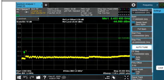
Band4-20MHz-QPSK-20050-1RB#0-3000~20000-PASS
