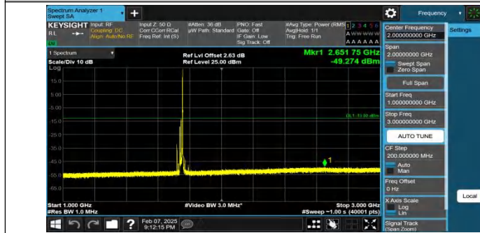
Band4-20MHz-QPSK-20300-1RB#99-1000~3000-PASS
