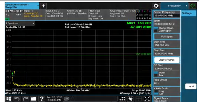
Band4-3MHz-QPSK-20385-1RB#0-0.15~30-PASS
