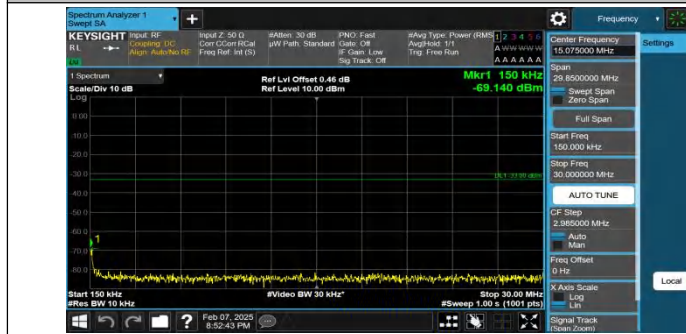
Band4-10MHz-QPSK-20175-1RB#49-0.15~30-PASS
