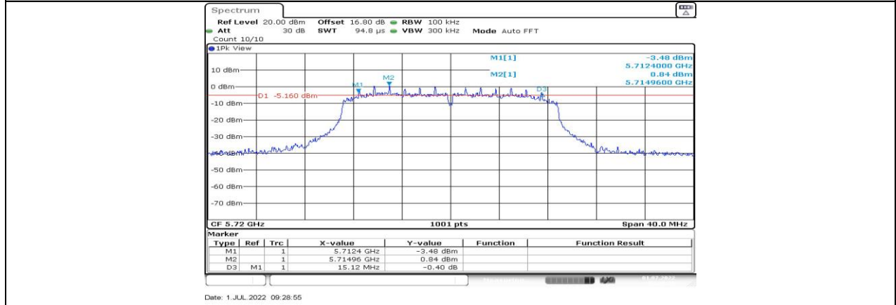
11N20SISO_Ant1_5720_UNII-3
