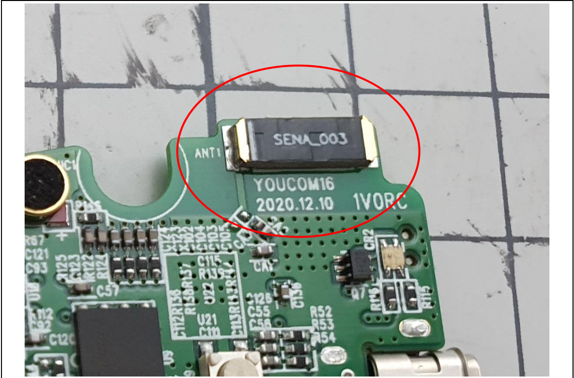
MESH Antenna
