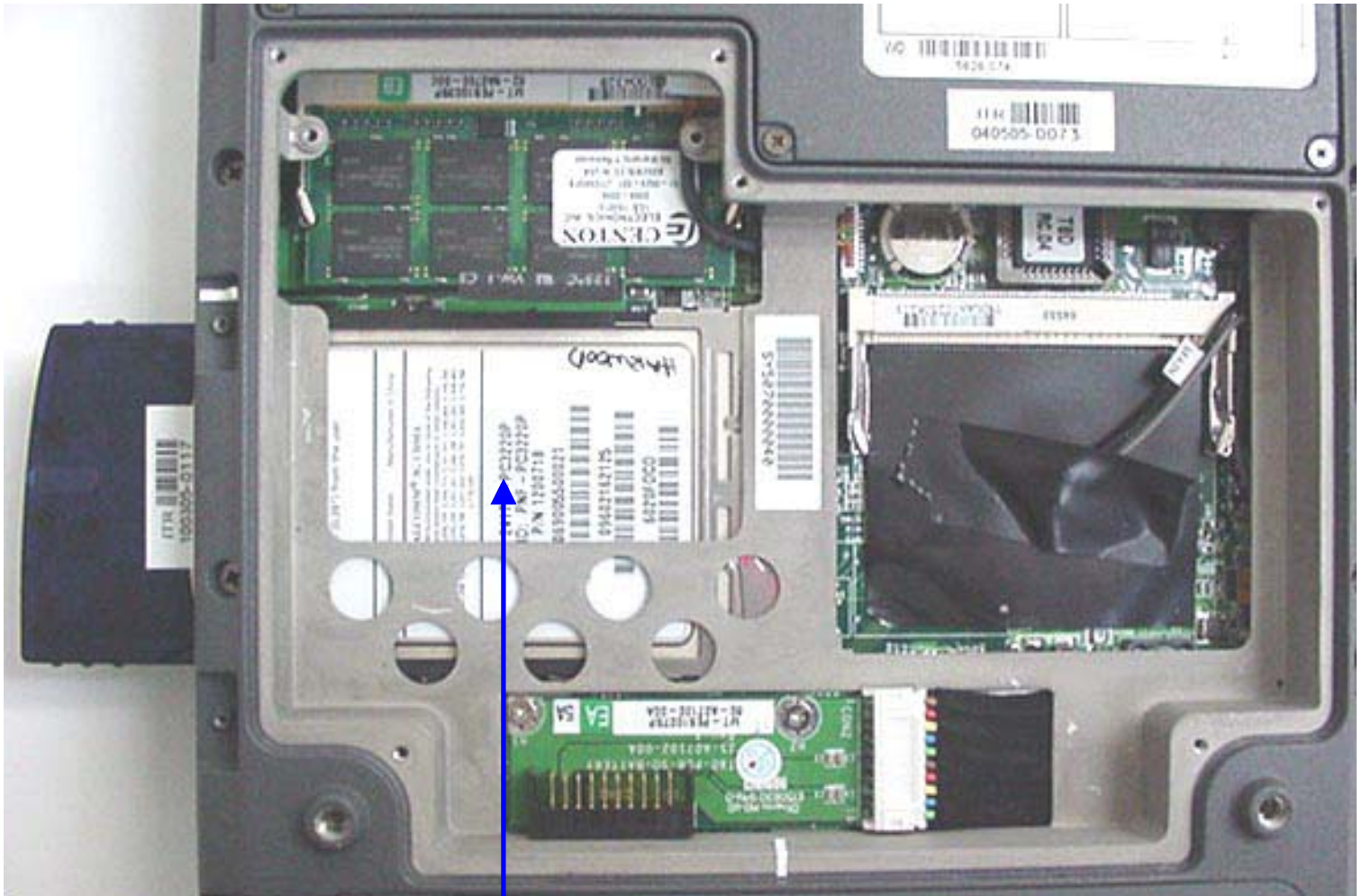
Sierra Wireless AirCard 580 CDMA PCMCIA Modem
