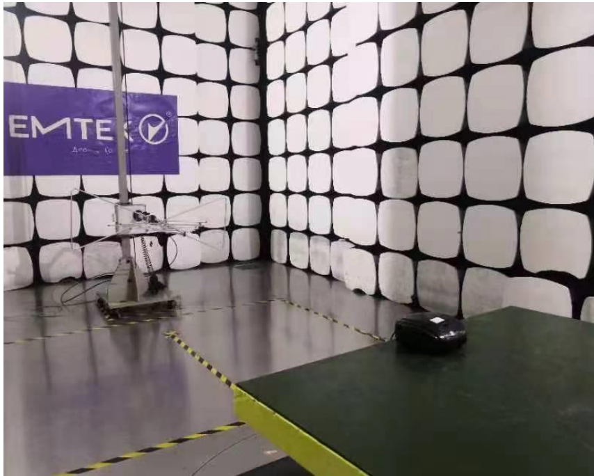
Spurious Emission Test Setup (Below 1GHz)
