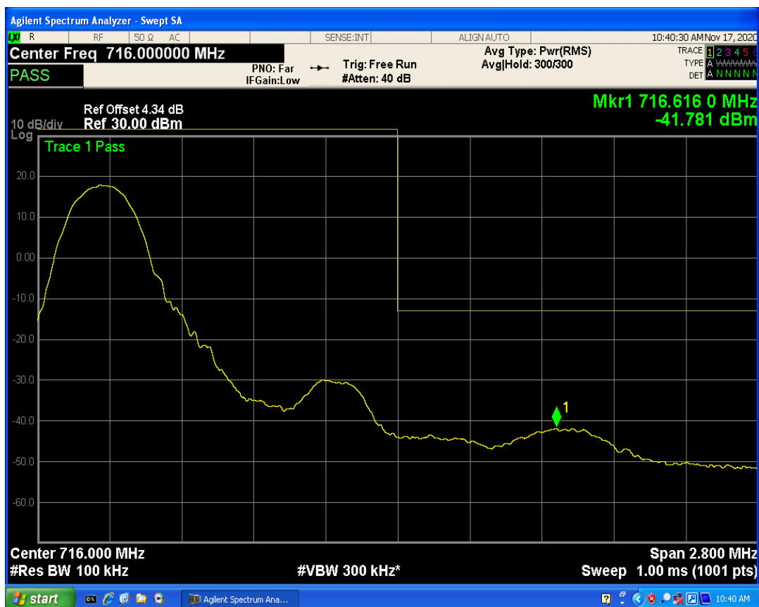
LTE Band12 QAM16 BW=1.4MHz Channel=23173 RB Size=1 Position=#Max
