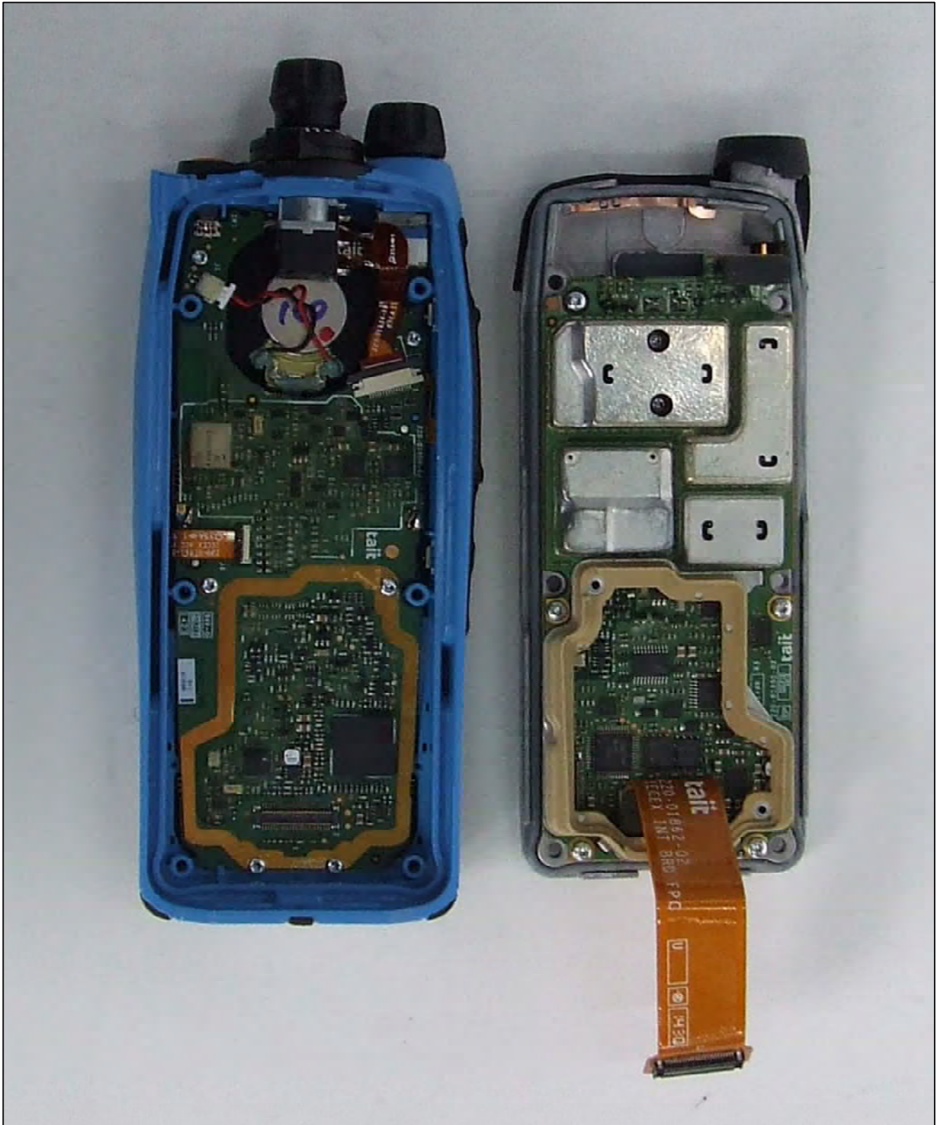
Photograph 01: PCBs Top
