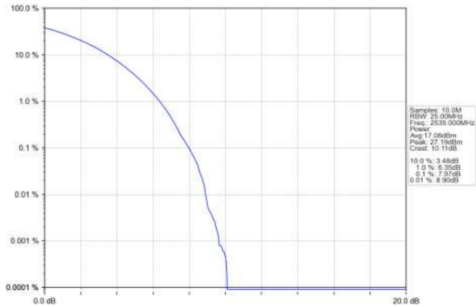
n7_30kHz_SISO_NTNV_15MHz_CP-OFDM_16_QAM_2535MHz_Outer_Full_Ant1
