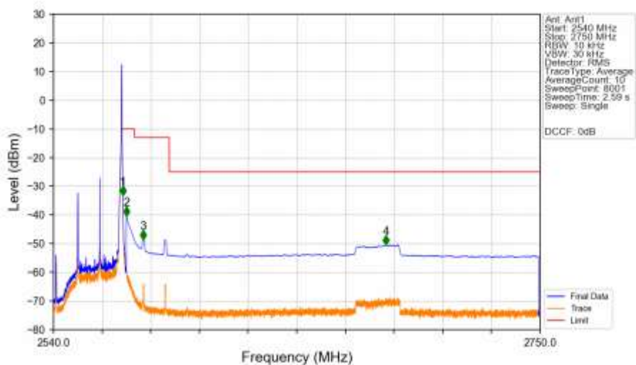
n7_15kHz_SISO_NTNV_20MHz_DFT-s-OFDM_QPSK_2560MHz_Edge_1RB_Right_Ant1
