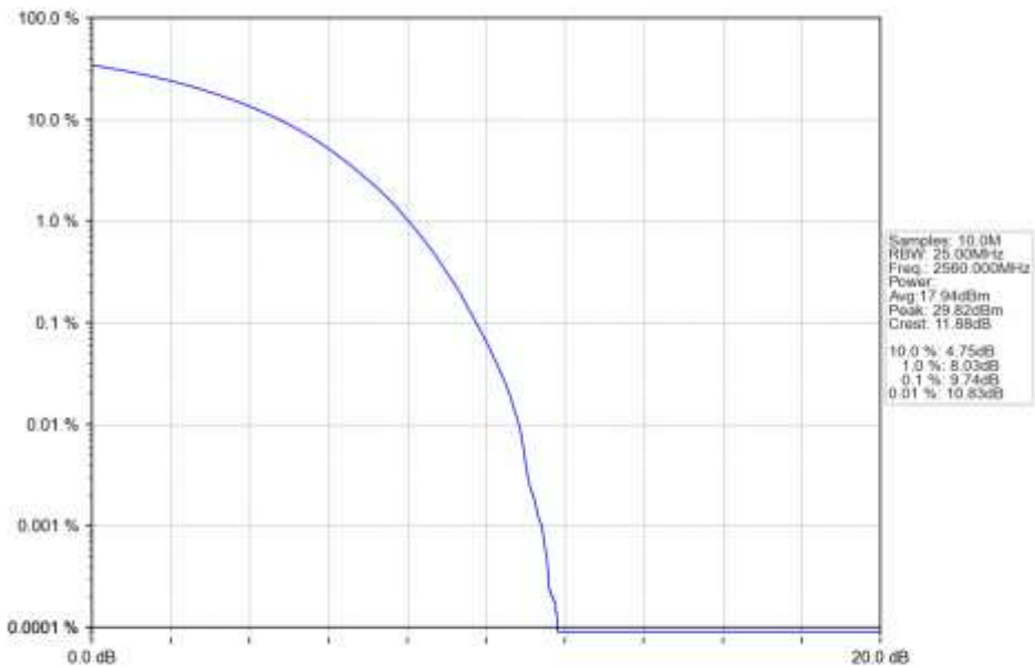
n7_15kHz_SISO_NTNV_20MHz_CP-OFDM_64_QAM_2560MHz_Outer_Full_Ant1
