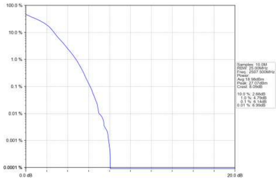
n7_30kHz_SISO_NTNV_15MHz_DFT-s-OFDM_16_QAM_2507.5MHz_Outer_Full_Ant1
