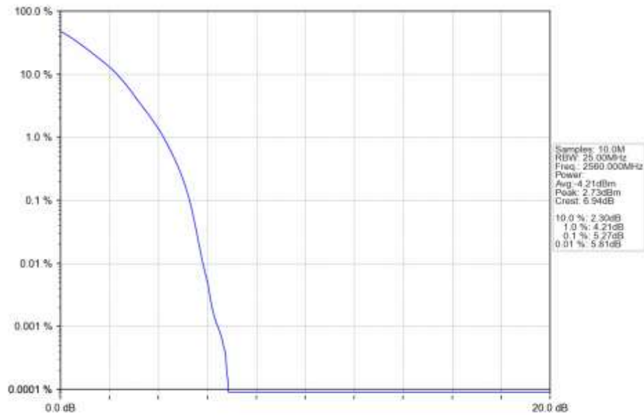
n7_30kHz_SISO_NTNV_20MHz_DFT-s-OFDM_QPSK_2560MHz_Outer_Full_Ant1
