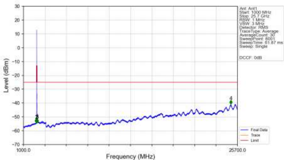
n7_15kHz_SISO_NTNV_10MHz_CP-OFDM_QPSK_2535MHz_Edge_1RB_Left_Ant1
