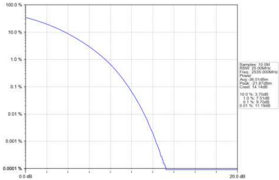
n7_30kHz_SISO_NTNV_15MHz_CP-OFDM_256_QAM_2535MHz_Outer_Full_Ant1
