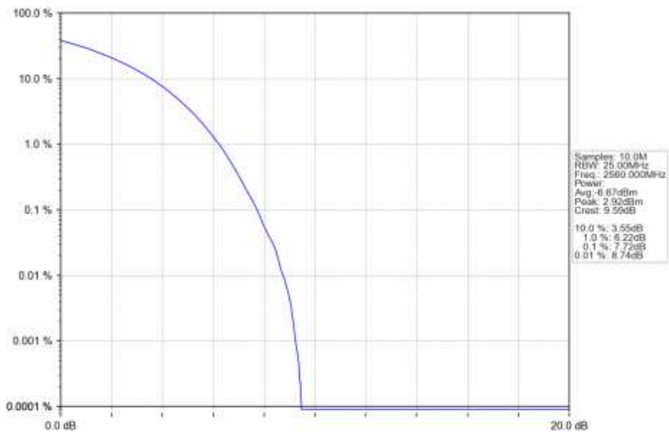
n7_30kHz_SISO_NTNV_20MHz_CP-OFDM_16_QAM_2560MHz_Outer_Full_Ant1
