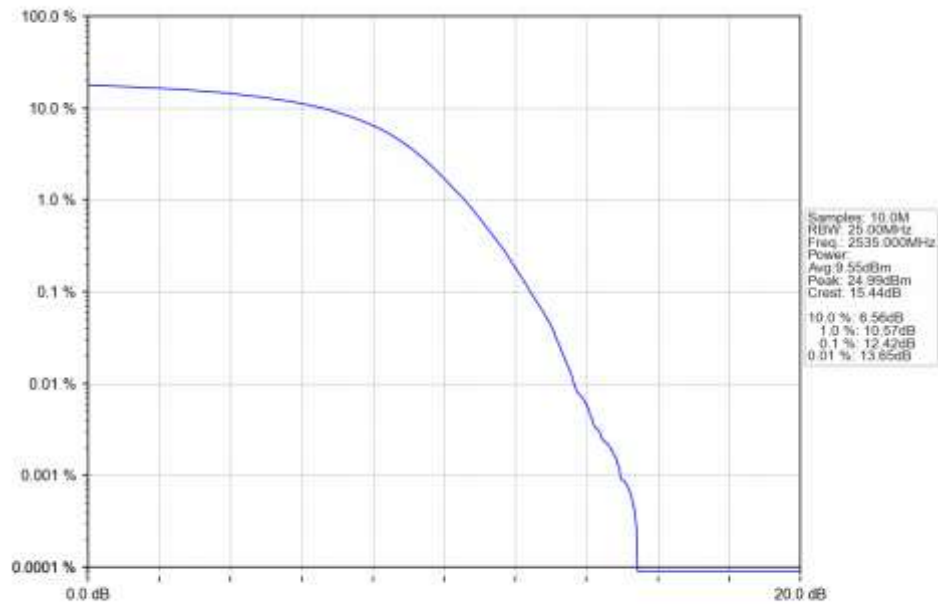
n7_30kHz_SISO_NTNV_15MHz_DFT-s-OFDM_256_QAM_2535MHz_Outer_Full_Ant1
