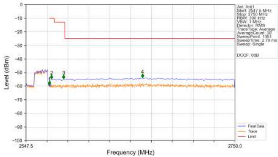
n7_30kHz_SISO_NTNV_15MHz_DFT-s-OFDM_QPSK_2562.5MHz_Outer_Full_Ant1
