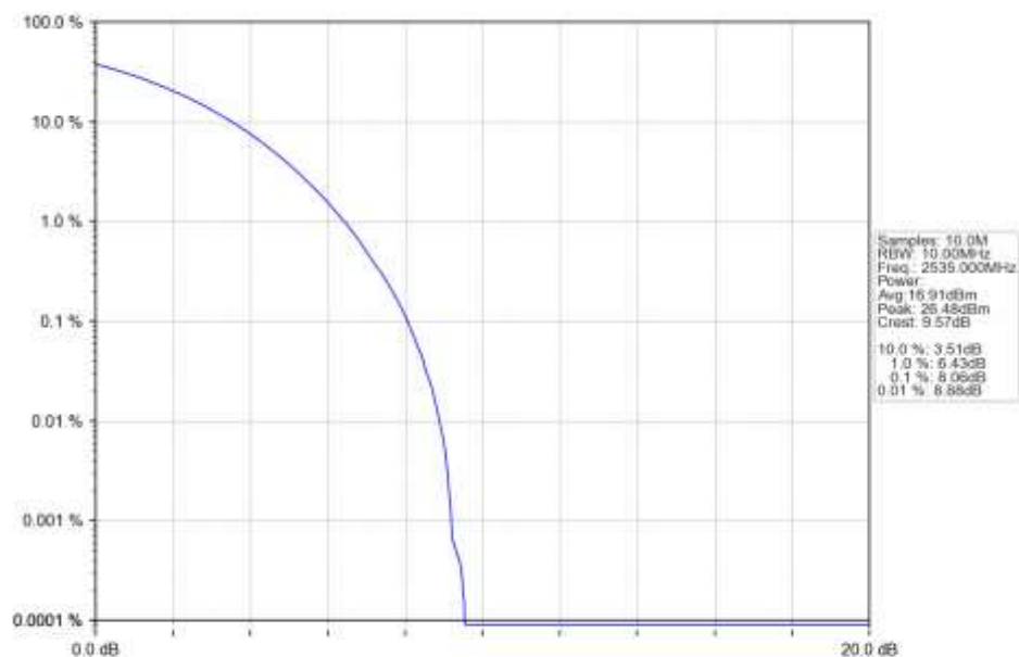
n7_30kHz_SISO_NTNV_10MHz_CP-OFDM_QPSK_2535MHz_Outer_Full_Ant1
