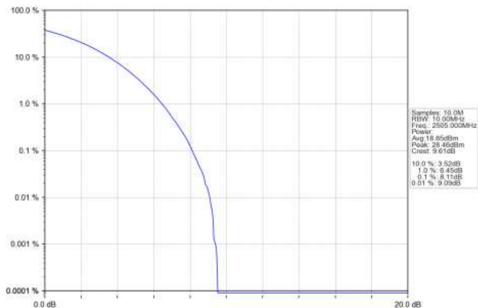
n7_30kHz_SISO_NTNV_10MHz_CP-OFDM_QPSK_2505MHz_Outer_Full_Ant1
