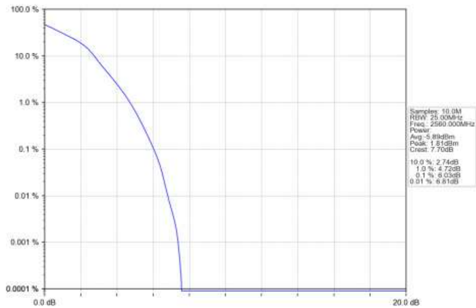
n7_30kHz_SISO_NTNV_20MHz_DFT-s-OFDM_16_QAM_2560MHz_Outer_Full_Ant1
