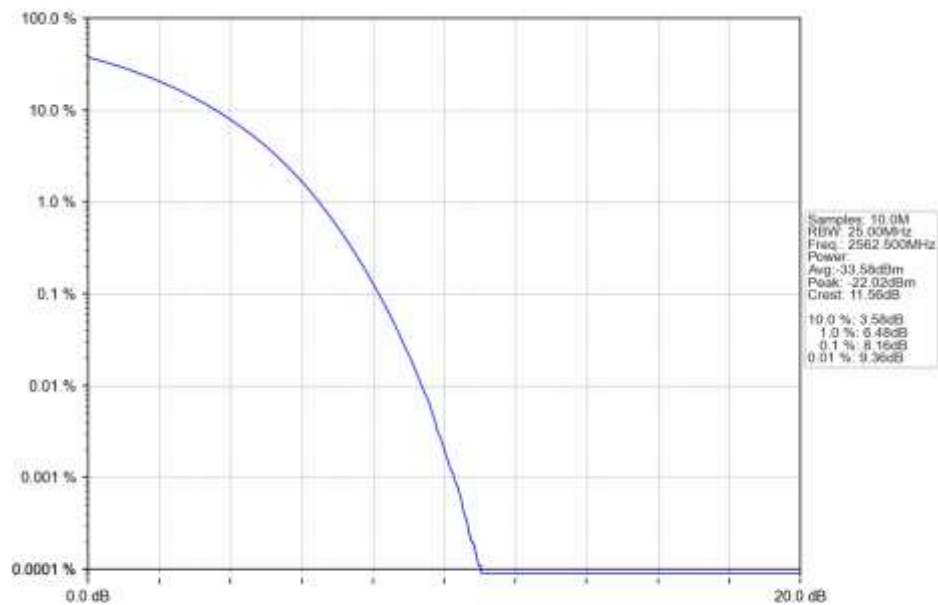
n7_30kHz_SISO_NTNV_15MHz_CP-OFDM_16_QAM_2562.5MHz_Outer_Full_Ant1
