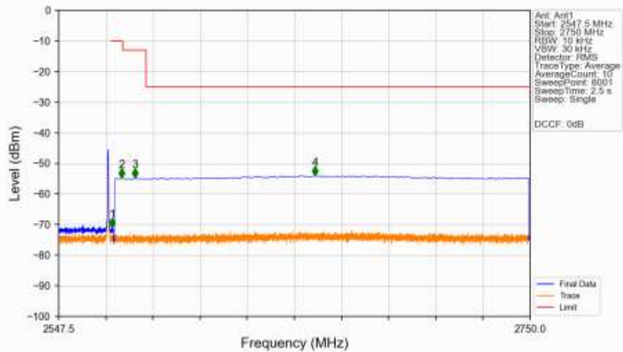
n7_30kHz_SISO_NTNV_15MHz_DFT-s-OFDM_QPSK_2562.5MHz_Inner_1RB_Right_Ant1
