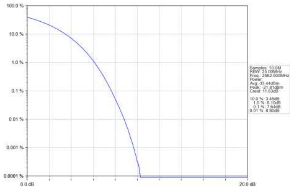
n7_30kHz_SISO_NTNV_15MHz_DFT-s-OFDM_256_QAM_2562.5MHz_Outer_Full_Ant1
