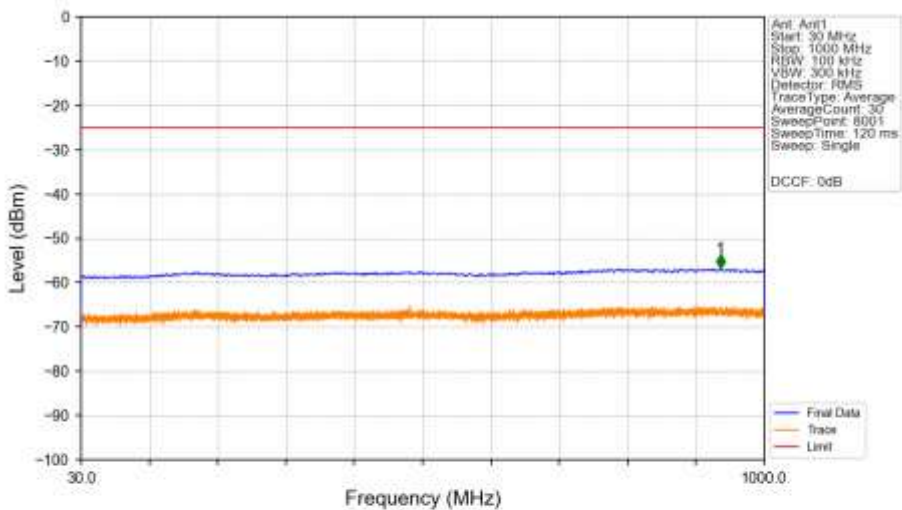
n7_15kHz_SISO_NTNV_15MHz_DFT-s-OFDM QPSK_2507.5MHz_Edge_1RB_Left_Ant1
