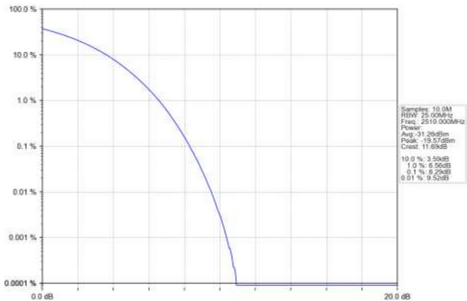
n7_30kHz_SISO_NTNV_20MHz_CP-OFDM_16_QAM_2510MHz_Outer_Full_Ant1
