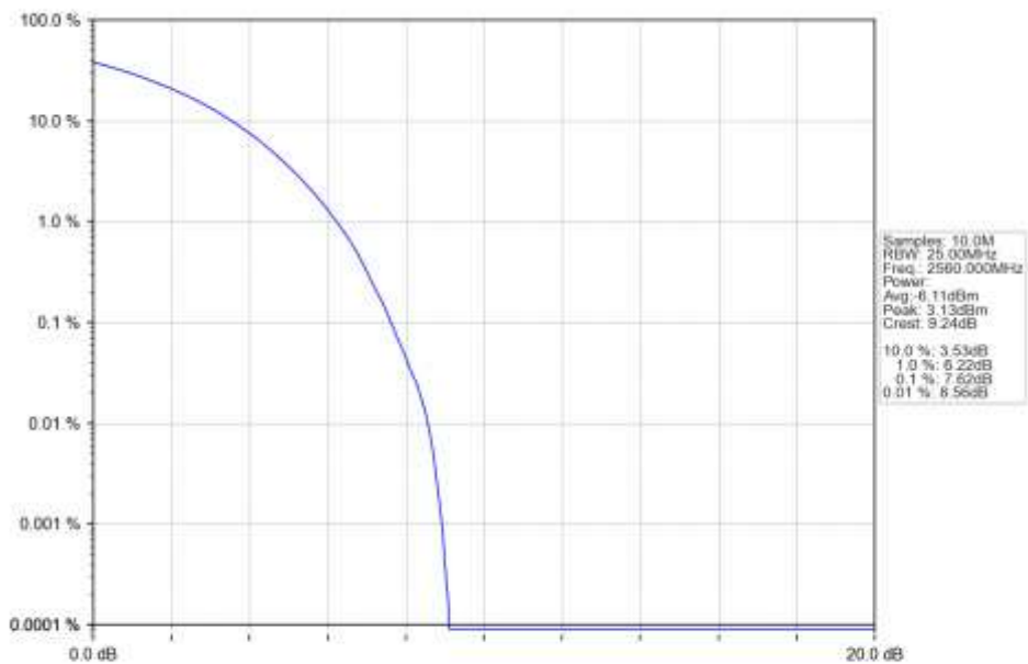
n7_30kHz_SISO_NTNV_20MHz_CP-OFDM_QPSK_2560MHz_Outer_Full_Ant1
