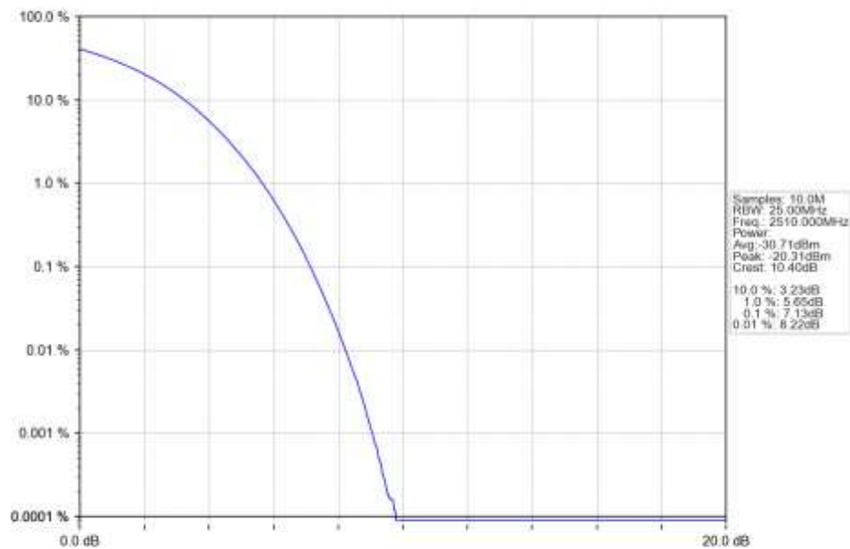
n7_30kHz_SISO_NTNV_20MHz_DFT-s-OFDM_16_QAM_2510MHz_Outer_Full_Ant1
