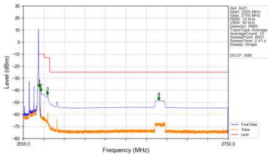
n7_15kHz_SISO_NTNV_10MHz_CP-OFDM_QPSK_2565MHz_Inner_1RB_Right Ant1
