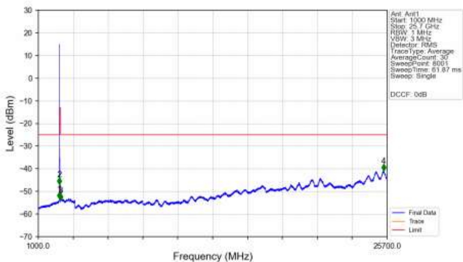
n7_15kHz_SISO_NTNV_15MHz_CP-OFDM_QPSK_2507.5MHz_Edge_1RB_Left_Ant1
