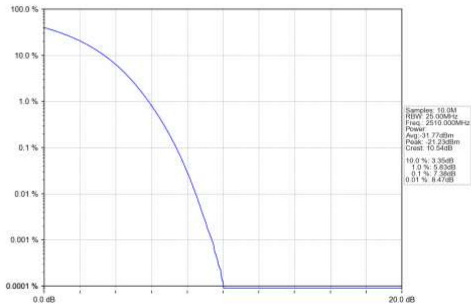
n7_30kHz_SISO_NTNV_20MHz_DFT-s-OFDM_256_QAM_2510MHz_Outer_Full_Ant1
