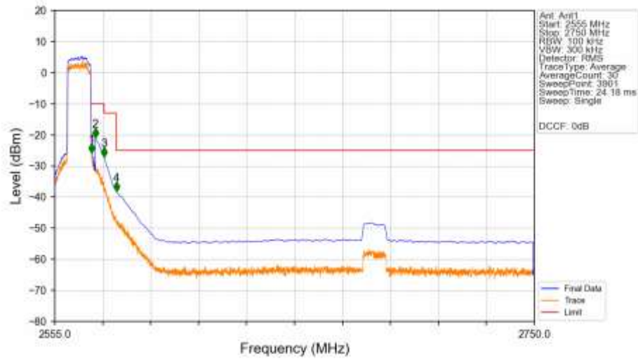
n7_15kHz_SISO_NTNV_10MHz_CP-OFDM_QPSK_2565MHz_Outer_Full_Ant1
