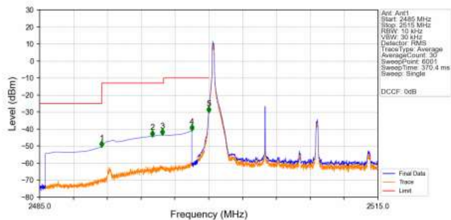
n7_15kHz_SISO_NTNV_10MHz_DFT-s-OFDM_QPSK_2505MHz_Edge_1RB_Left_Ant1
