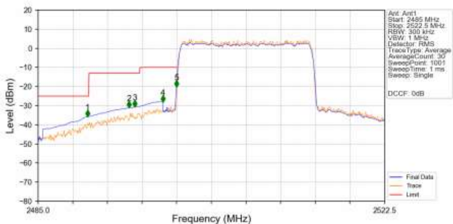
n7_15kHz_SISO_NTNV_15MHz_CP-OFDM_QPSK_2507.5MHz_Outer_Full_Ant1
