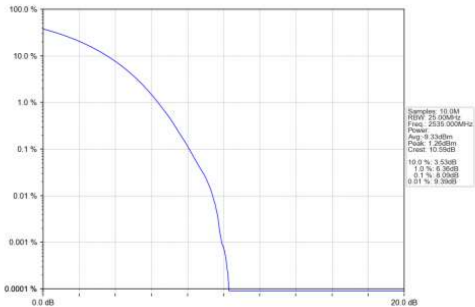
n7_30kHz_SISO_NTNV_20MHz_CP-OFDM_16_QAM_2535MHz_Outer_Full_Ant1
