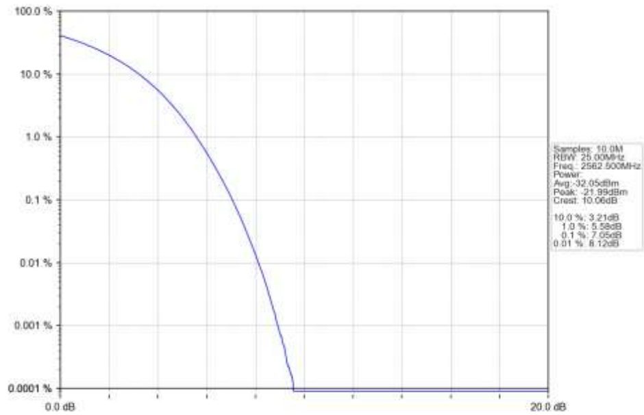
n7_30kHz_SISO_NTNV_15MHz_DFT-s-OFDM_QPSK_2562.5MHz_Outer_Full_Ant1
