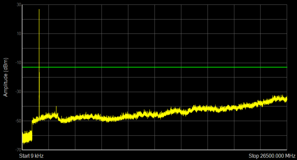
Band4 16QAM BW=15MHz Channel=20025 RB Size=1 Position=#0
