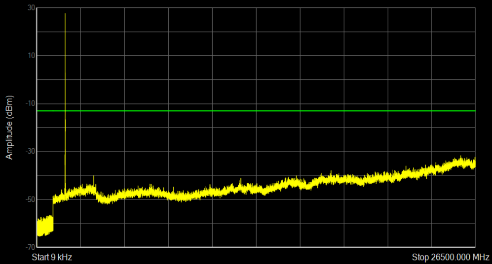
Band4 16QAM BW=5MHz Channel=20175 RB Size=1 Position=#0
