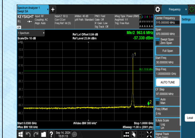
Band5-4233-1-30~1000MHz-PASS
