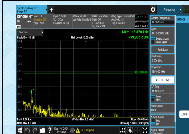
Band5-4233-0.009~0.15MHz-PASS
