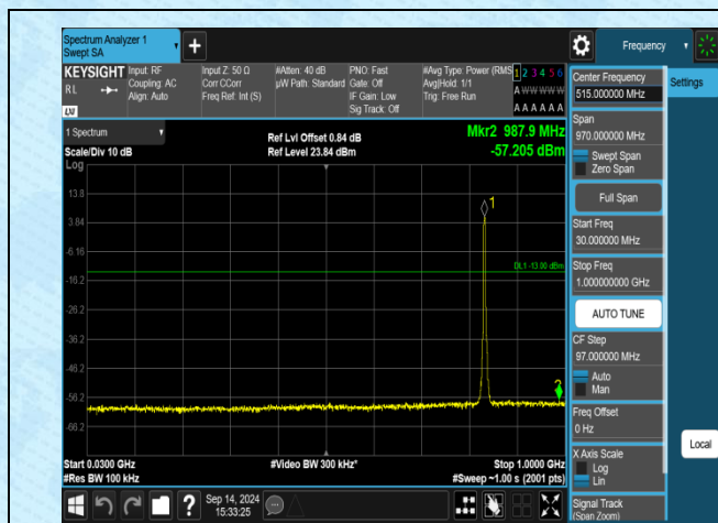
Band5-4182-30~1000MHz-PASS
