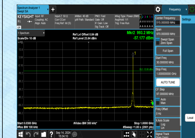
Band5-4233-30~1000MHz-PASS
