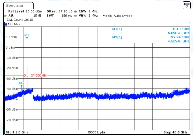
11A-Ant1-5580-1000~40000-PASS
