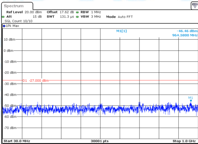
11AC40SISO-Ant1-5510-30~1000-PASS
