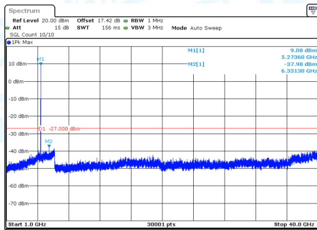
11A-Ant1-5260-1000~40000-PASS
