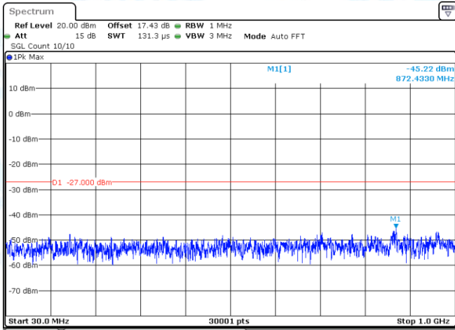
11AC40SISO-Ant1-5310-30~1000-PASS
