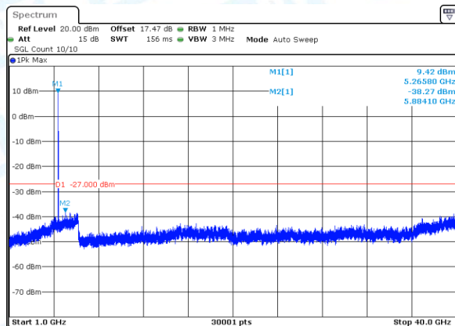
11A-Ant1-5260-1000~40000-PASS
