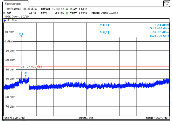
11AC40SISO-Ant1-5190-1000~40000-PASS
