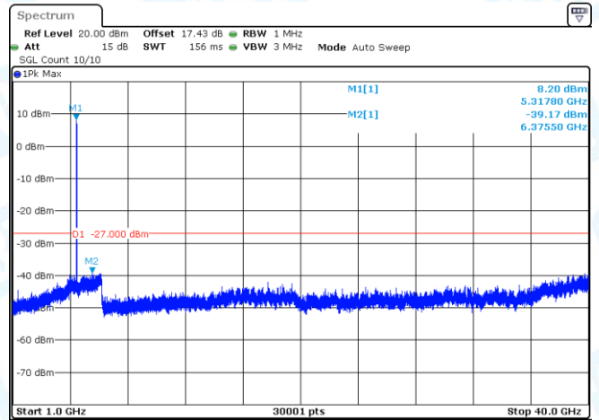
11AC20SISO-Ant1-5280-1000~40000-PASS
