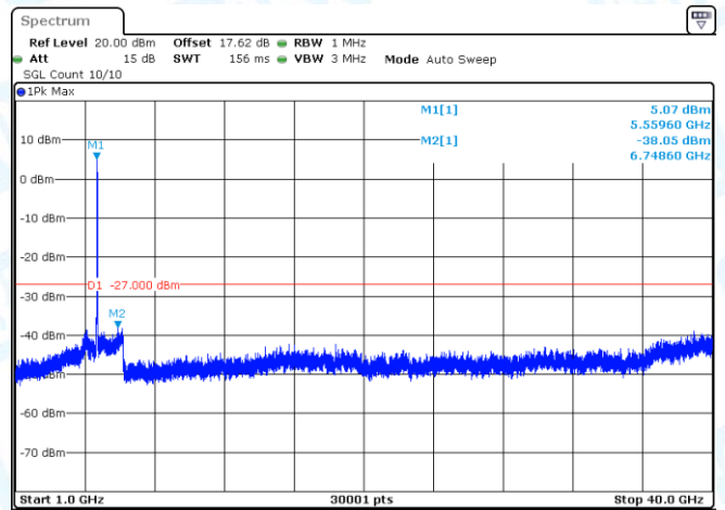
11AC40SISO-Ant1-5510-1000~40000-PASS
