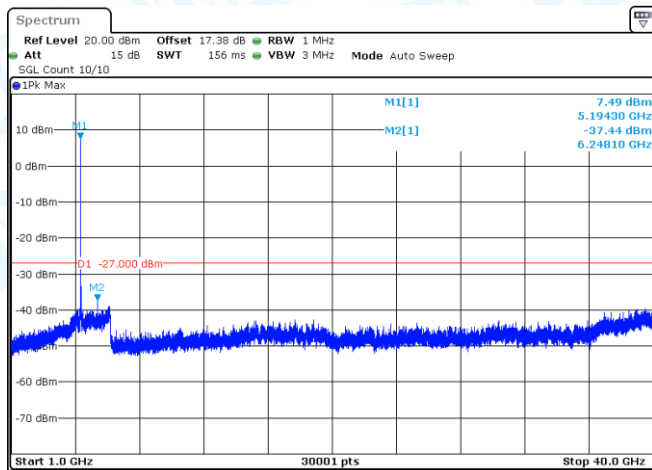
11AX20SISO-Ant1-5180-1000~40000-PASS
