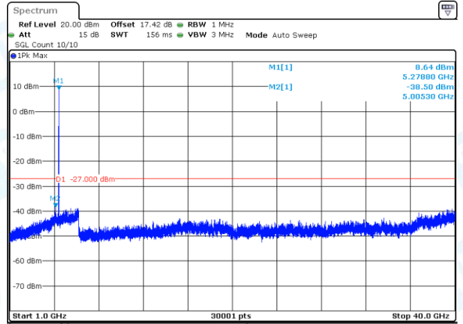
11AC20SISO-Ant1-5260-1000~40000-PASS
