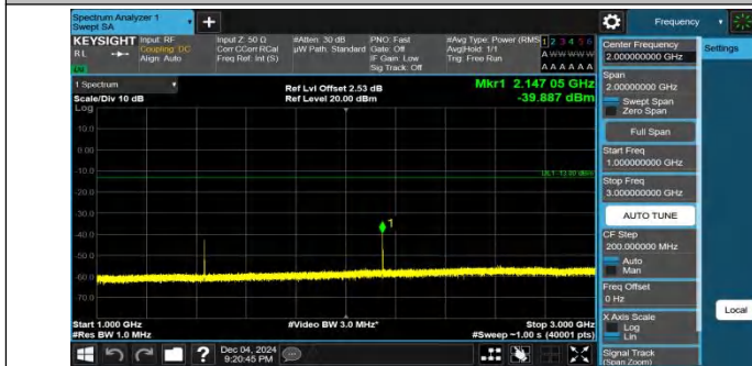
Band17-5MHz-QPSK-23825-1RB#24-1000~3000-PASS
