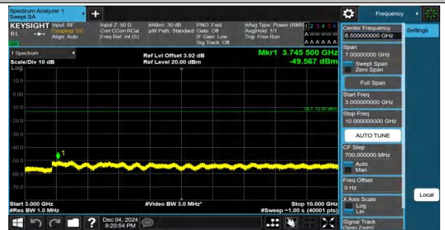
Band17-5MHz-QPSK-23825-1RB#24-3000~10000-PASS
