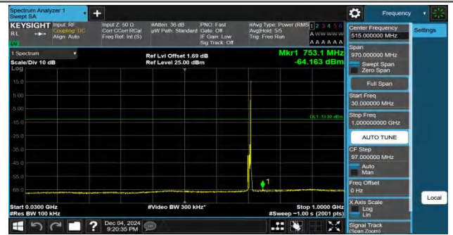
Band17-5MHz-QPSK-23825-1RB#24-30~1000-PASS
