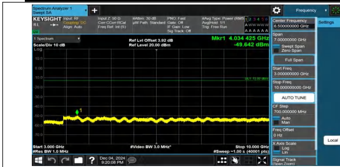
Band17-5MHz-QPSK-23825-1RB#0-3000~10000-PASS
