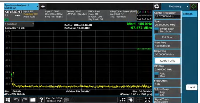
Band17-10MHz-QPSK-23780-1RB#0-0.15~30-PASS
