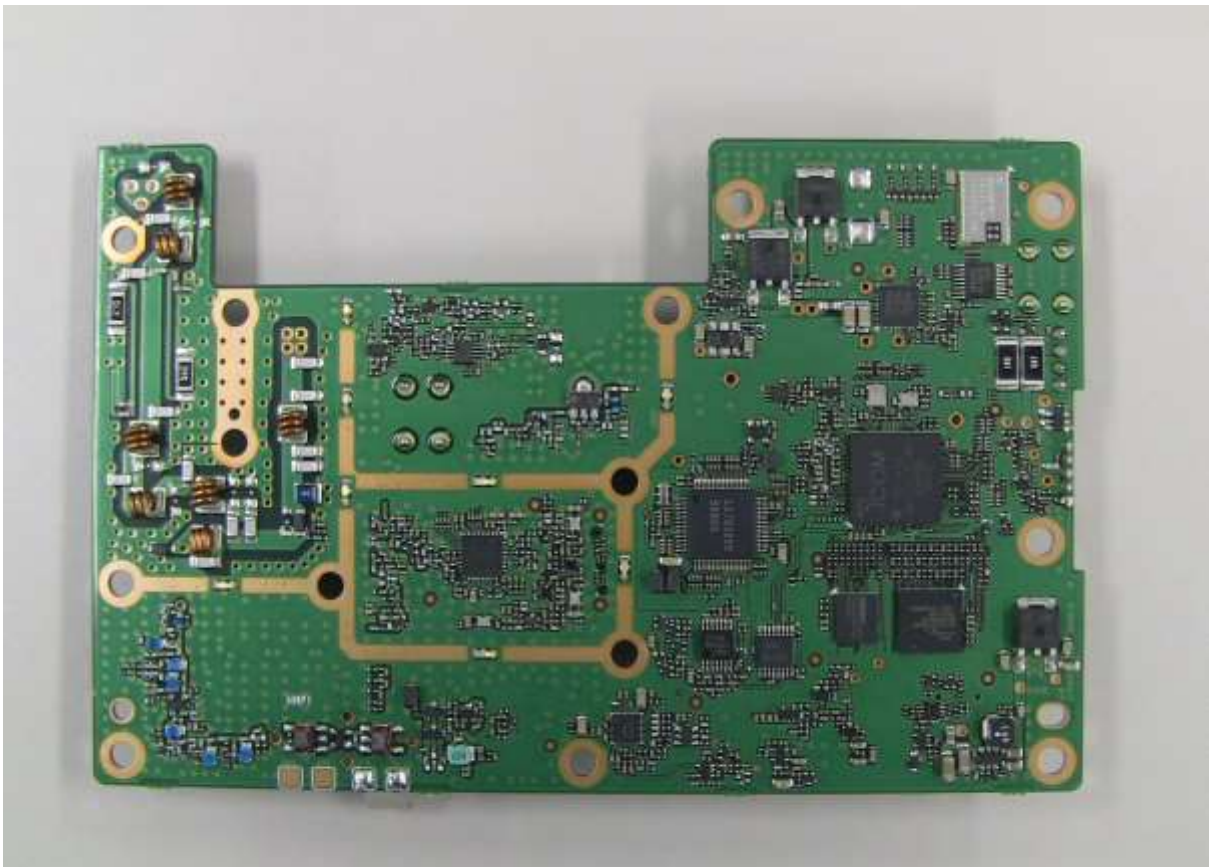
IC-F7520 MAIN-C UNIT B SIDE
