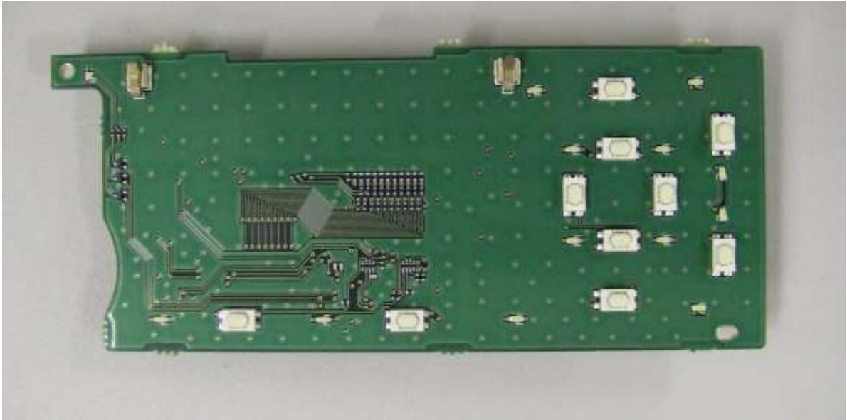
IC-F7520 FRONT-A UNIT A SIDE
