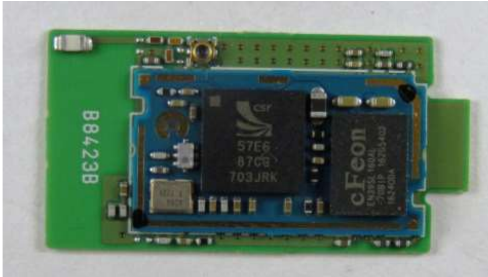
IC-F7520 Board(UT-136) on RELAY-C UNIT A SIDE
