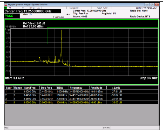
Band42_20MHz_16QAM_42190_1RB#99
