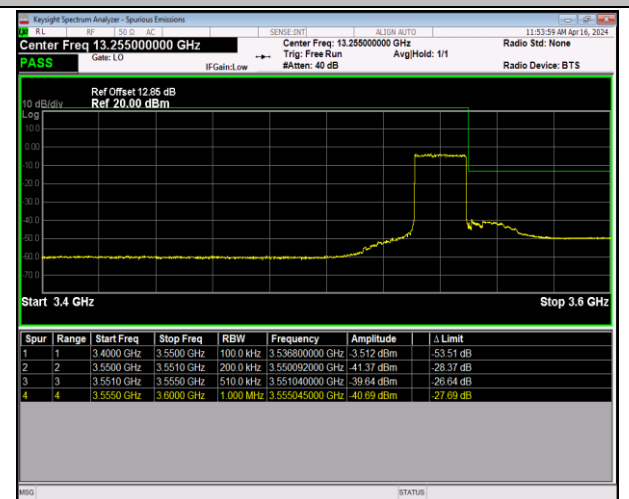
Band42_20MHz_QPSK_42990_100RB#0
