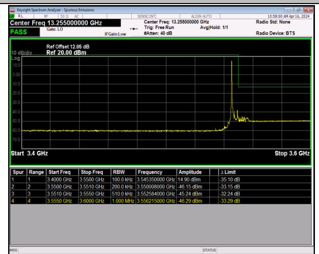
Band42_5MHz_64QAM_42115_25RB#24
