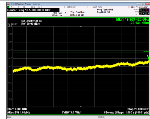
Band2_1.4MHz_64QAM_18900_1RB#0_1000~20000_1000~20000
