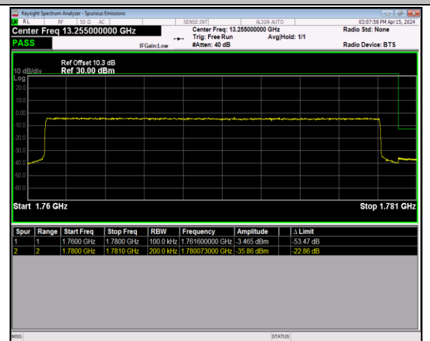
Band66_20MHz_16QAM_132572_100RB#0
