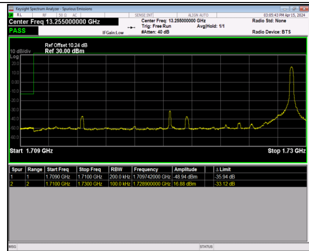
Band66_20MHz_64QAM_132072_1RB#99
