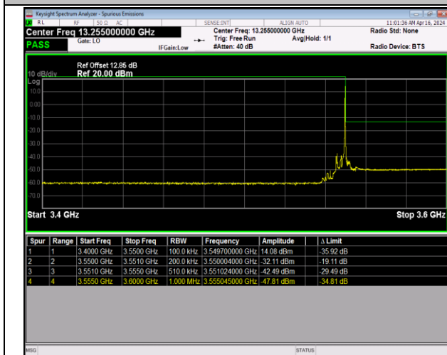
Band42_5MHz_64QAM_43065_1RB#24
