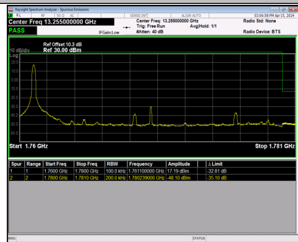
Band66_20MHz_64QAM_132572_1RB#0
