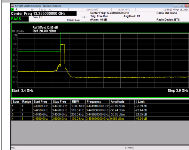
Band42_5MHz_64QAM_42115_25RB#0
