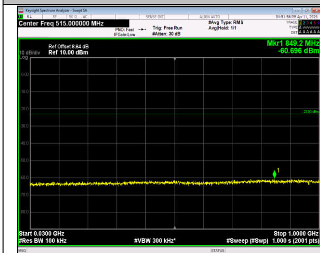
Band2_1.4MHz_64QAM_19193_1RB#0_30~1000_30~1000
