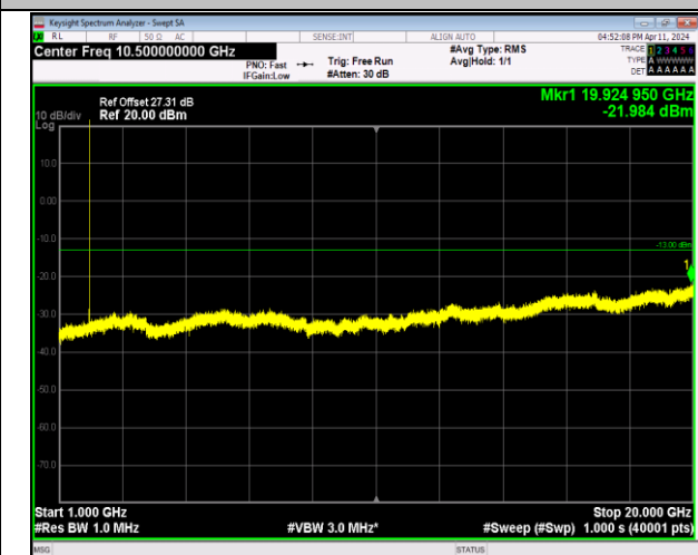
Band2_1.4MHz_64QAM_19193_1RB#0_1000~20000_1000~20000
