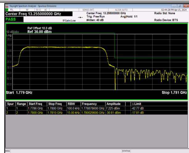
Band66_1.4MHz_64QAM_132665_6RB#0
