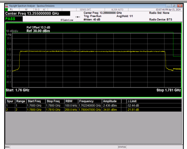
Band66_20MHz_QPSK_132572_100RB#0
