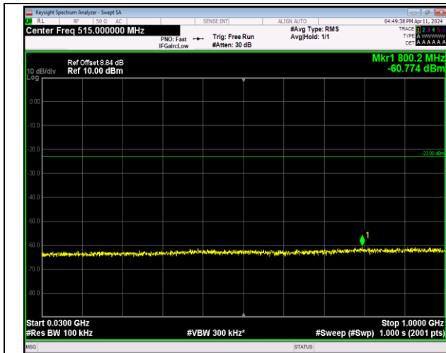
Band2_1.4MHz_64QAM_18607_1RB#0_30~1000_30~1000
