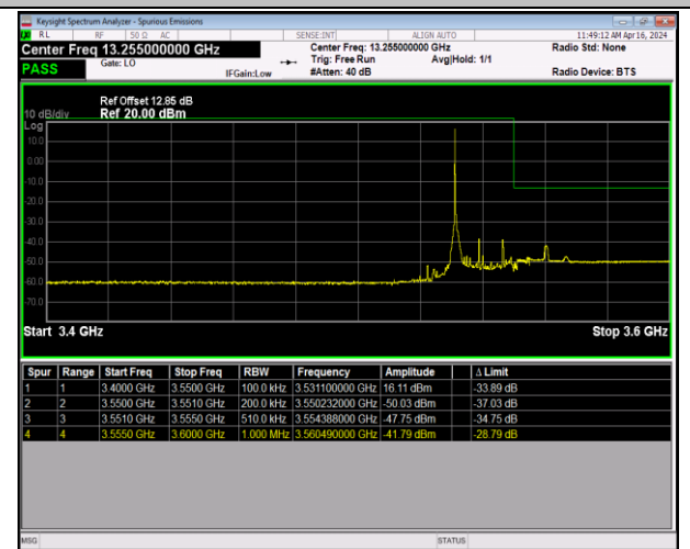
Band42_20MHz_64QAM_42990_1RB#0
