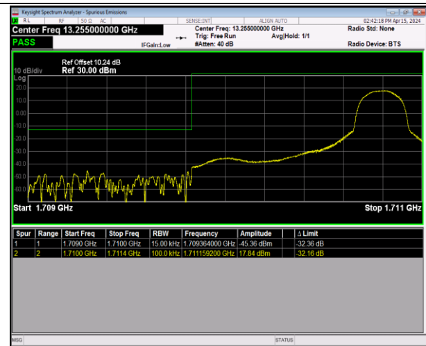
Band66_1.4MHz_16QAM_131979_1RB#5
