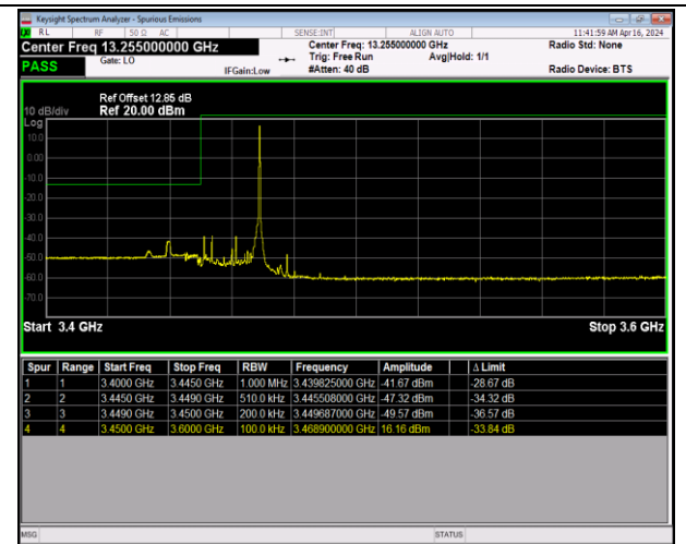
Band42_20MHz_64QAM_42190_1RB#99
