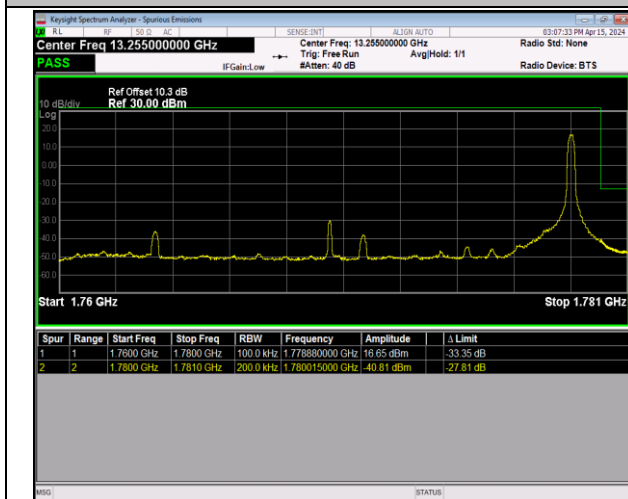
Band66_20MHz_64QAM_132572_1RB#99
