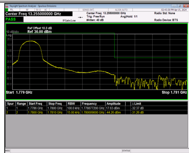
Band66_1.4MHz_64QAM_132665_1RB#0
