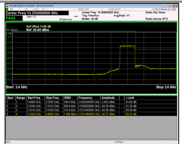
Band42_20MHz_64QAM_42990_100RB#0
