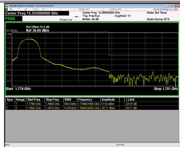
Band66_1.4MHz_16QAM_132665_1RB#0
