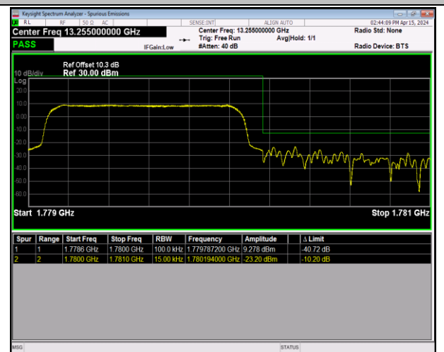
Band66_1.4MHz_QPSK_132665_6RB#0
