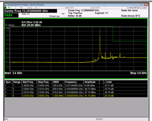
Band42_20MHz_16QAM_42990_1RB#0
