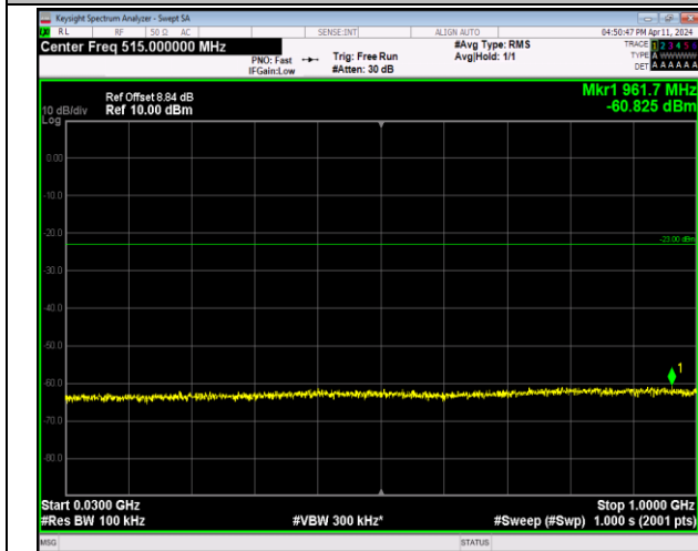
Band2_1.4MHz_64QAM_18900_1RB#0_30~1000_30~1000
