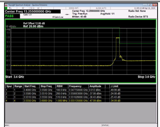
Band42_5MHz_64QAM_43065_25RB#0
