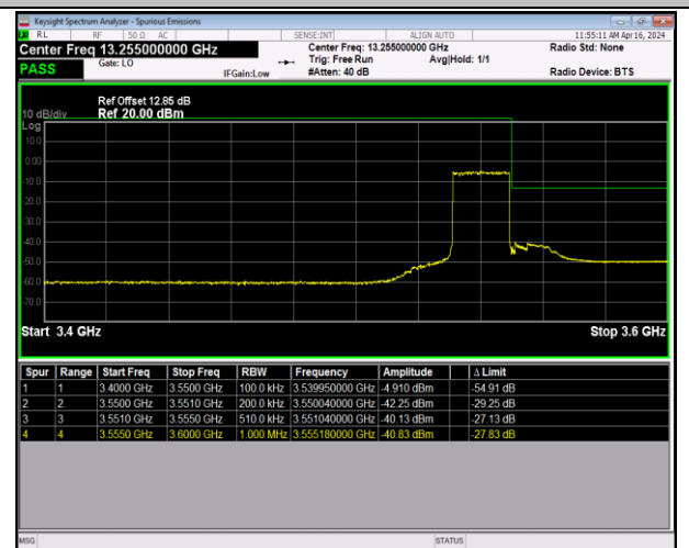
Band42_20MHz_16QAM_42990_100RB#0
