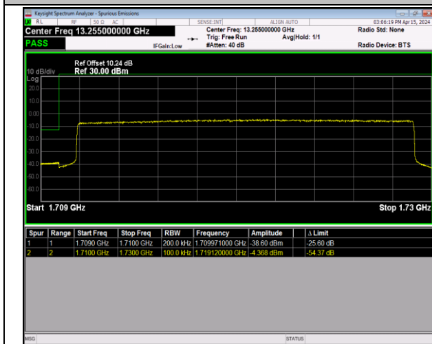
Band66_20MHz_64QAM_132072_100RB#0
