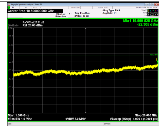
Band2_1.4MHz_64QAM_18607_1RB#0_1000~20000_1000~20000
