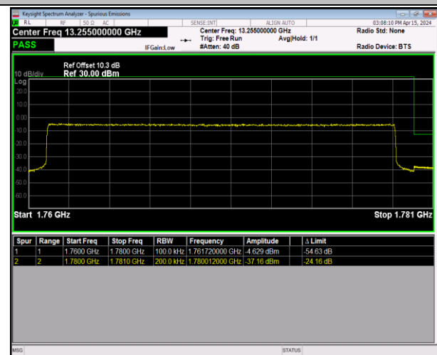
Band66_20MHz_64QAM_132572_100RB#0
