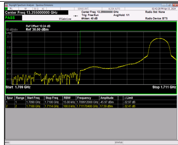
Band66_1.4MHz_64QAM_131979_1RB#5
