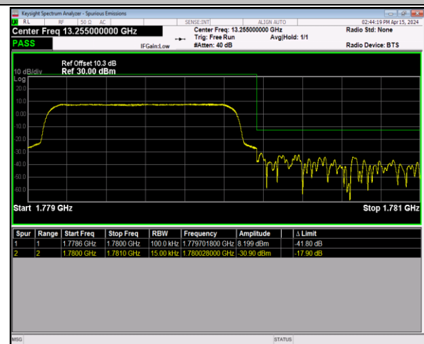
Band66_1.4MHz_16QAM_132665_6RB#0
