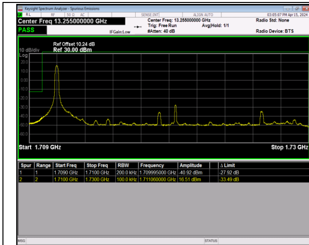
Band66_20MHz_64QAM_132072_1RB#0
