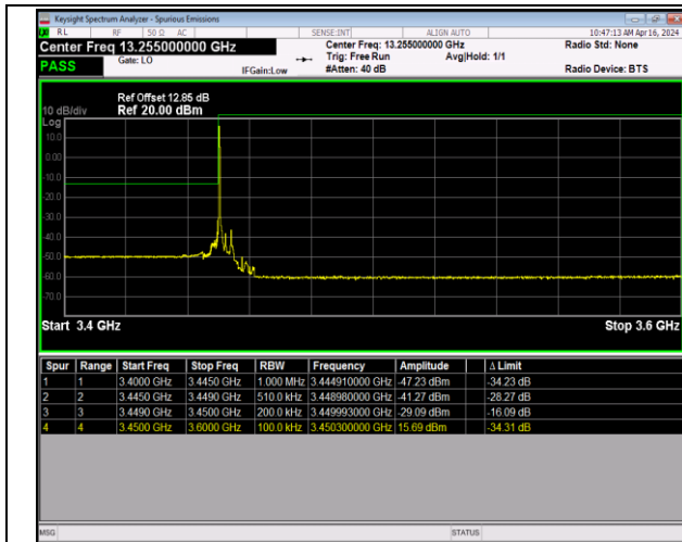
Band42_5MHz_64QAM_42115_1RB#0
