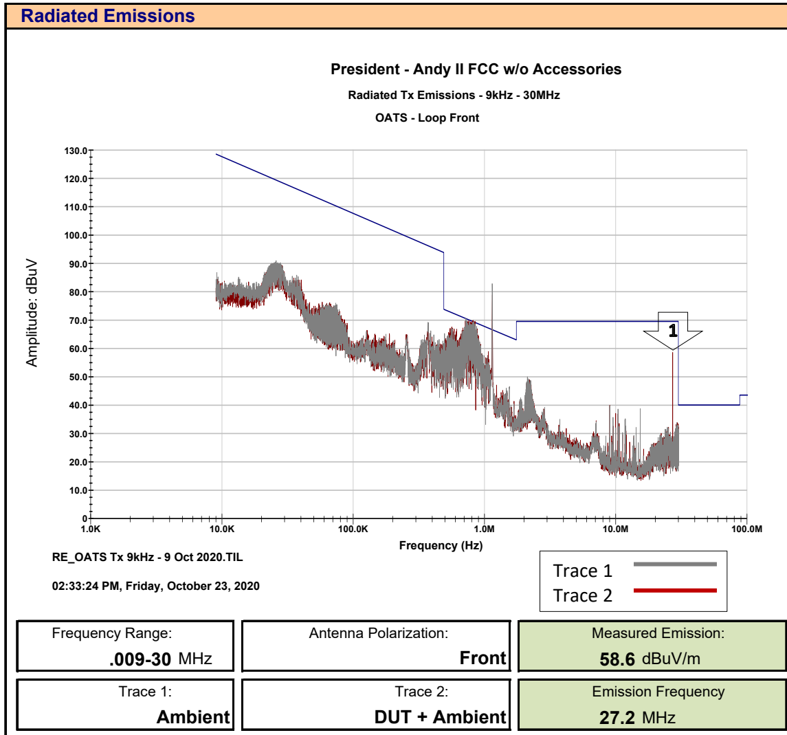
Plot 11.1 – Radiated Spurious Emissions OATS, 9kHz - 30MHz, Front without Accessories
