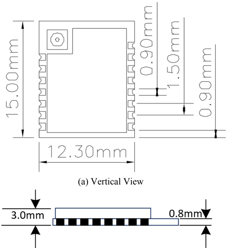
(a) Vertical View (b) Side View Fig. 3.2 Size for ESP-M1
