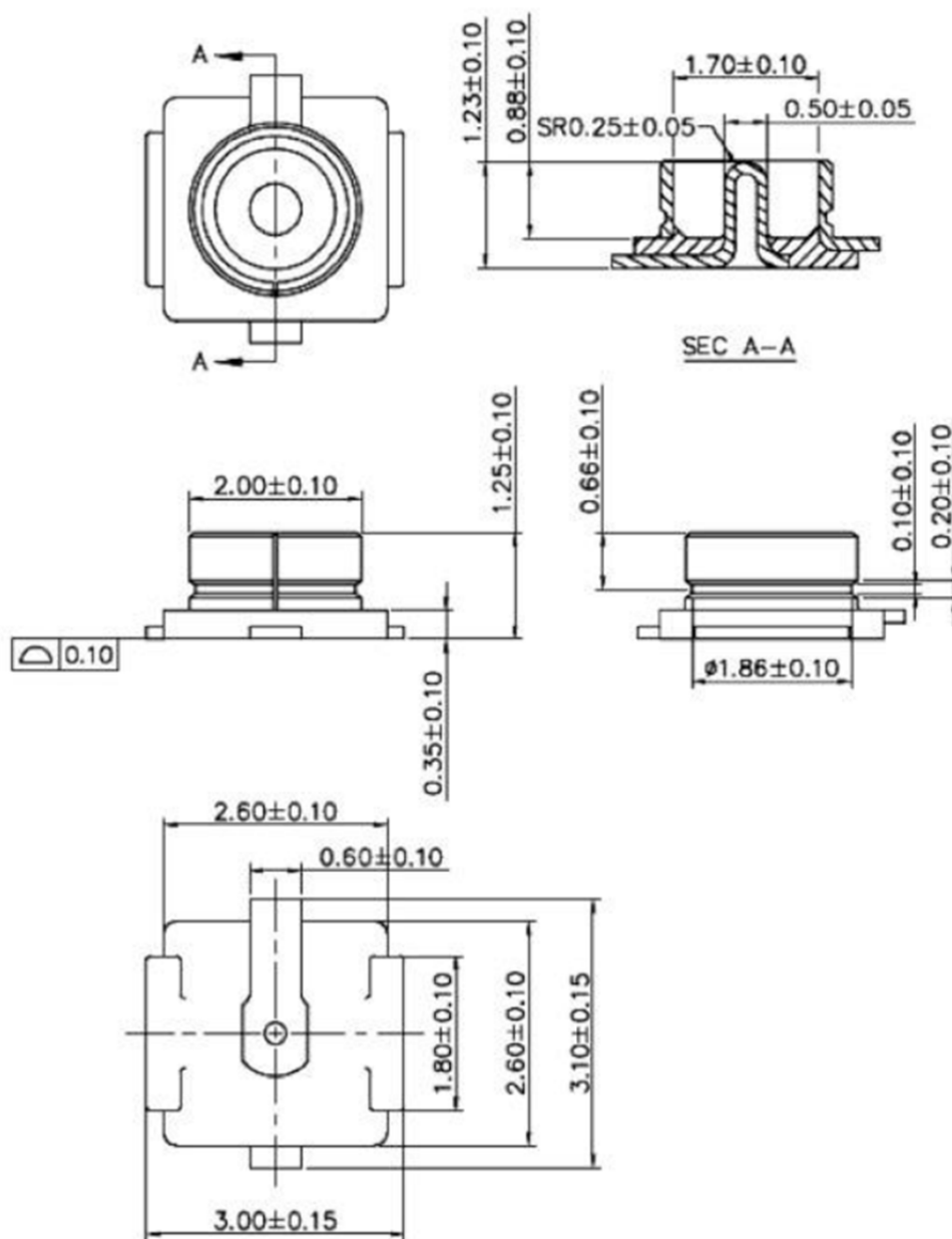
Fig. 9. 1 Connector for the external antenna
