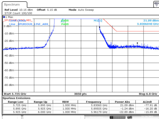
BE-NR-HIGH-PEAK, MIMO-A, 802.11ax80-MCS0, Ch171
