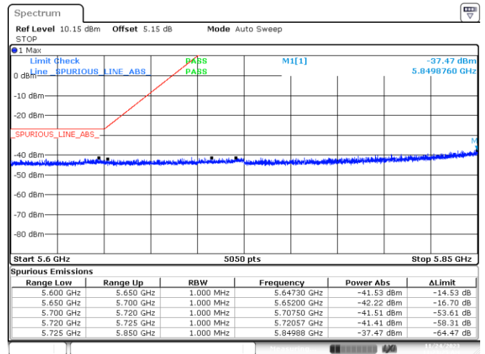
BE-NR-LOW, SISO-B, 802.11ax20-MCS0, Ch177
