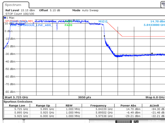
BE-NR-HIGH-PEAK, SISO-B, 802.11ax160-MCS0, Ch163
