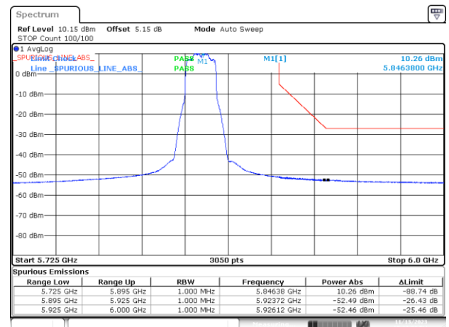
BE-NR-HIGH, MIMO-B, 802.11ax20-MCS0, Ch169
