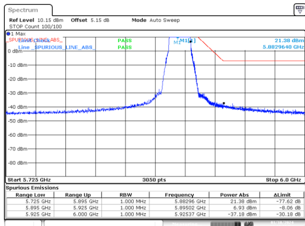
BE-NR-HIGH-PEAK, MIMO-B, 802.11ax20-MCS0, Ch177
