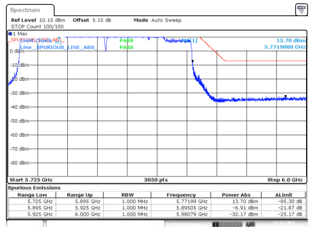
BE-NR-HIGH-PEAK, MIMO-A, 802.11ax160-MCS0, Ch163
