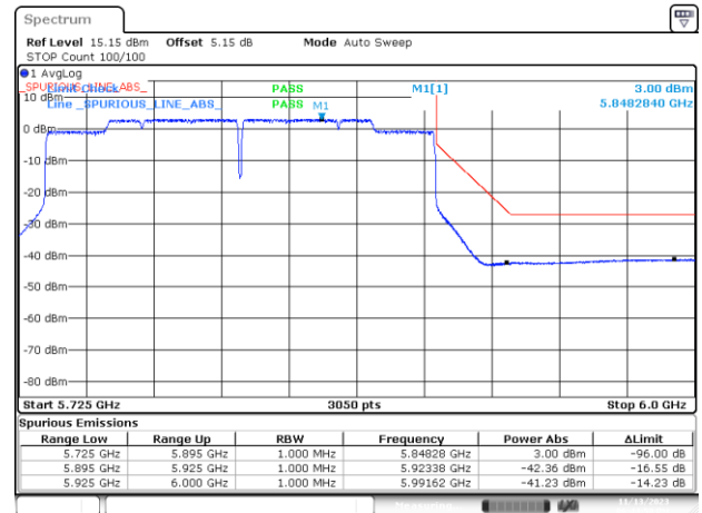
BE-NR-HIGH, SISO-B, 802.11ax160-MCS0, Ch163
