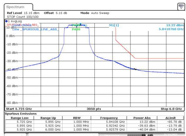
BE-NR-HIGH, SISO-B, 802.11ax40-MCS0, Ch167
