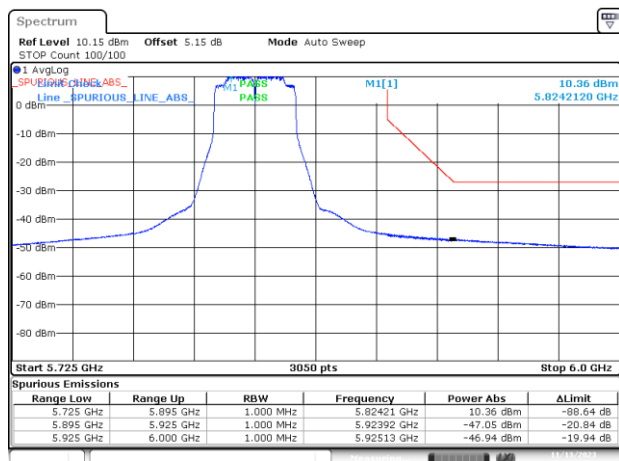
BE-NR-HIGH, MIMO-B, 802.11n40-HT0, Ch167
