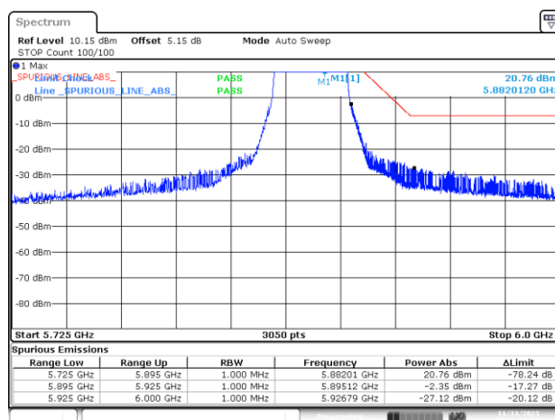
BE-NR-HIGH-PEAK, MIMO-B, 802.11n40-HT0, Ch175
