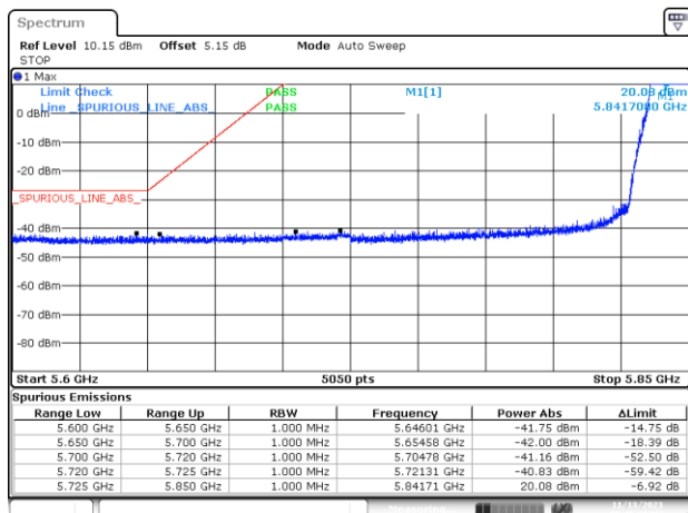
BE-NR-LOW, MIMO-B, 802.11n20-HT0, Ch169
