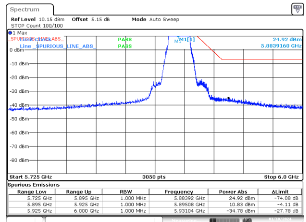
BE-NR-HIGH-PEAK, SISO-B, 802.11ax20-MCS0, Ch177
