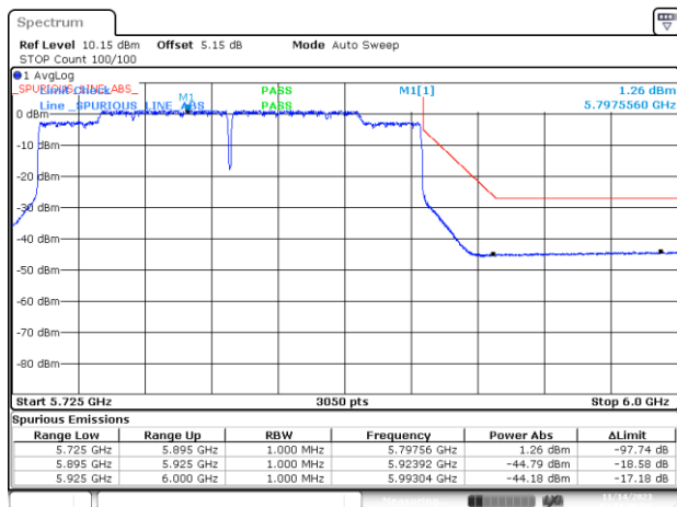
BE-NR-HIGH, MIMO-A, 802.11ax160-MCS0, Ch163
