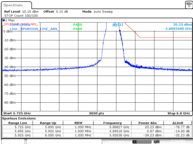
BE-NR-HIGH-PEAK, MIMO-B, 802.11n20-HT0, Ch177
