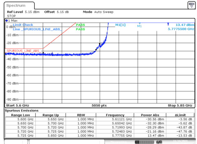
BE-NR-LOW, MIMO-A, 802.11ax160-MCS0, Ch163
