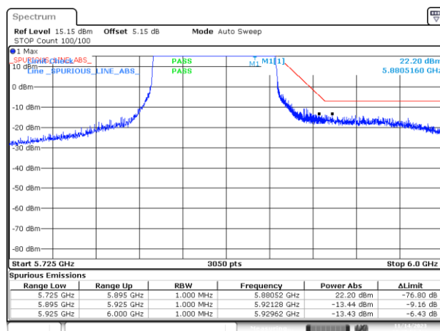
BE-NR-HIGH-PEAK, SISO-B, 802.11ax80-MCS0, Ch171
