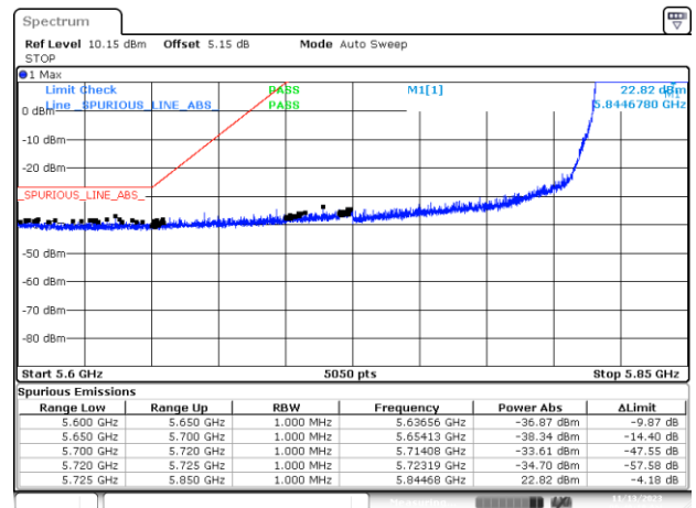
BE-NR-LOW, MIMO-A, 802.11ax40-MCS0, Ch167
