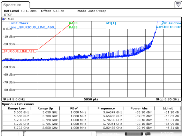
BE-NR-LOW, MIMO-B, 802.11n40-HT0, Ch167
