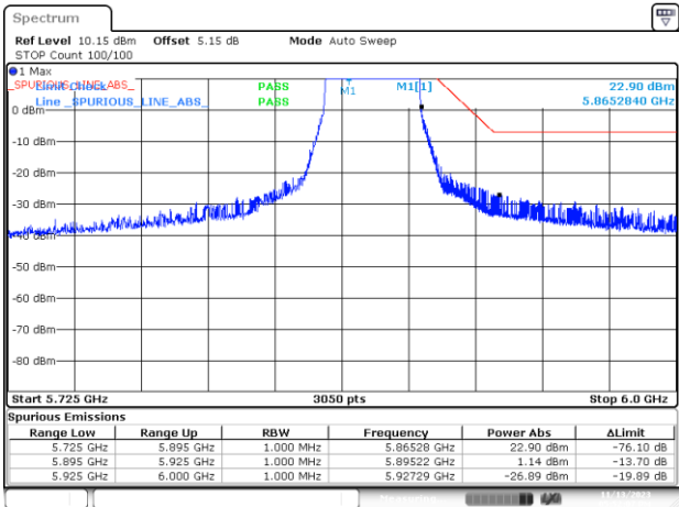
BE-NR-HIGH-PEAK, MIMO-B, 802.11ax40-MCS0, Ch175
