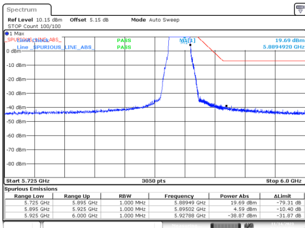
BE-NR-HIGH-PEAK, MIMO-A, 802.11ax20-MCS0, Ch177
