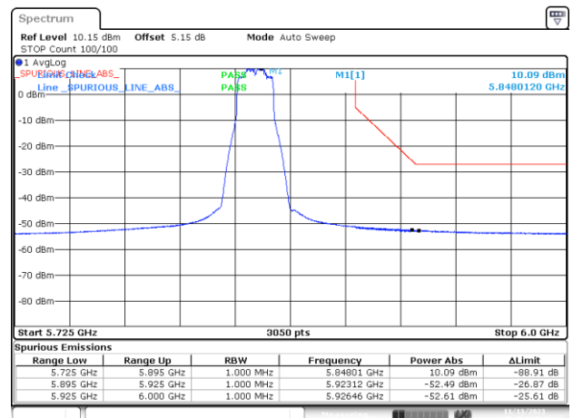
BE-NR-HIGH, MIMO-B, 802.11n20-HT0, Ch169
