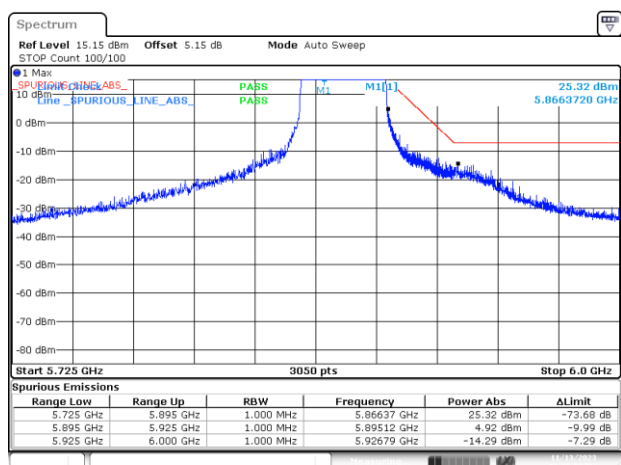
BE-NR-HIGH-PEAK, SISO-B, 802.11ax40-MCS0, Ch175
