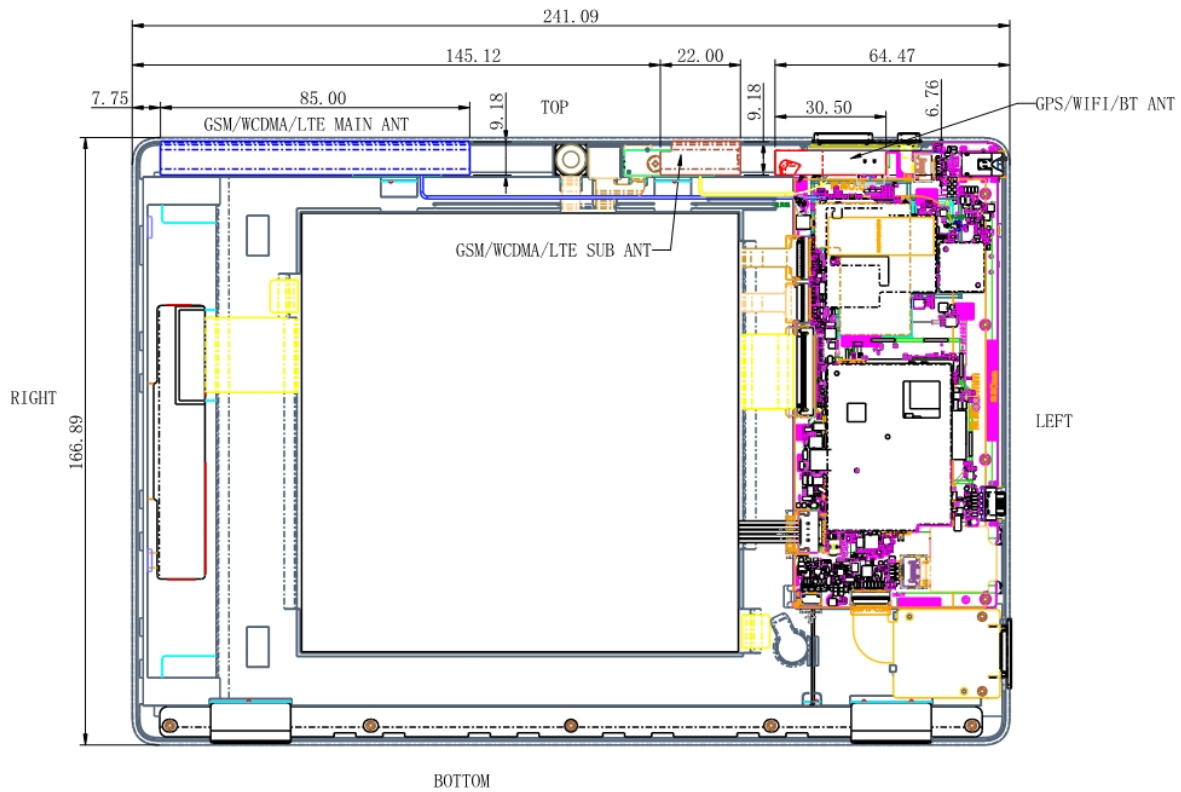
Fig.11.1 EUT Antenna Locations
