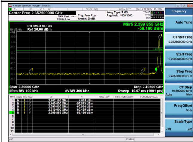
DH5-Ant1-Hop_2402-PASS
