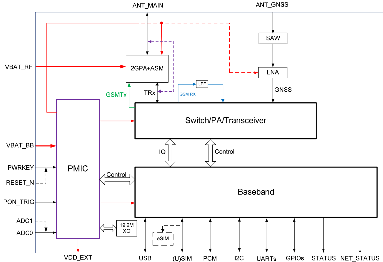
Figure 1: Functional Diagram
