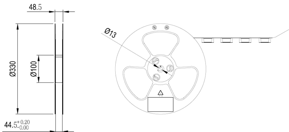
Figure 41: Reel Dimensions
