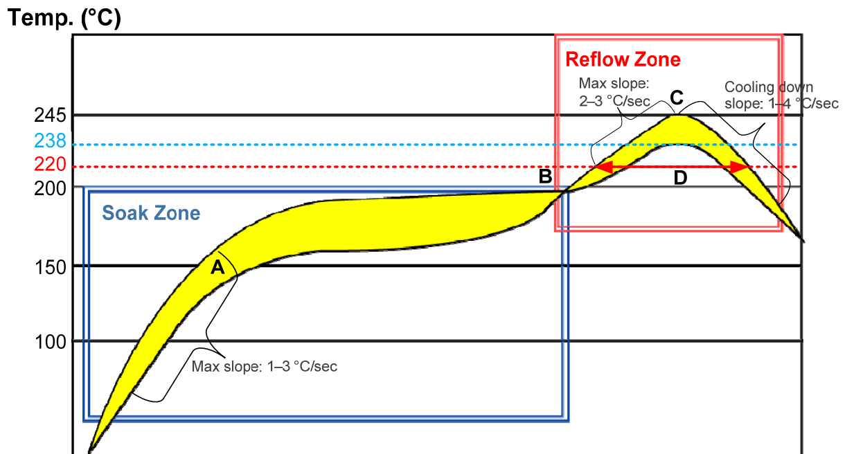
Figure 39: Recommended Reflow Soldering Thermal Profile
