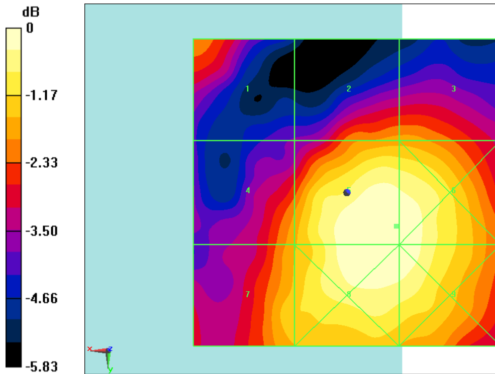
Fig B.2 HAC RF E-Field GSM 1900 Low
