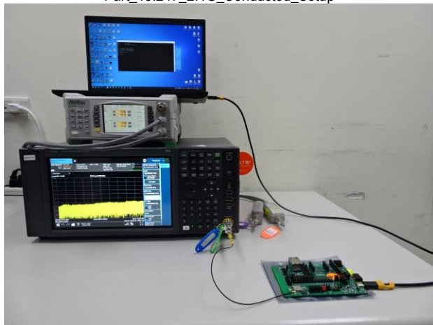
Part_15.247_LE_Port1_Conducted_Setup
