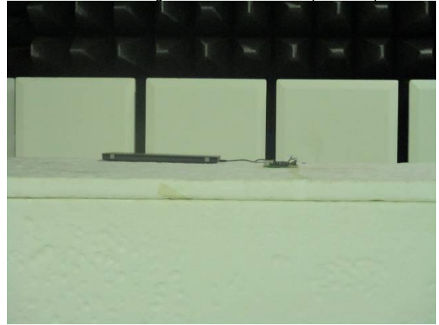
Part_15.247_ZigBee_Port1_Radiated_Dipole_Setup
