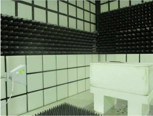
Part_15.247_LE_Port2_Radiated_Setup
