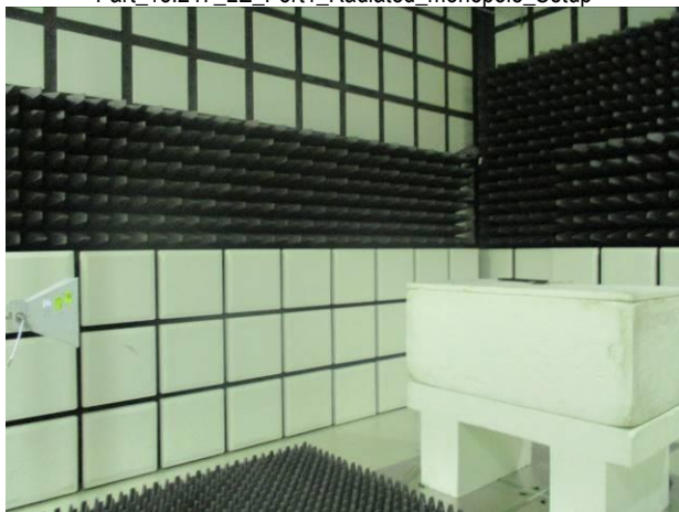
Part_15.247_LE_Port1_Radiated_monopole_Setup
