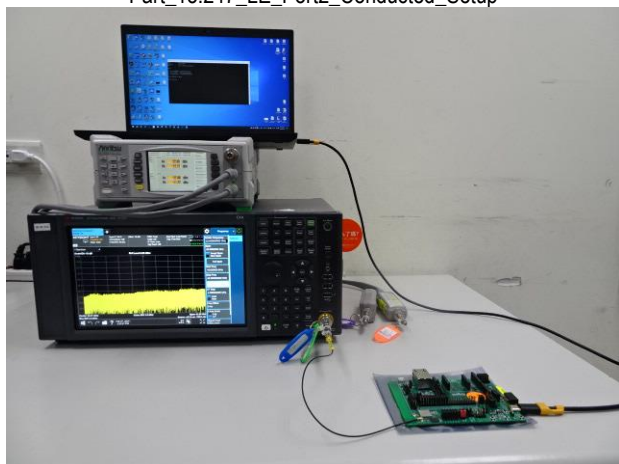
Part_15.247_LE_Port2_Conducted_Setup
