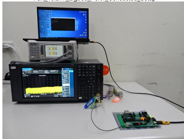
Part_15.247_ZigBee_Port2_Conducted_Setup
