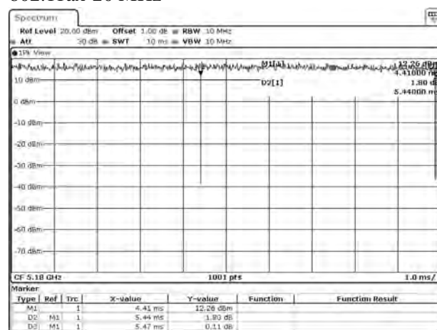
802.11ax-20 MHz
