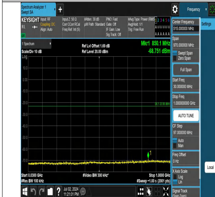
Band66-15MHz-QPSK-132047-1RB#0-30~1000-PASS
