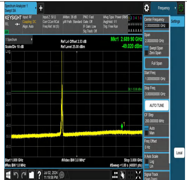
Band66-10MHz-QPSK-132622-1RB#0-1000~3000-PASS
