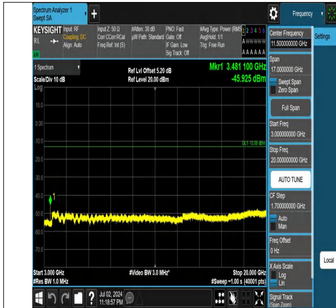
Band66-10MHz-QPSK-132322-1RB#0-3000~20000-PASS
