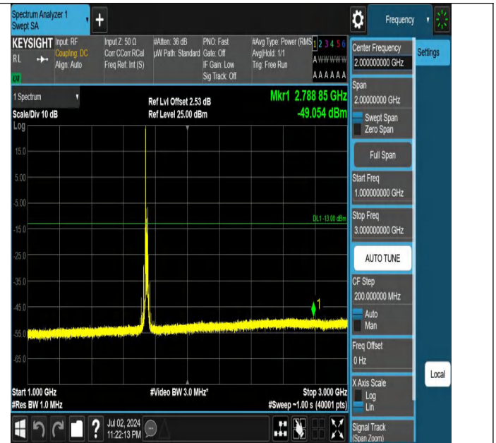
Band66-15MHz-QPSK-132322-1RB#0-1000~3000-PASS
