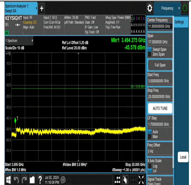
Band66-5MHz-QPSK-132322-1RB#24-3000~20000-PASS
