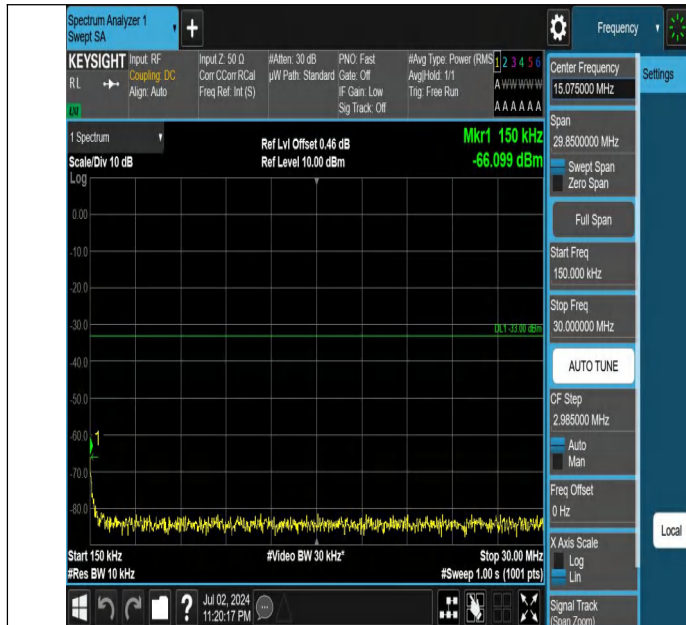
Band66-10MHz-QPSK-132622-1RB#49-0.15~30-PASS
