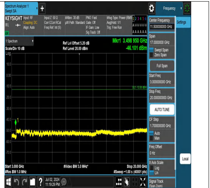
Band66-10MHz-QPSK-132322-1RB#49-3000~20000-PASS
