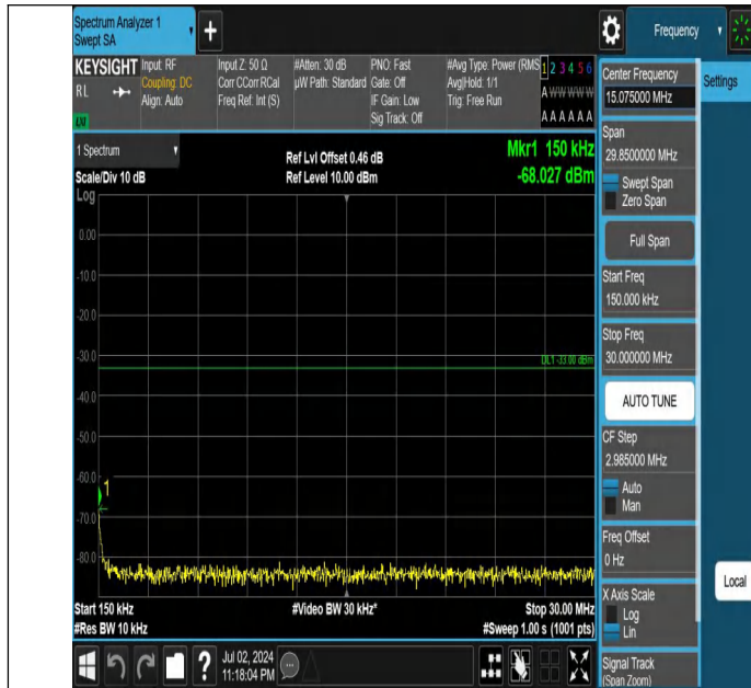
Band66-10MHz-QPSK-132022-1RB#49-0.15~30-PASS
