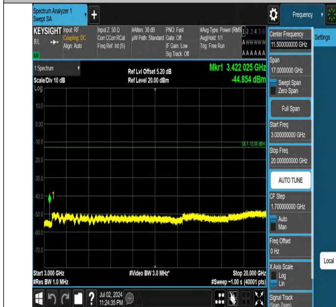
Band66-20MHz-QPSK-132072-1RB#0-3000~20000-PASS
