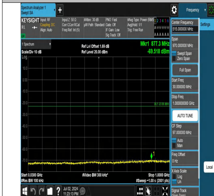
Band66-15MHz-QPSK-132597-1RB#0-30~1000-PASS
