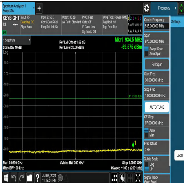
Band66-10MHz-QPSK-132622-1RB#0-30~1000-PASS
