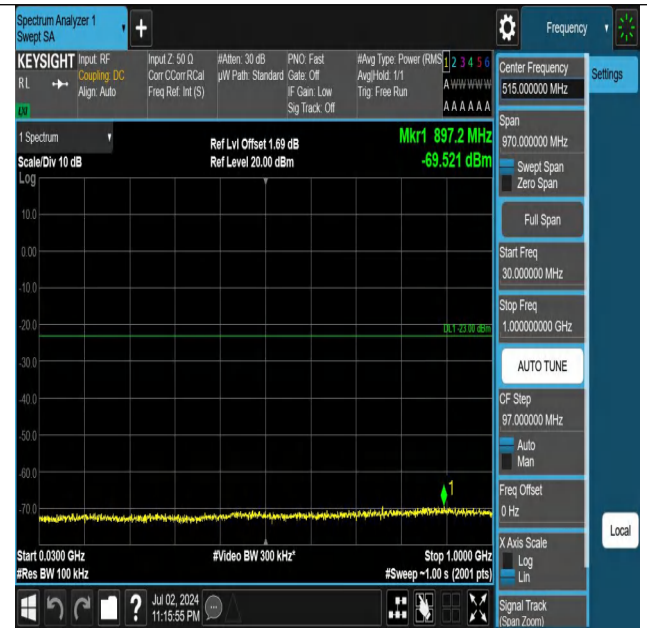
Band66-5MHz-QPSK-132322-1RB#24-30~1000-PASS
