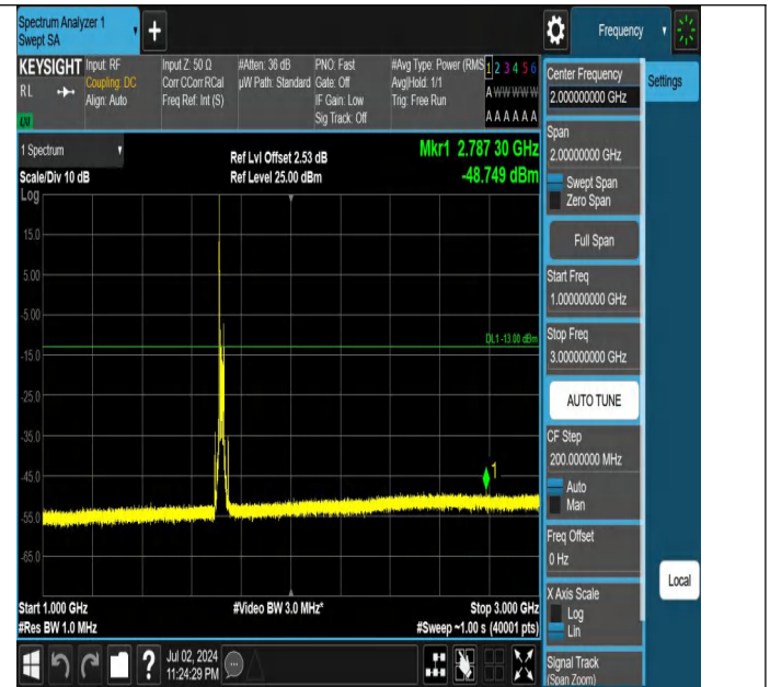
Band66-20MHz-QPSK-132072-1RB#0-1000~3000-PASS
