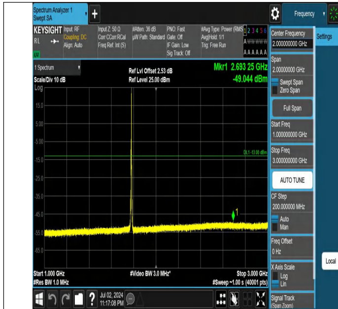
Band66-5MHz-QPSK-132647-1RB#24-1000~3000-PASS
