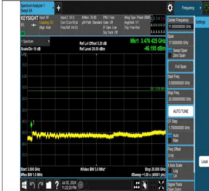
Band66-15MHz-QPSK-132322-1RB#0-3000~20000-PASS
