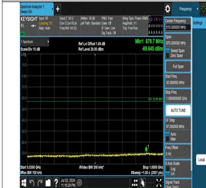
Band66-5MHz-QPSK-132647-1RB#0-30~1000-PASS
