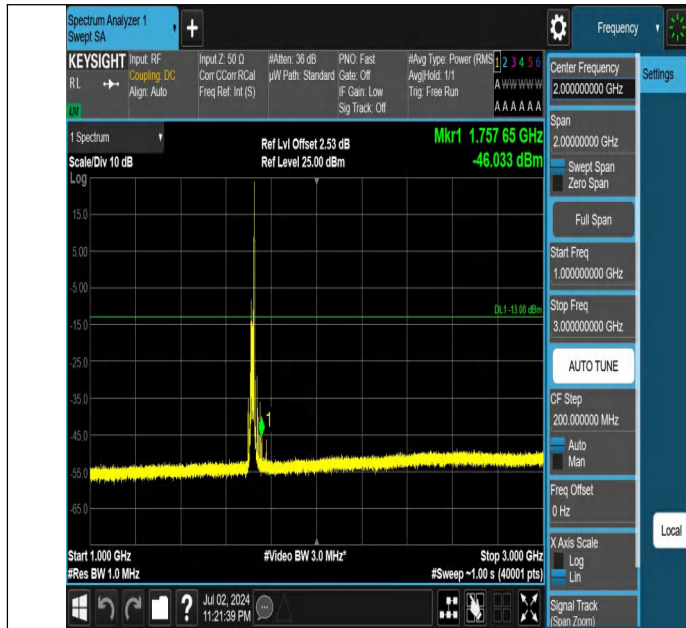
Band66-15MHz-QPSK-132047-1RB#74-1000~3000-PASS
