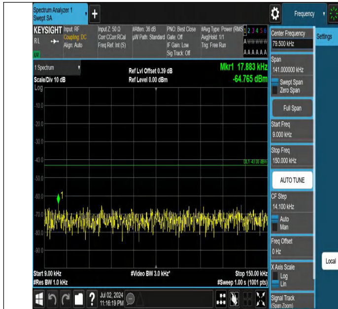
Band66-5MHz-QPSK-132647-1RB#0-0.009~0.15-PASS
