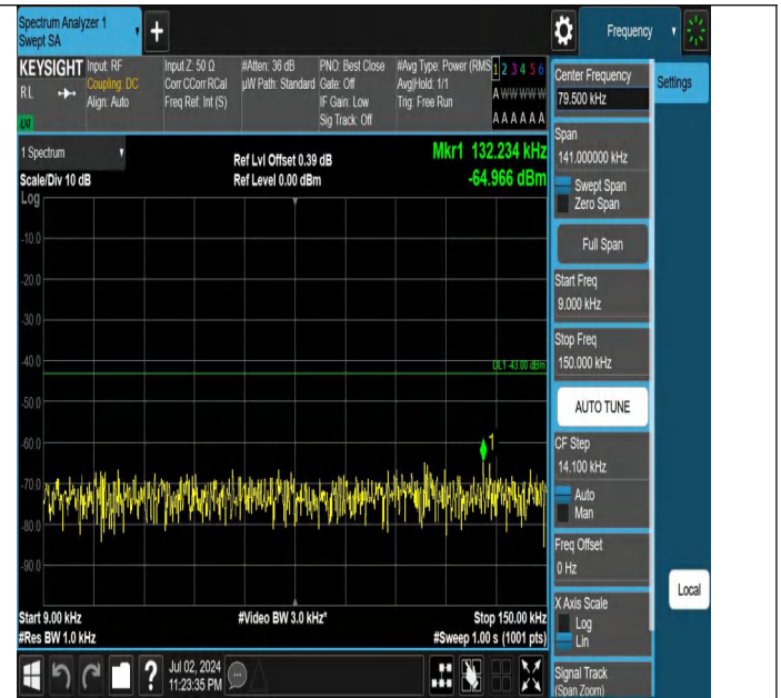
Band66-15MHz-QPSK-132597-1RB#74-0.009~0.15-PASS
