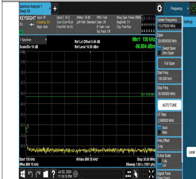
Band66-10MHz-QPSK-132322-1RB#49-0.15~30-PASS
