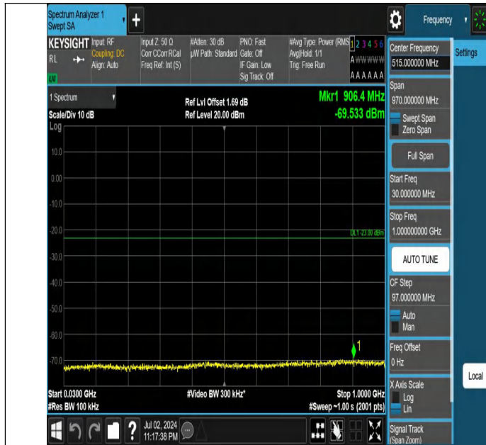
Band66-10MHz-QPSK-132022-1RB#0-30~1000-PASS
