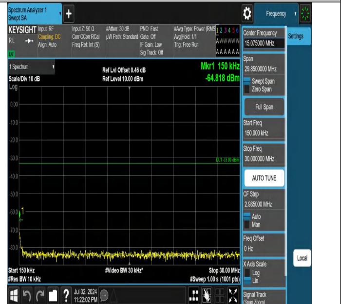
Band66-15MHz-QPSK-132322-1RB#0-0.15~30-PASS
