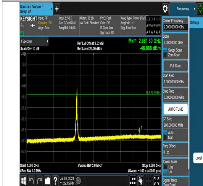
Band66-15MHz-QPSK-132322-1RB#74-1000~3000-PASS
