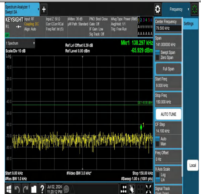
Band66-10MHz-QPSK-132622-1RB#49-0.009~0.15-PASS
