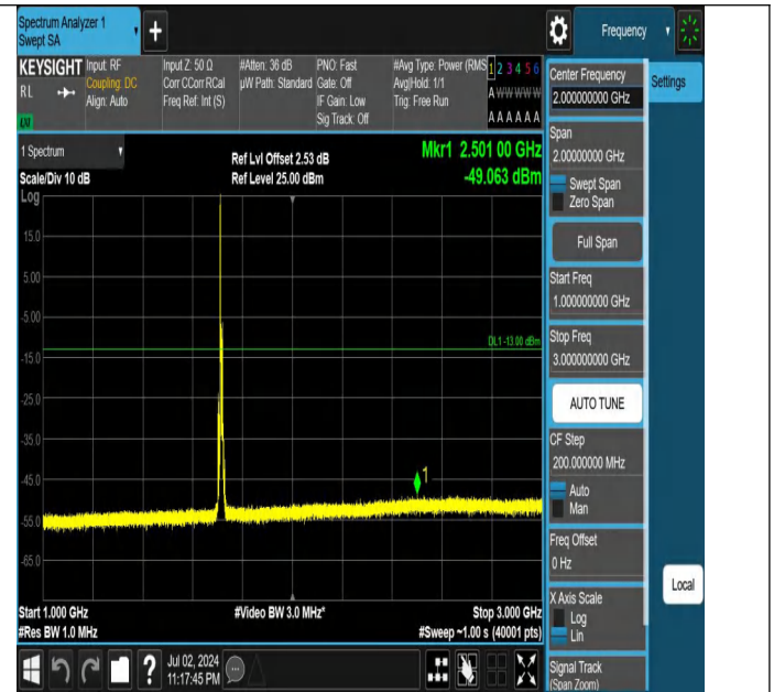
Band66-10MHz-QPSK-132022-1RB#0-1000~3000-PASS
