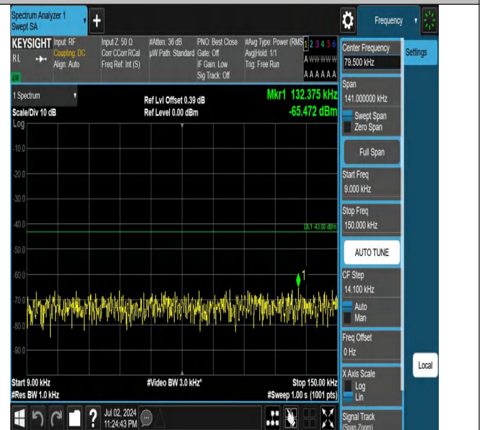
Band66-20MHz-QPSK-132072-1RB#99-0.009~0.15-PASS
