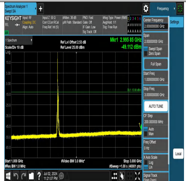
Band66-15MHz-QPSK-132047-1RB#0-1000~3000-PASS
