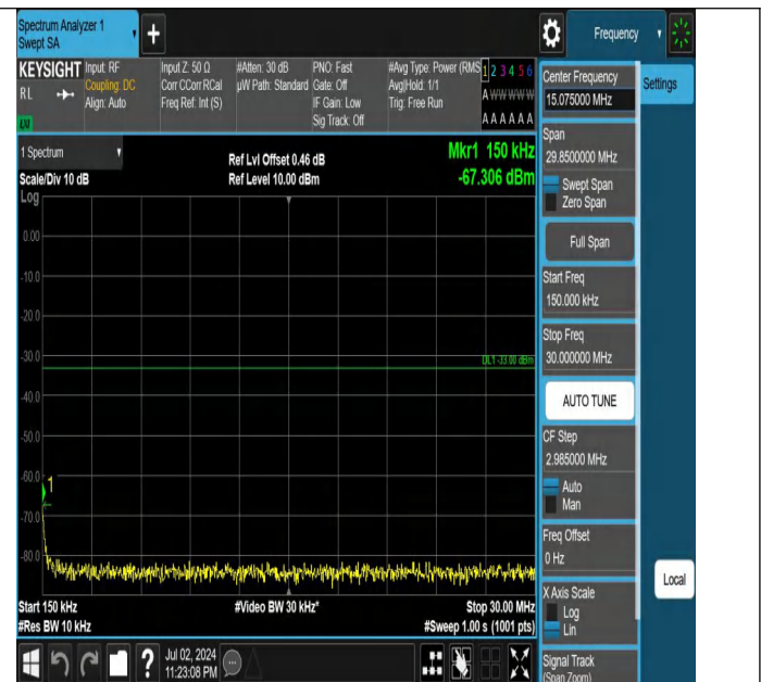
Band66-15MHz-QPSK-132597-1RB#0-0.15~30-PASS
