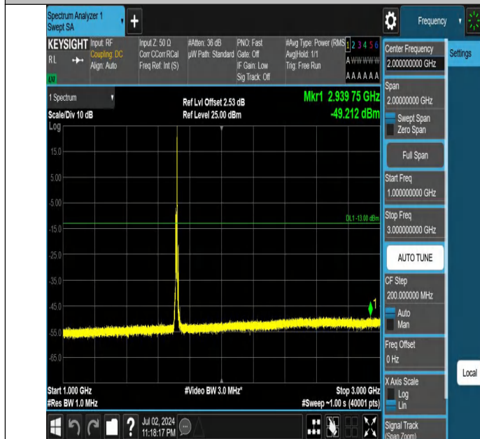
Band66-10MHz-QPSK-132022-1RB#49-1000~3000-PASS
