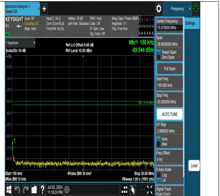
Band66-5MHz-QPSK-132647-1RB#0-0.15~30-PASS
