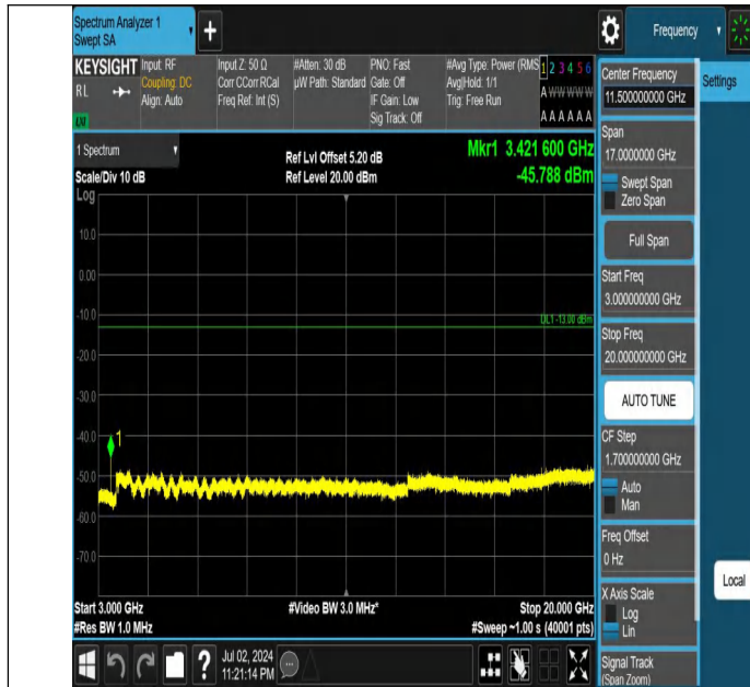
Band66-15MHz-QPSK-132047-1RB#0-3000~20000-PASS
