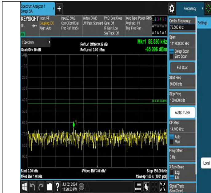
Band66-15MHz-QPSK-132047-1RB#0-0.009~0.15-PASS
