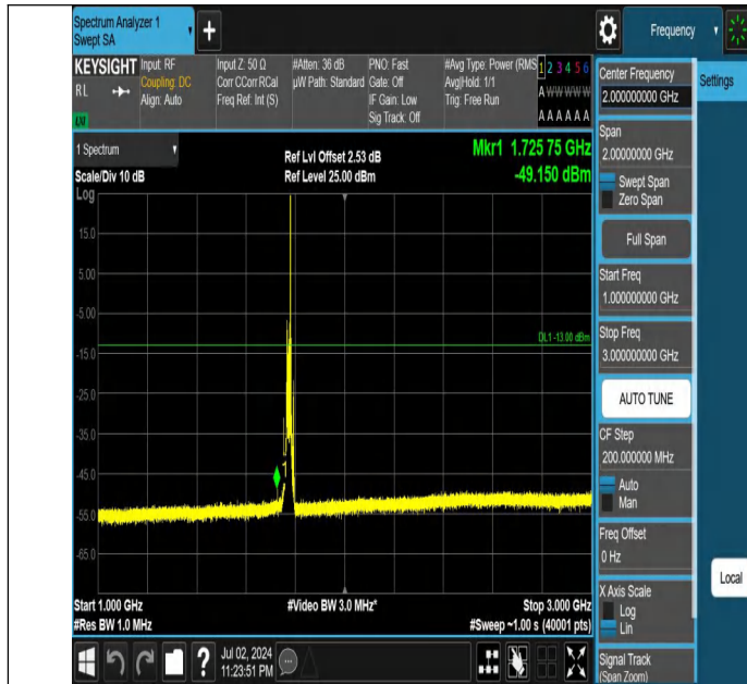
Band66-15MHz-QPSK-132597-1RB#74-1000~3000-PASS
