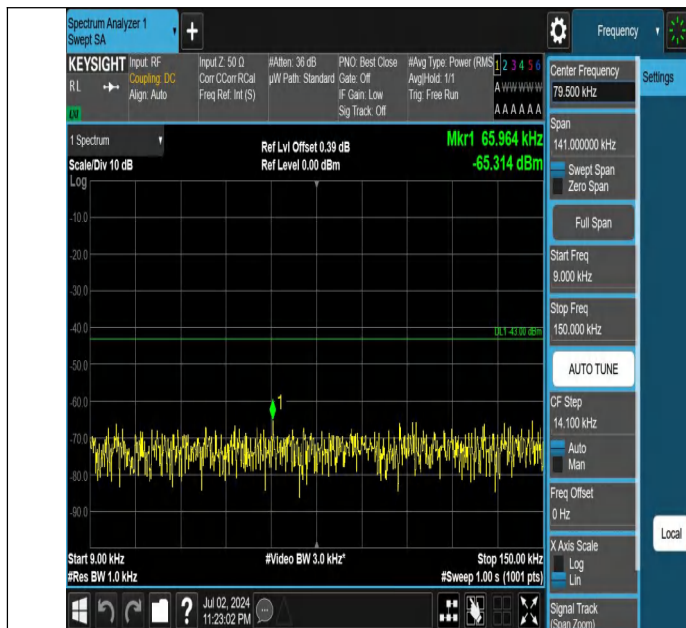
Band66-15MHz-QPSK-132597-1RB#0-0.009~0.15-PASS
