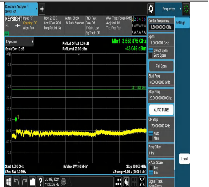
Band66-10MHz-QPSK-132622-1RB#49-3000~20000-PASS
