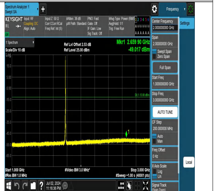
Band66-5MHz-QPSK-132647-1RB#0-1000~3000-PASS
