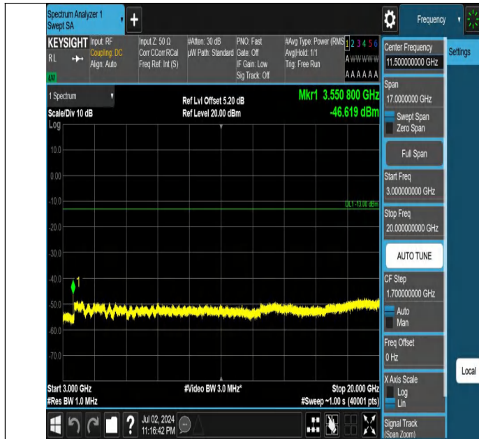
Band66-5MHz-QPSK-132647-1RB#0-3000~20000-PASS
