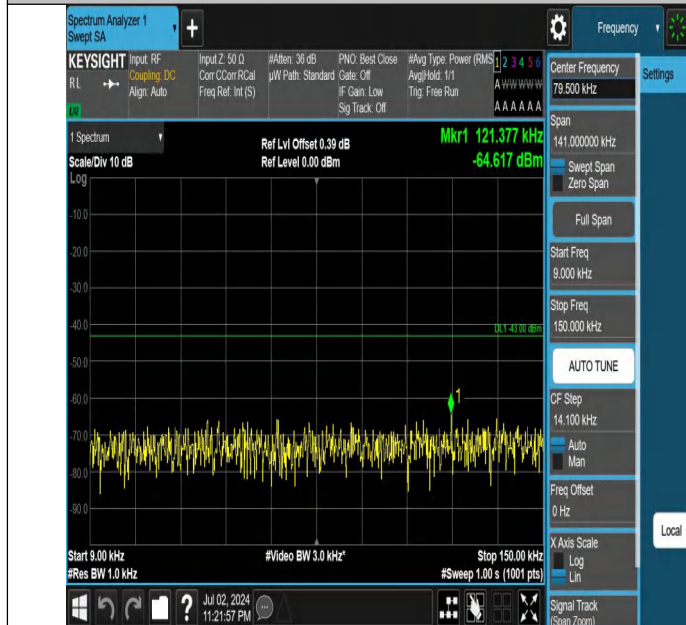
Band66-15MHz-QPSK-132322-1RB#0-0.009~0.15-PASS
