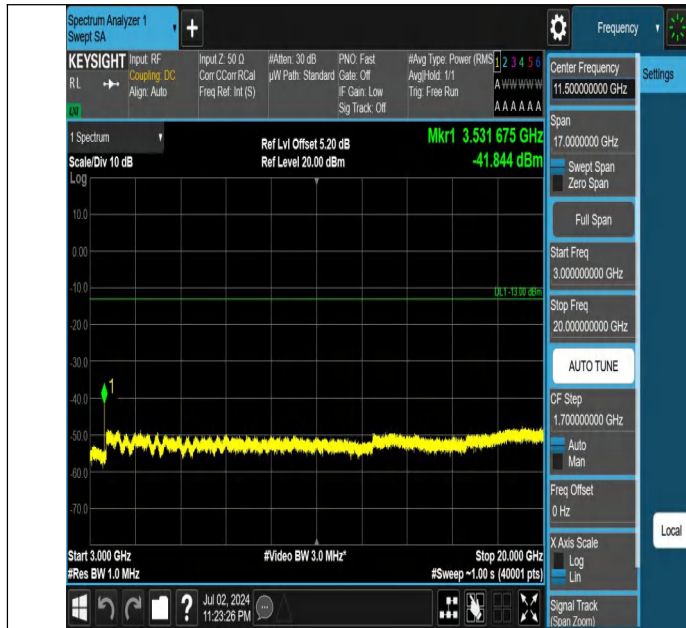
Band66-15MHz-QPSK-132597-1RB#0-3000~20000-PASS
