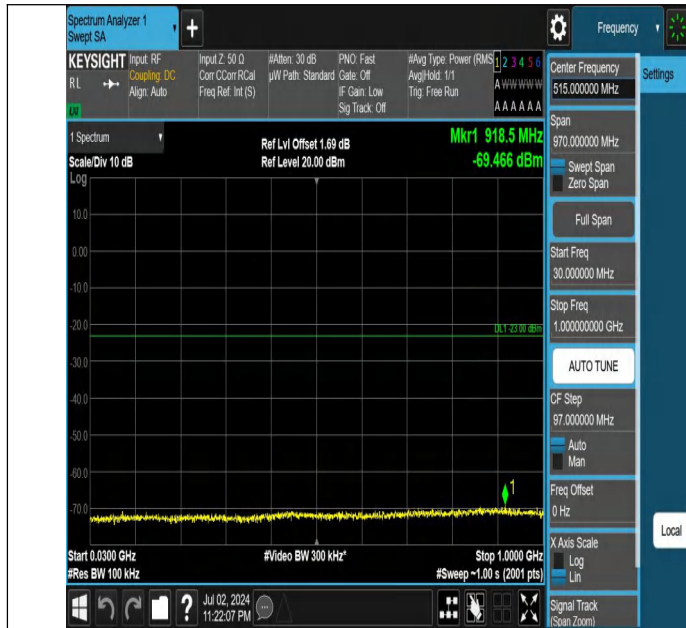
Band66-15MHz-QPSK-132322-1RB#0-30~1000-PASS
