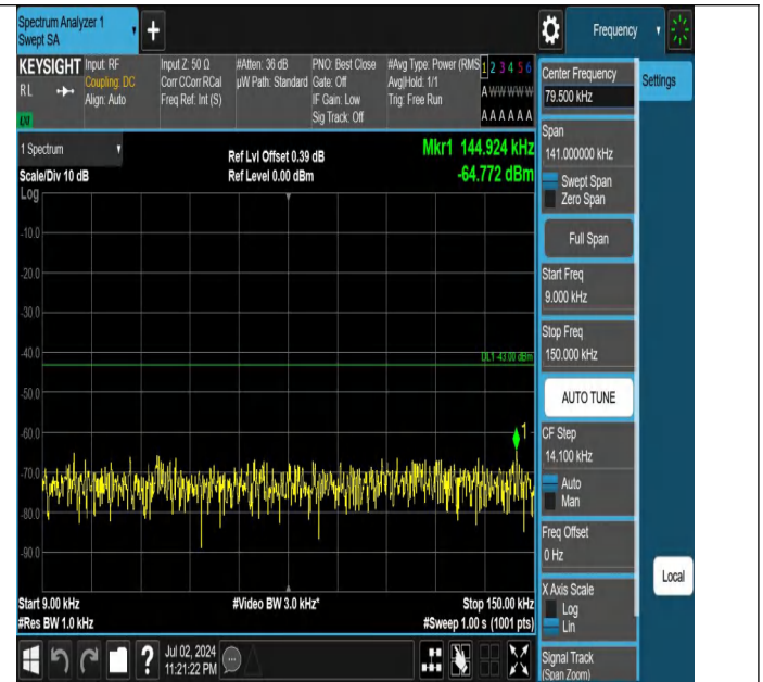
Band66-15MHz-QPSK-132047-1RB#74-0.009~0.15-PASS
