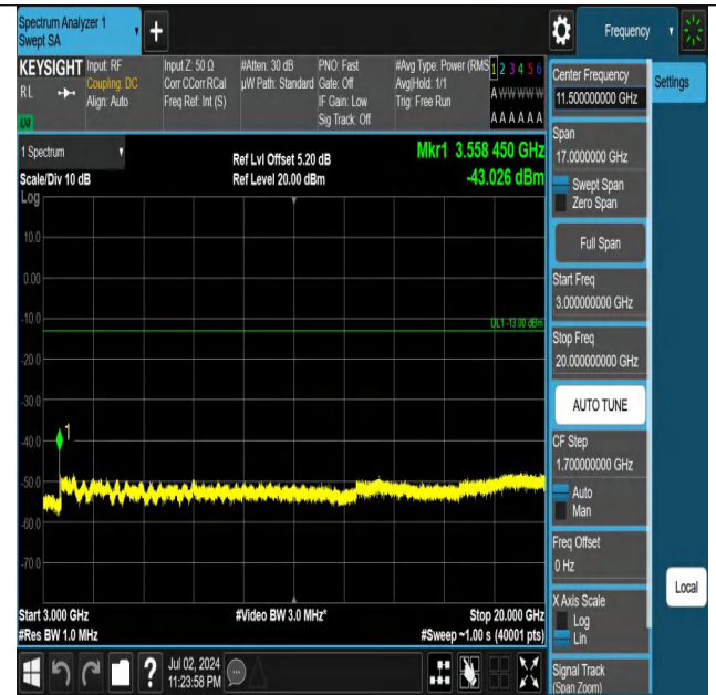
Band66-15MHz-QPSK-132597-1RB#74-3000~20000-PASS
