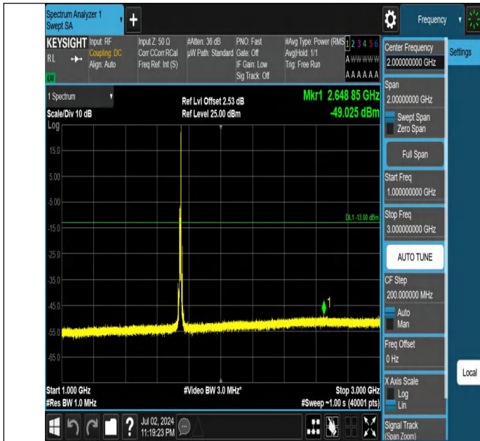
Band66-10MHz-QPSK-132322-1RB#49-1000~3000-PASS
