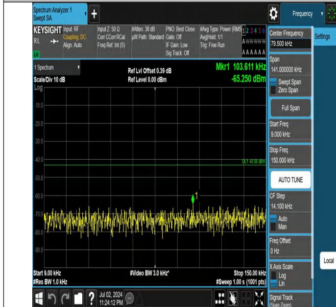
Band66-20MHz-QPSK-132072-1RB#0-0.009~0.15-PASS
