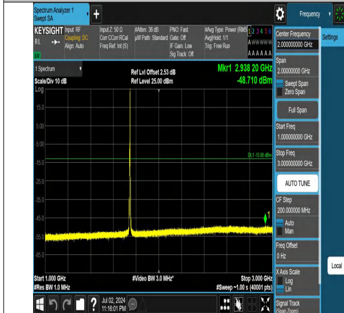
Band66-5MHz-QPSK-132322-1RB#24-1000~3000-PASS
