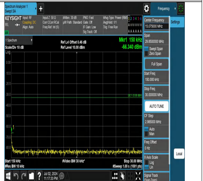
Band66-10MHz-QPSK-132022-1RB#0-0.15~30-PASS
