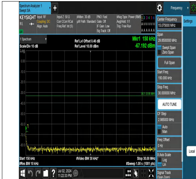
Band66-15MHz-QPSK-132322-1RB#74-0.15~30-PASS
