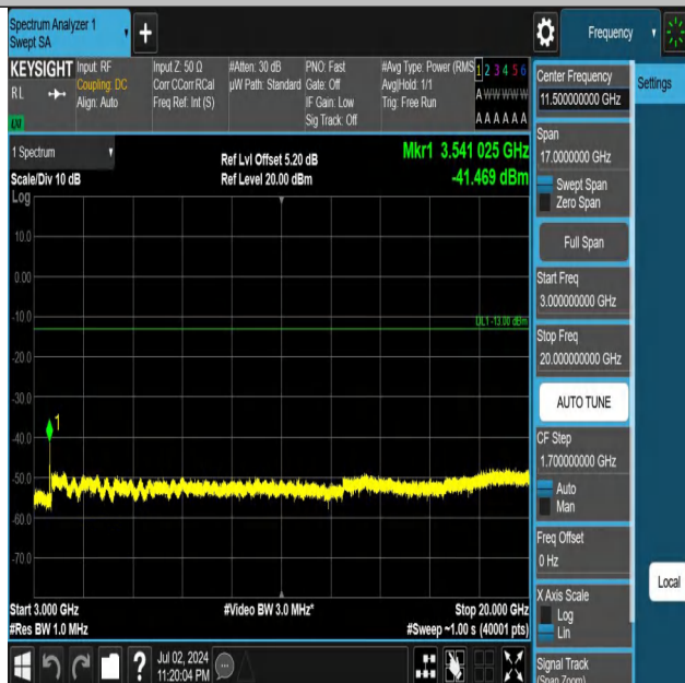
Band66-10MHz-QPSK-132622-1RB#0-3000~20000-PASS
