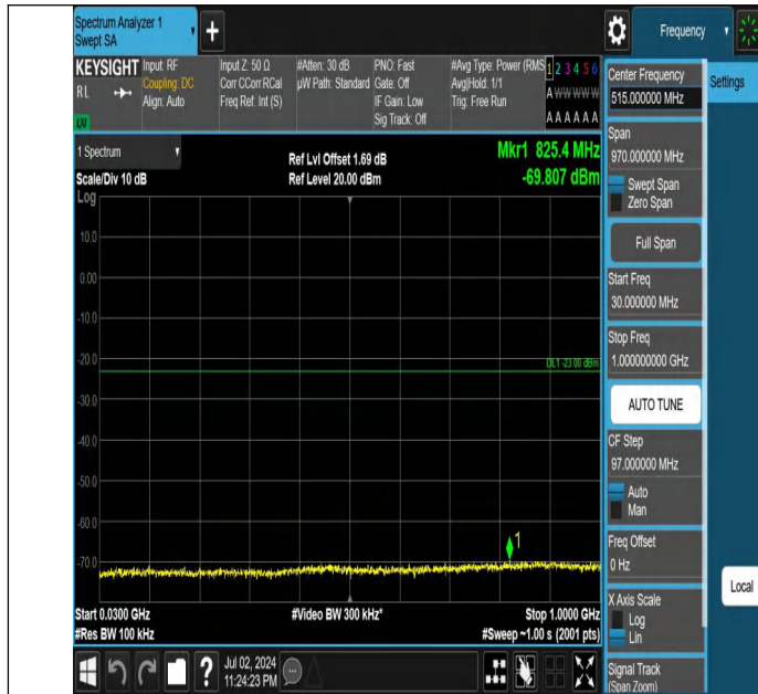
Band66-20MHz-QPSK-132072-1RB#0-30~1000-PASS
