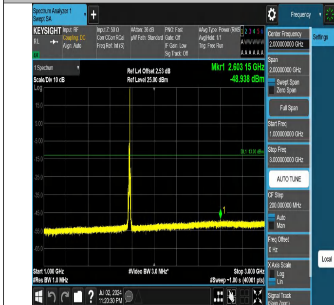
Band66-10MHz-QPSK-132622-1RB#49-1000~3000-PASS
