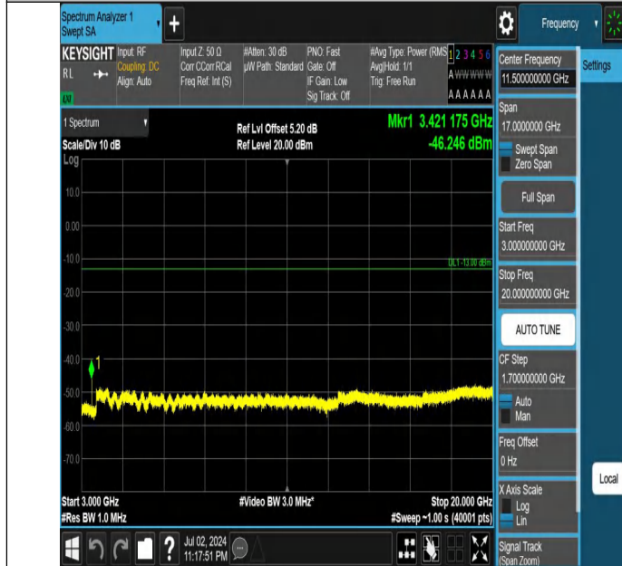
Band66-10MHz-QPSK-132022-1RB#0-3000~20000-PASS
