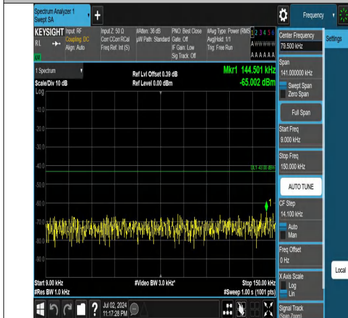
Band66-10MHz-QPSK-132022-1RB#0-0.009~0.15-PASS
