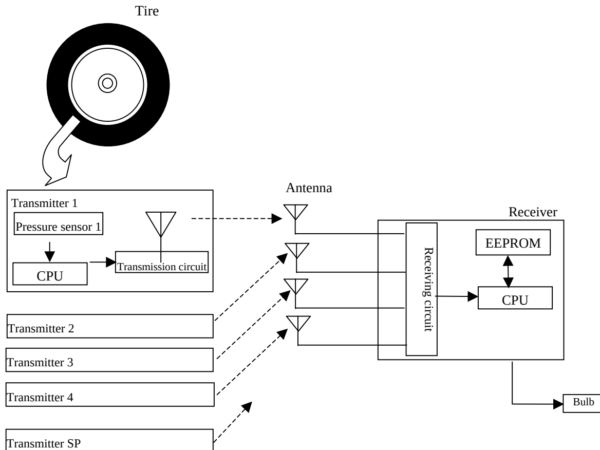
Figure 2-1 System Architecture
