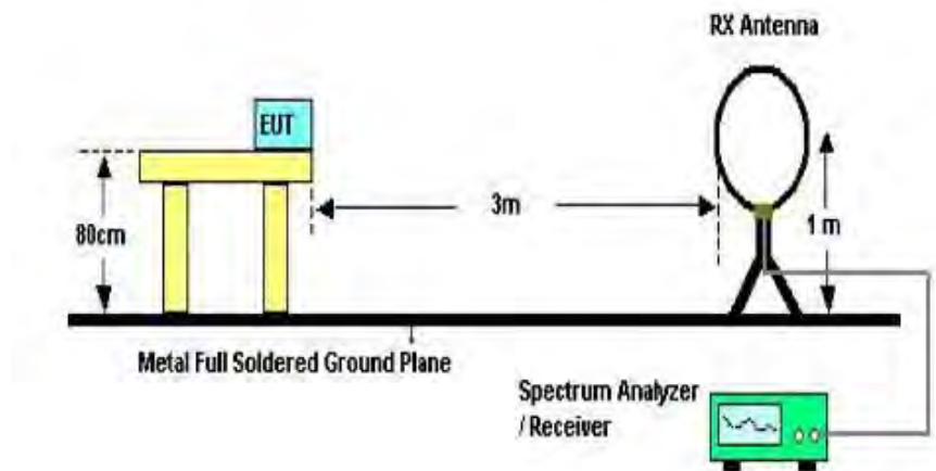
Below 30MHz Test Setup
