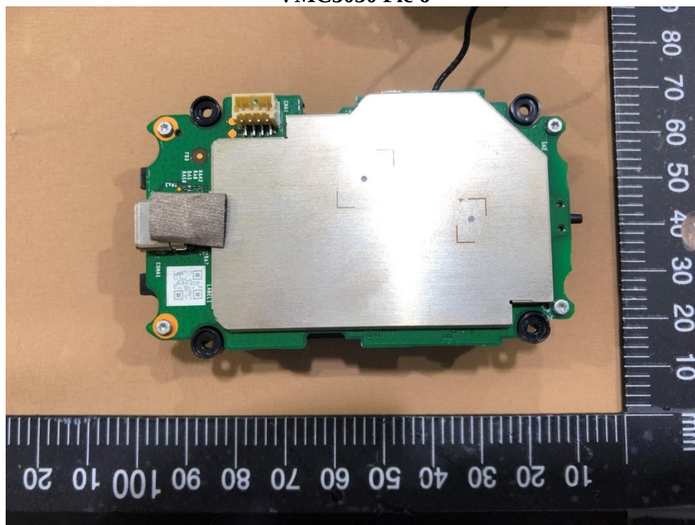
VMC3050 Pic 6
