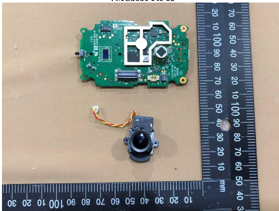
VMC3050 Pic 18
