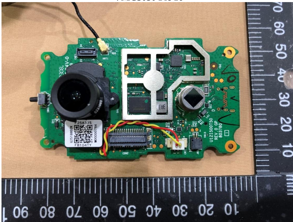
VMC3050 Pic 16
