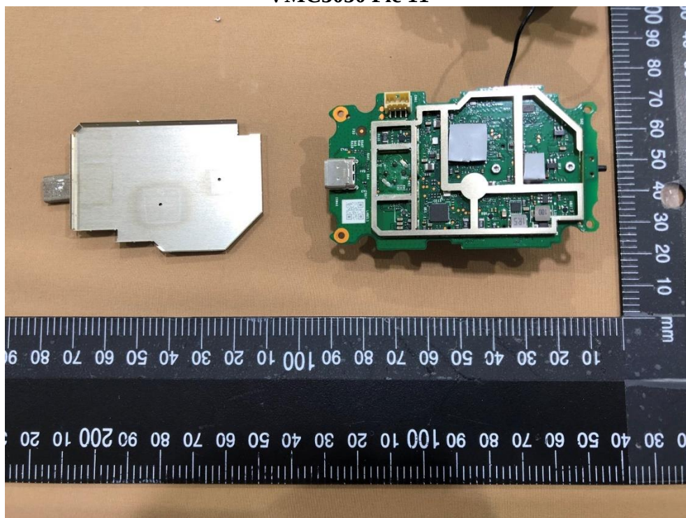
VMC3050 Pic 11
