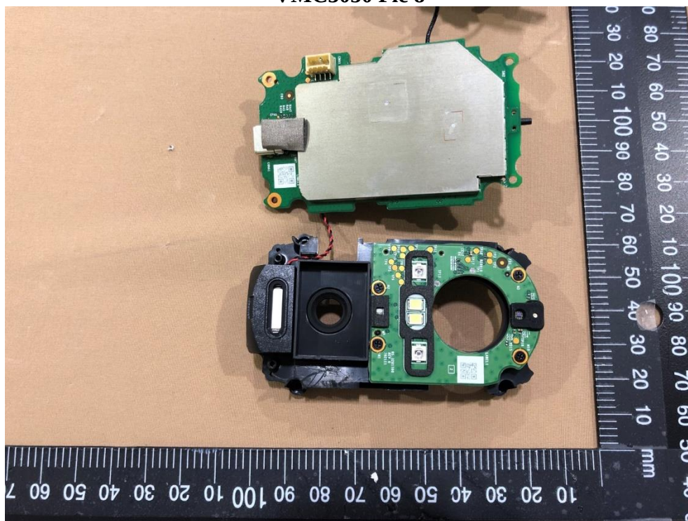
VMC3050 Pic 8
