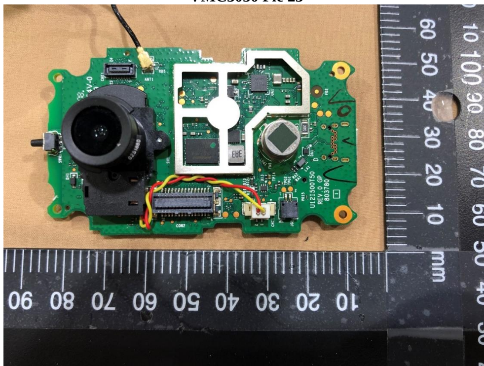
VMC3050 Pic 23
