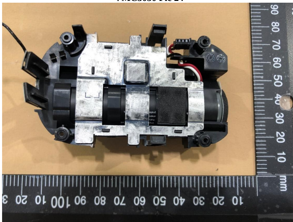
VMC3050 Pic 24
