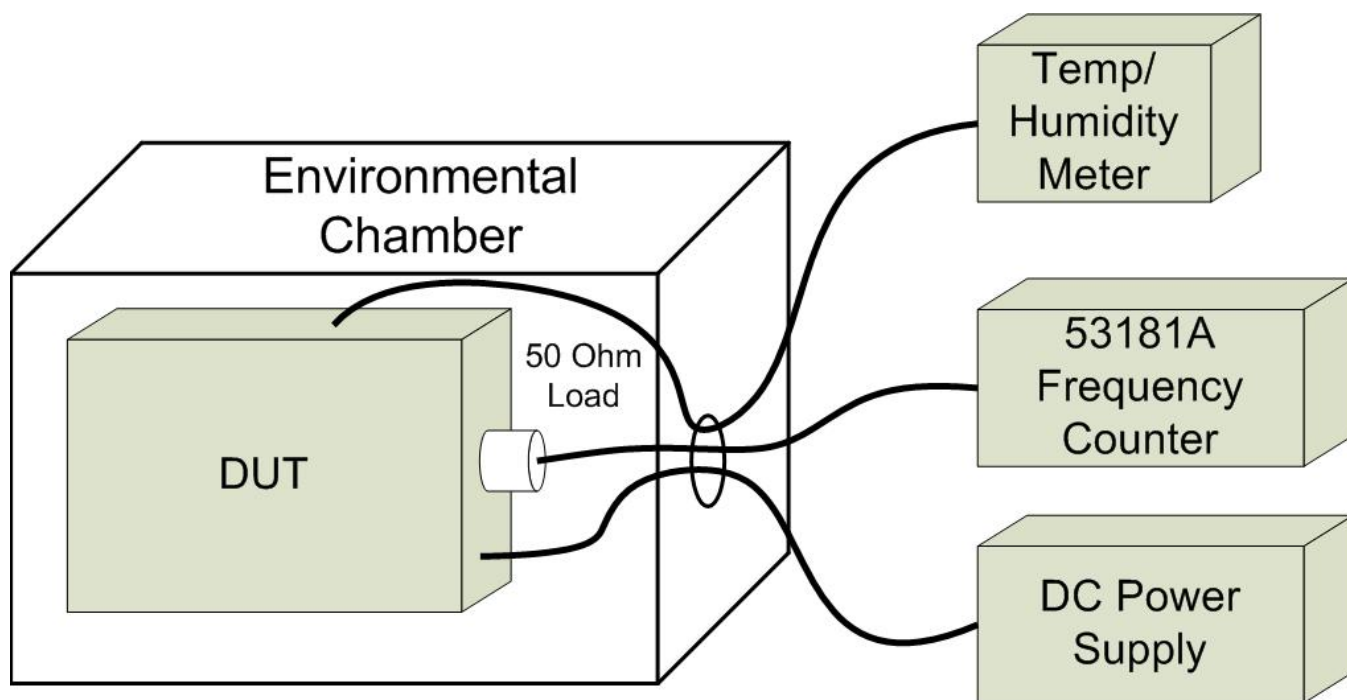
Figure A.4 – Test Setup Frequency Stability Measurements
