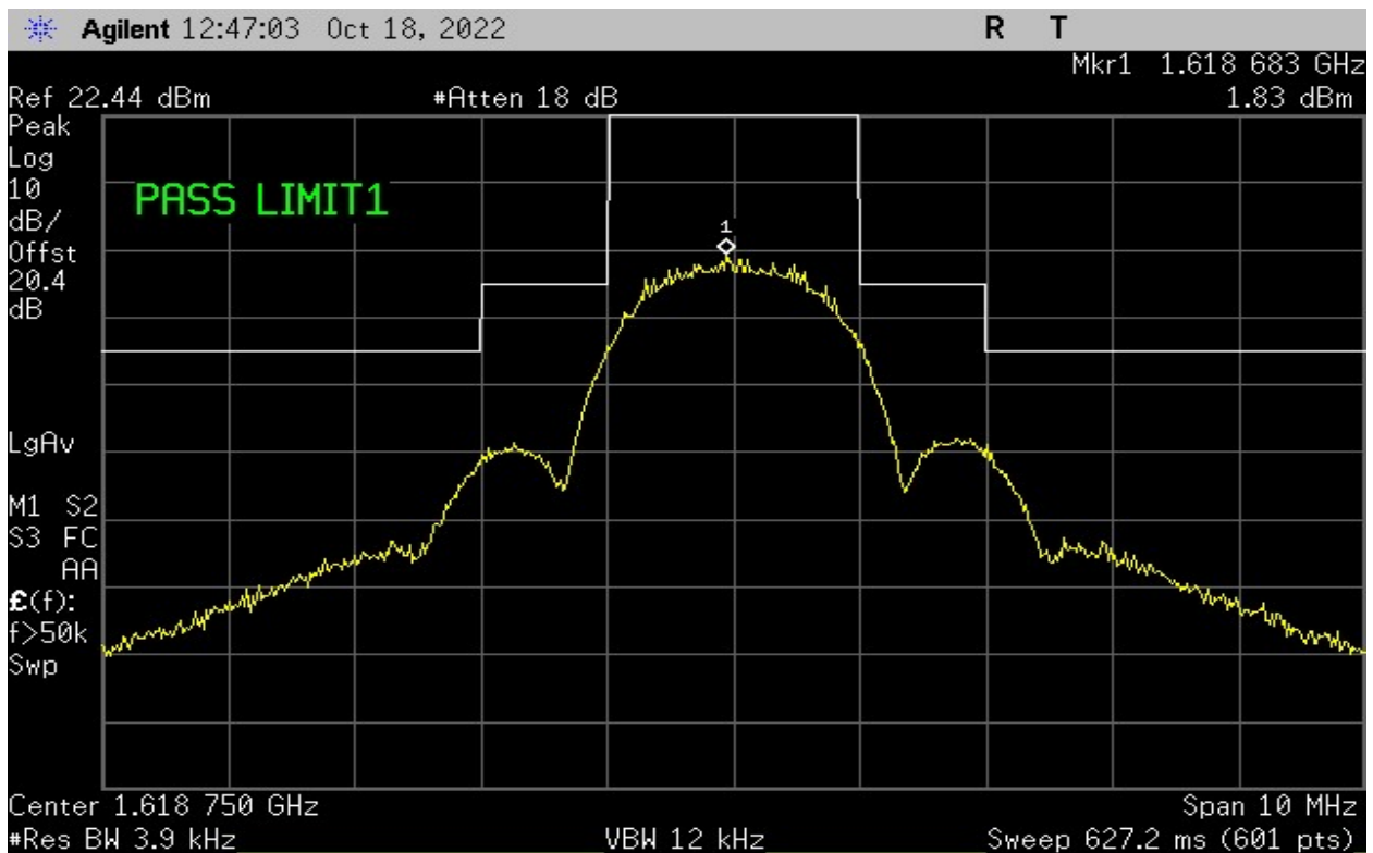
Plot 4 – Emission Mask - High Channel
