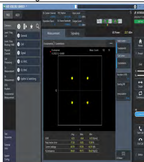
1-N77-3700-3980-30-100-M-6-CP-QPSK-Outer_Full-273@0-Ant1-see graph-PASS
