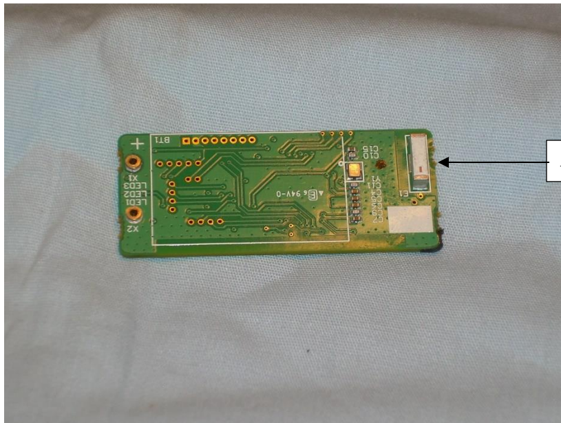
Photograph 10 – Bottom View of the PCB
