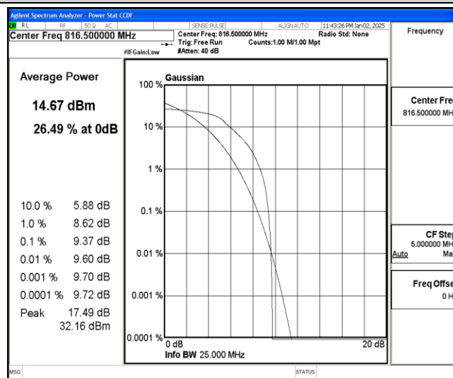
Band26-5MHz-16QAM-26715-6-0-Low-9.37-&lt;=13-PASS
