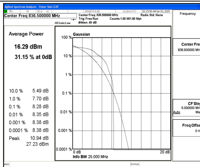
Band26-10MHz-QPSK-26915-1-0-Low-8.28-&lt;=13-PASS
