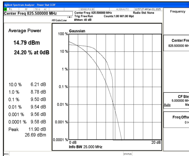
Band26-3MHz-QPSK-26805-1-0-Low-9.50-&lt;=13-PASS
