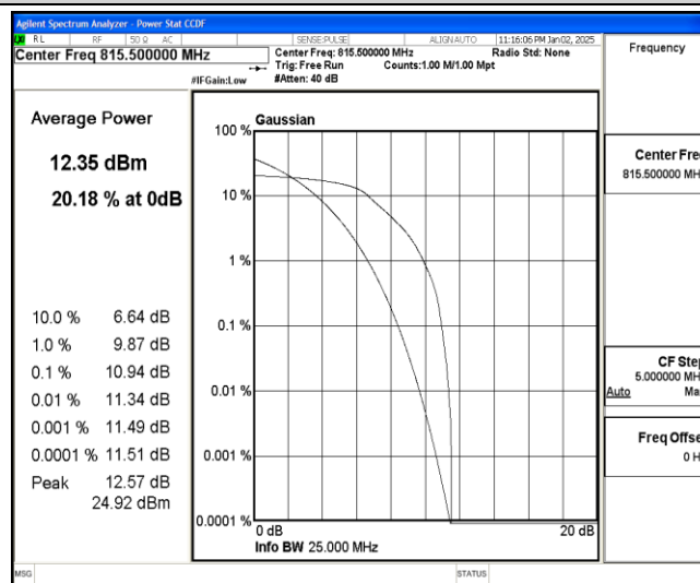
Band26-3MHz-QPSK-26705-6-0-Low-10.94-&lt;=13-PASS
