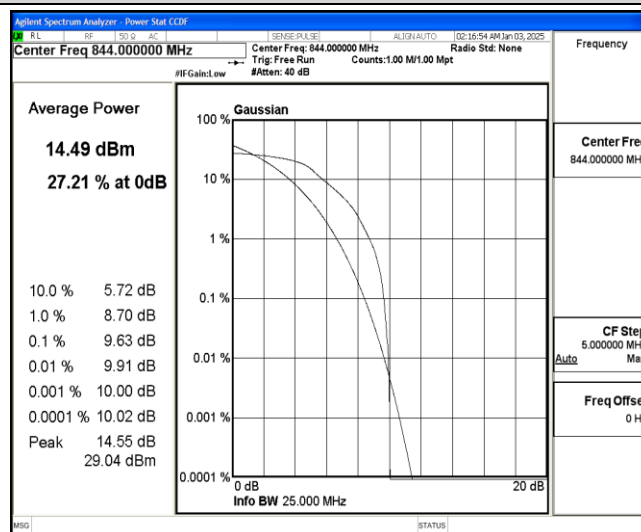
Band26-10MHz-QPSK-26990-6-0-High-9.63-&lt;=13-PASS
