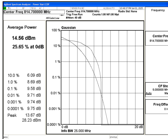
Band26-1.4MHz-16QAM-26697-1-0-Low-9.58-&lt;=13-PASS
