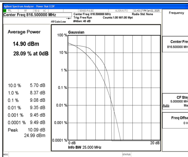
Band26-5MHz-QPSK-26715-6-0-Low-9.08-&lt;=13-PASS
