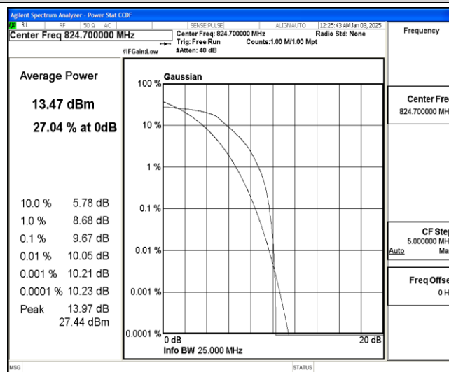
Band26-1.4MHz-QPSK-26797-6-0-Low-9.67-&lt;=13-PASS
