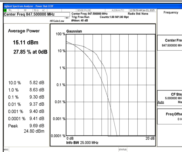
Band26-3MHz-16QAM-27025-1-0-High-9.30-&lt;=13-PASS
