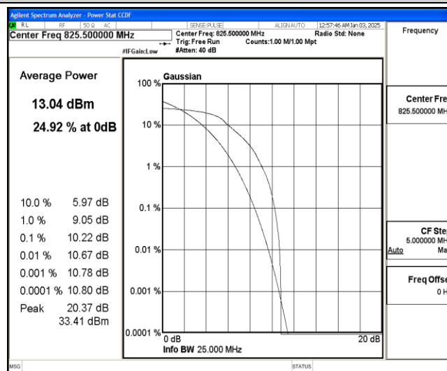
Band26-3MHz-QPSK-26805-6-0-Low-10.22-&lt;=13-PASS
