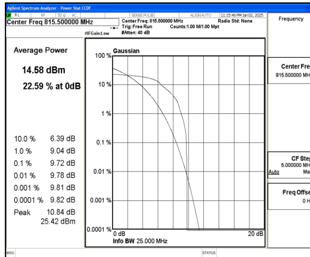
Band26-3MHz-QPSK-26705-1-0-Low-9.72-&lt;=13-PASS
