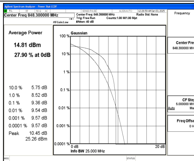
Band26-1.4MHz-16QAM-27033-1-0-High-9.36-&lt;=13-PASS
