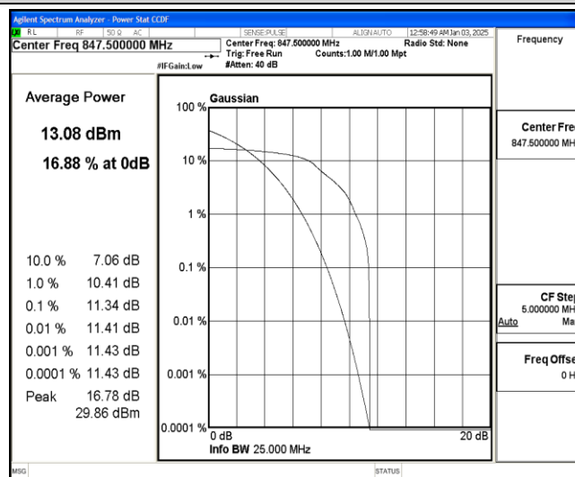
Band26-3MHz-QPSK-27025-1-0-High-11.34-&lt;=13-PASS
