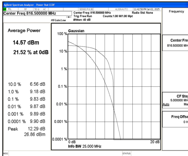
Band26-5MHz-QPSK-26715-1-0-Low-9.83-&lt;=13-PASS
