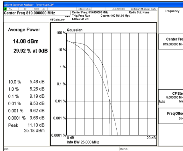
Band26-1.4MHz-QPSK-26740-6-0-Low-9.19-&lt;=13-PASS
