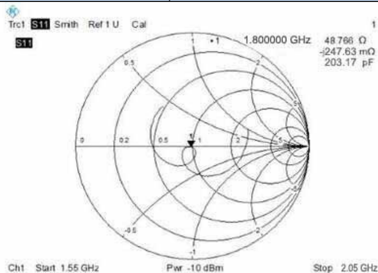
Impedance
