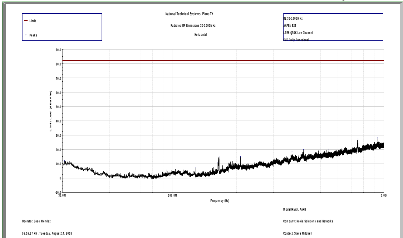
Radiated Spurious Emissions 30MHz-1GHz Horizontal at 3m LTE5-QPSK-Low Channel
