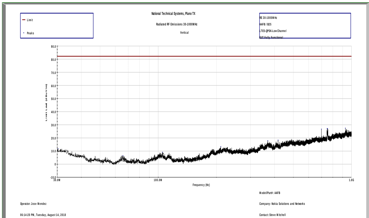
Radiated Spurious Emissions 30MHz-1GHz Vertical at 3m LTE5-QPSK-Low Channel
