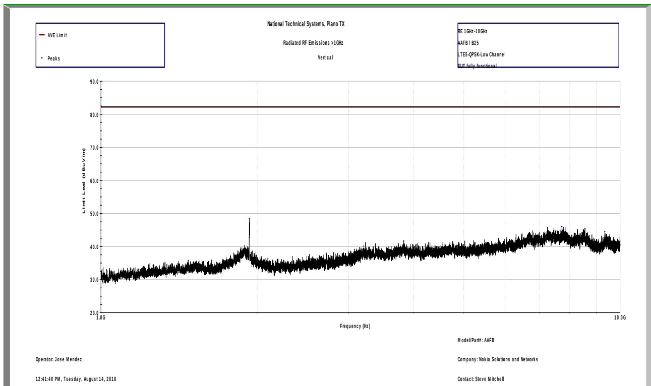
Radiated Spurious Emissions 1-10GHz Vertical at 3m LTE5-QPSK-Low Channel
