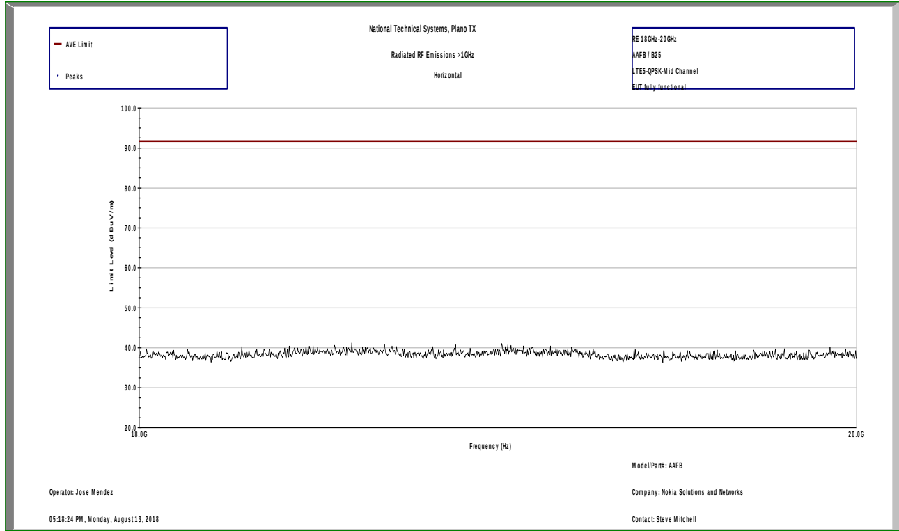
Radiated Spurious Emissions 18-20GHz Horizontal at 1m LTE5-QPSK-Mid Channel
