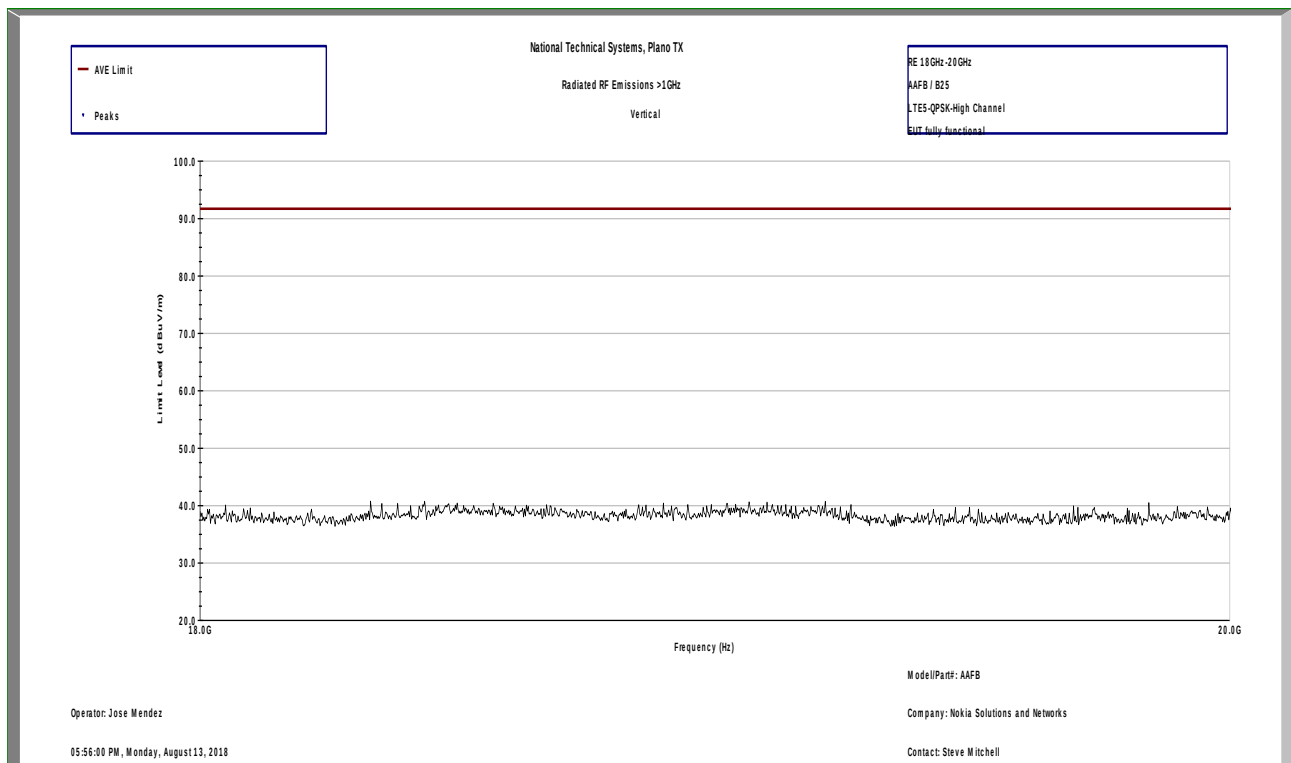
Radiated Spurious Emissions 18-20GHz Vertical at 1m LTE5-QPSK-High Channel
