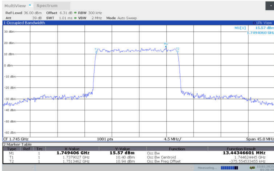
n66,15MHz Bandwidth,DFT-s-16QAM (99% OBW)
