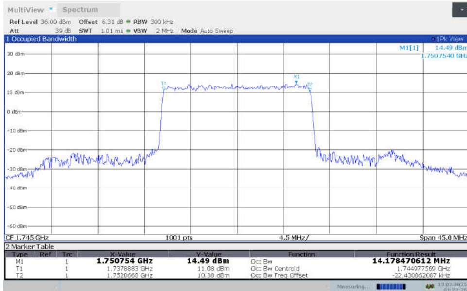
n66,15MHz Bandwidth,CP-16QAM (99% OBW)
