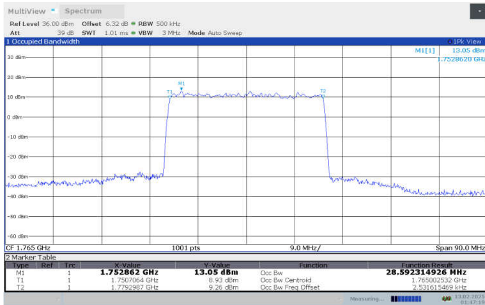
n66,30MHz Bandwidth,CP-QPSK (99% OBW)
