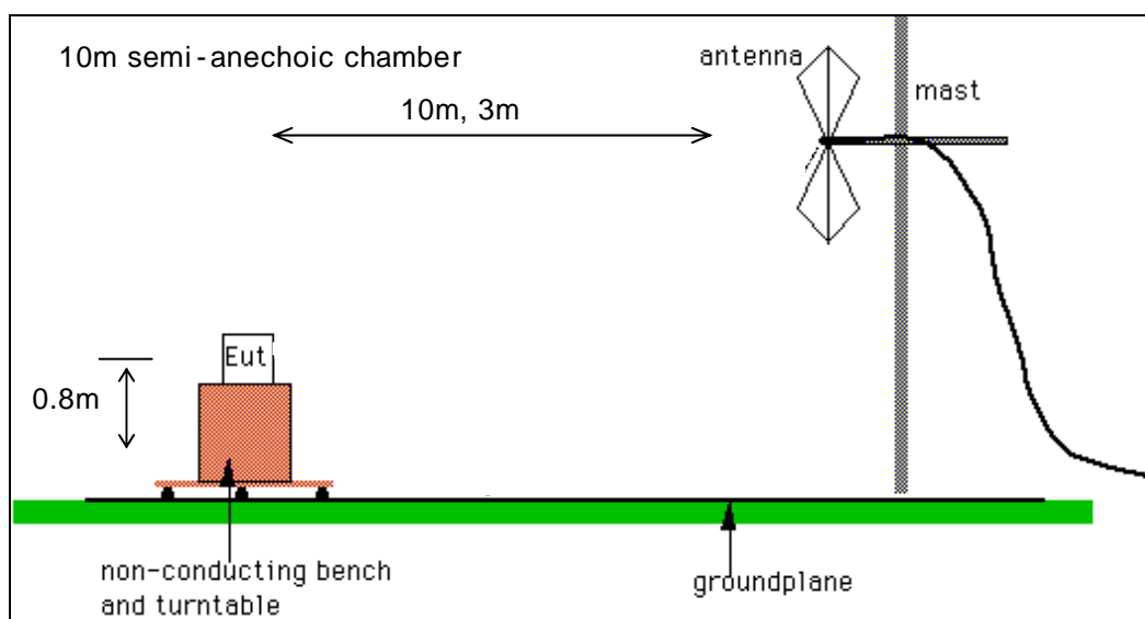
<General test set-up for radiated emissions>
