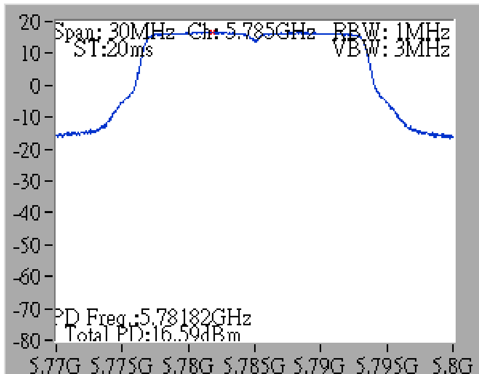
Power Density Plot on Configuration IEEE 802.11a / Chain 5 + Chain 6 + Chain 7 + Chain 8 / 5785 MHz
