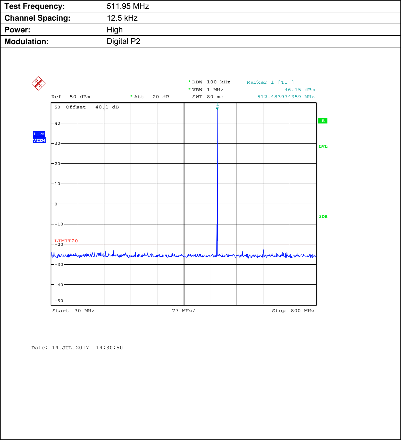
Plot 5.9.4.3.1. Conducted Transmitter Spurious Emissions for 511.95 MHz, High Power
