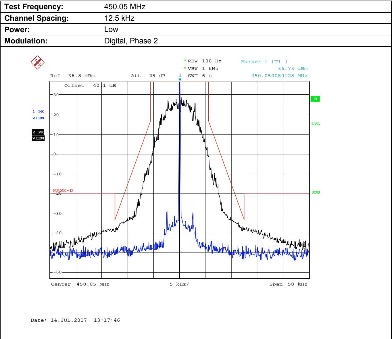
Plot 5.8.4.2.16. Emission Mask D, Low Power
