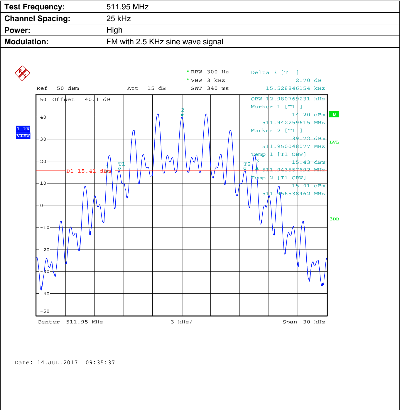
Plot 5.8.4.1.3. Occupied Bandwidth
