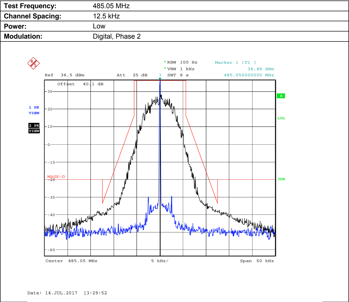
Plot 5.8.4.2.17. Emission Mask D, Low Power
