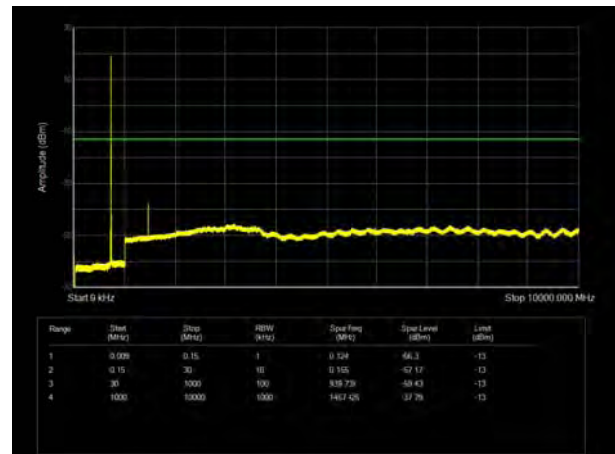
LTE Band 28 5MHz CH-Middle 9kHz~10.00GHz
