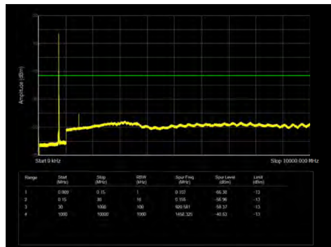
LTE Band 28 15MHz CH- Middle 9kHz~10.00GHz
