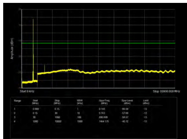
LTE Band 28 15MHz CH-High 9kHz~10.00GHz
