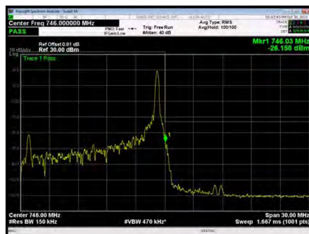
LTE Band 28 64QAM 15MHz CH-High, 100%RB
