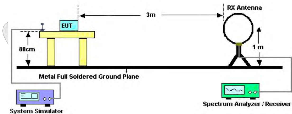
Figure 1. Below 30MHz
