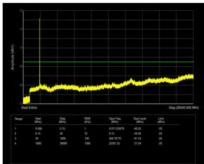
Band7 QPSK BW=5MHz Channel=21100 RB Size=25 Position=#0
