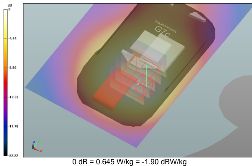
SAR Measurement Plot 45
