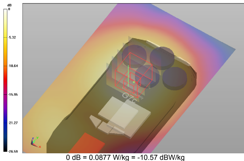
SAR Measurement Plot 42
