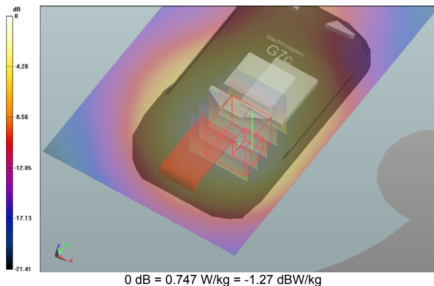
SAR Measurement Plot 46
