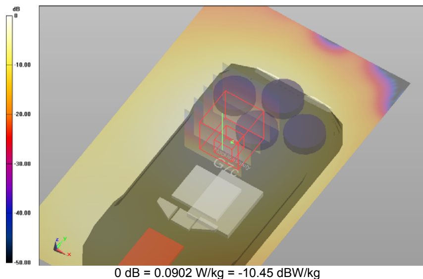
SAR Measurement Plot 40
