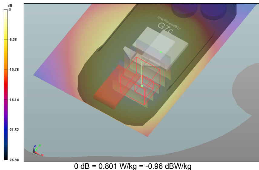
SAR Measurement Plot 53
