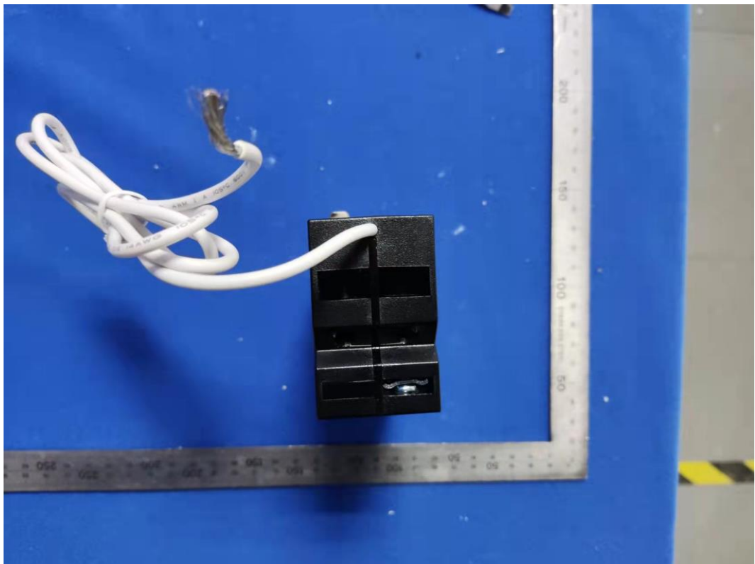
FIGURE 4 QO ADAPTIVE PHASE DIMMER, PIGTAIL (M/N: GPM-Q2APD10-21) RIGHT
