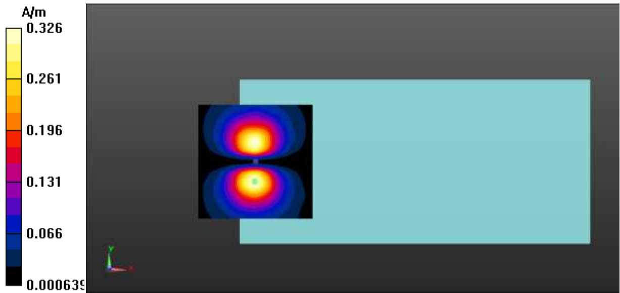
Fig A.24 T-Coil LTE-Band 66
