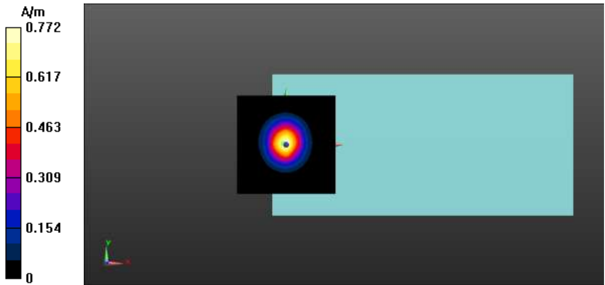
Fig A.11 T-Coil LTE-Band 2
