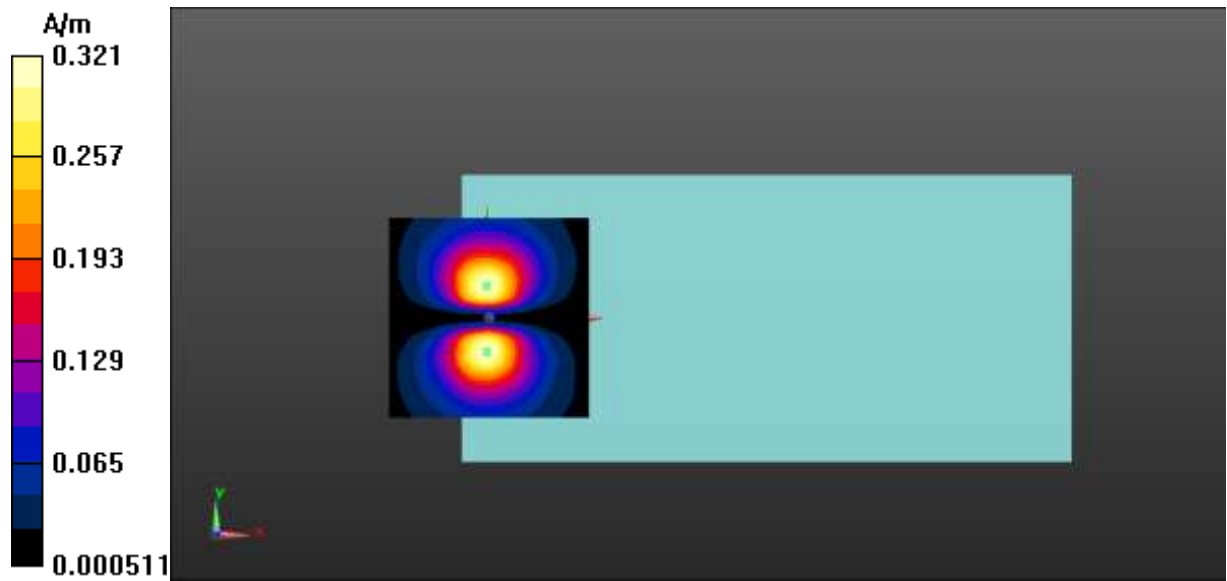
Fig A.14 T-Coil LTE-Band 4
