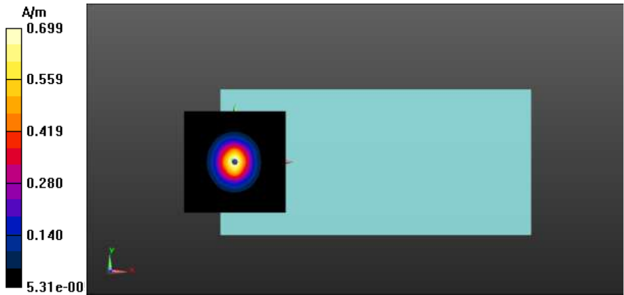
Fig A.3 T-Coil GSM 1900
