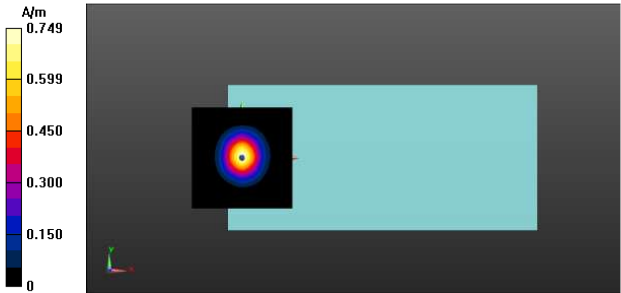
Fig A.13 T-Coil LTE-Band 4
