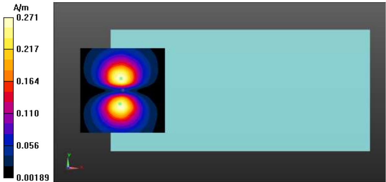
Fig A.2 T-Coil GSM 850
