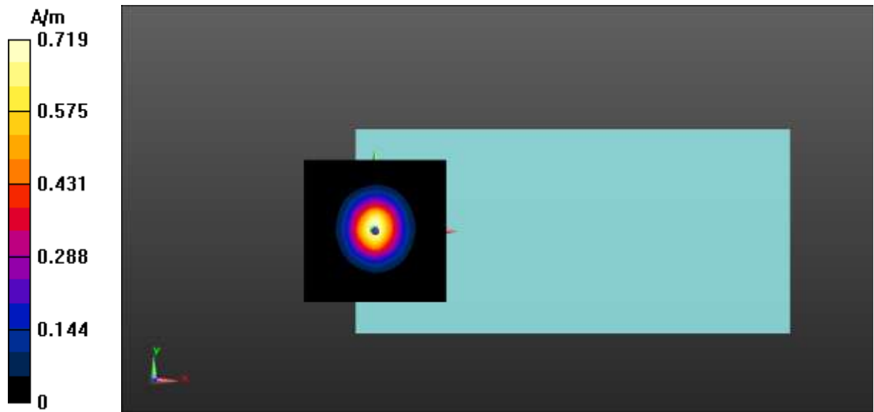
Fig A.15 T-Coil LTE-Band 5
