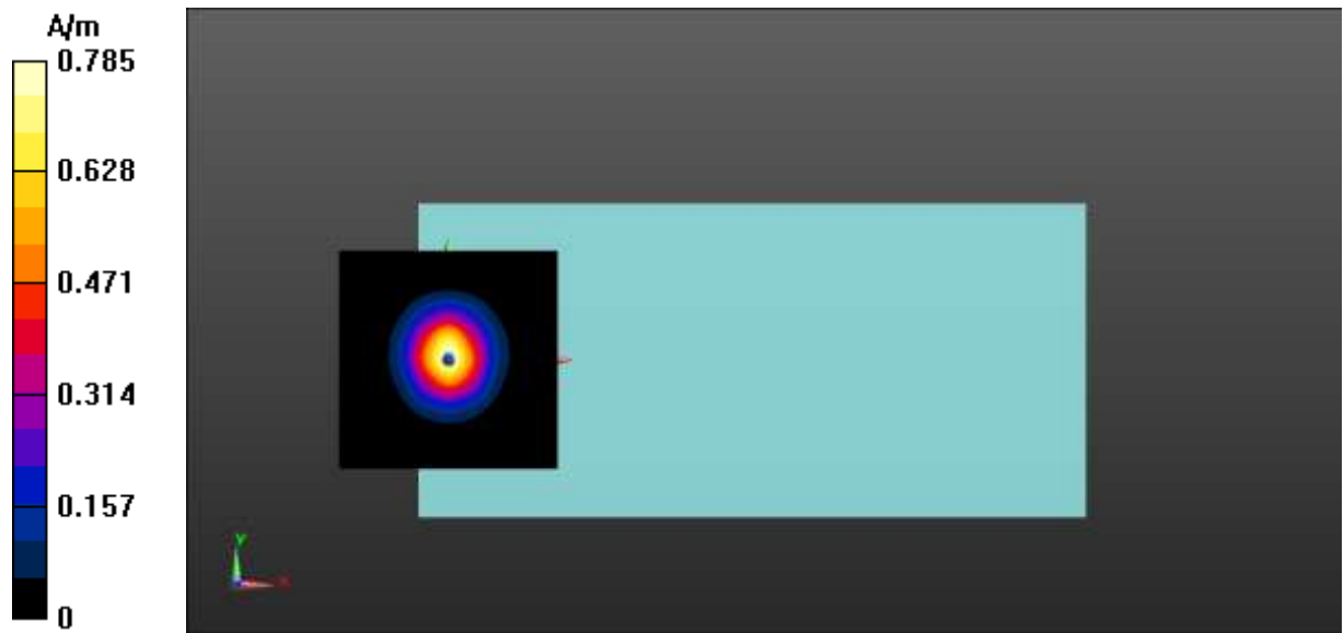
Fig A.17 T-Coil LTE-Band 12
