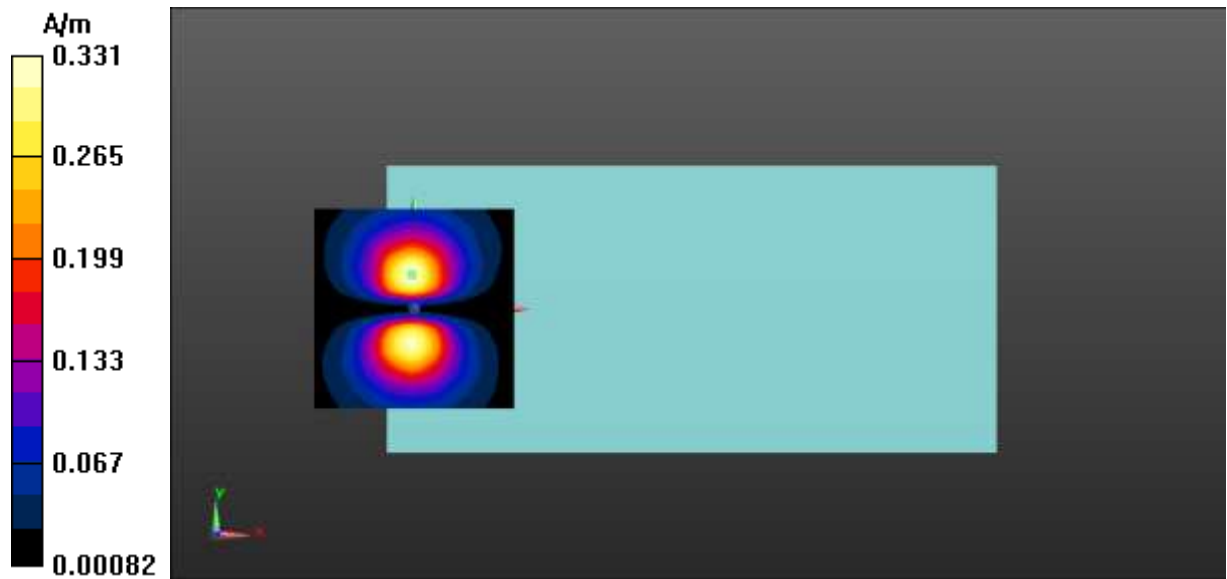
Fig A.20 T-Coil LTE-Band 13
