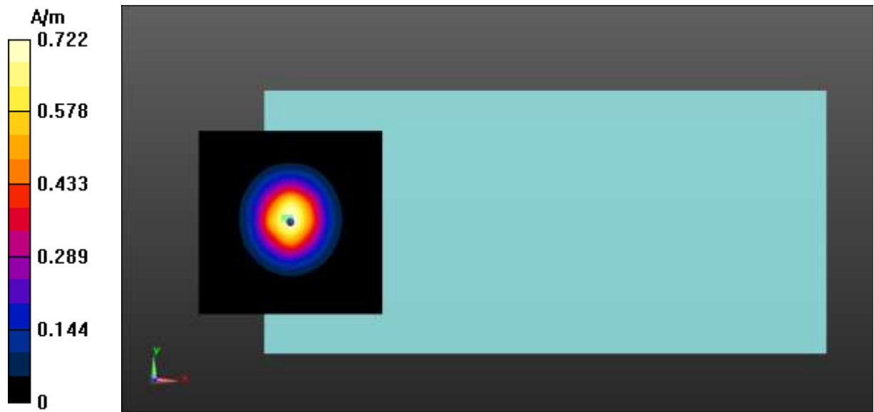
Fig A.21 T-Coil LTE-Band 17
