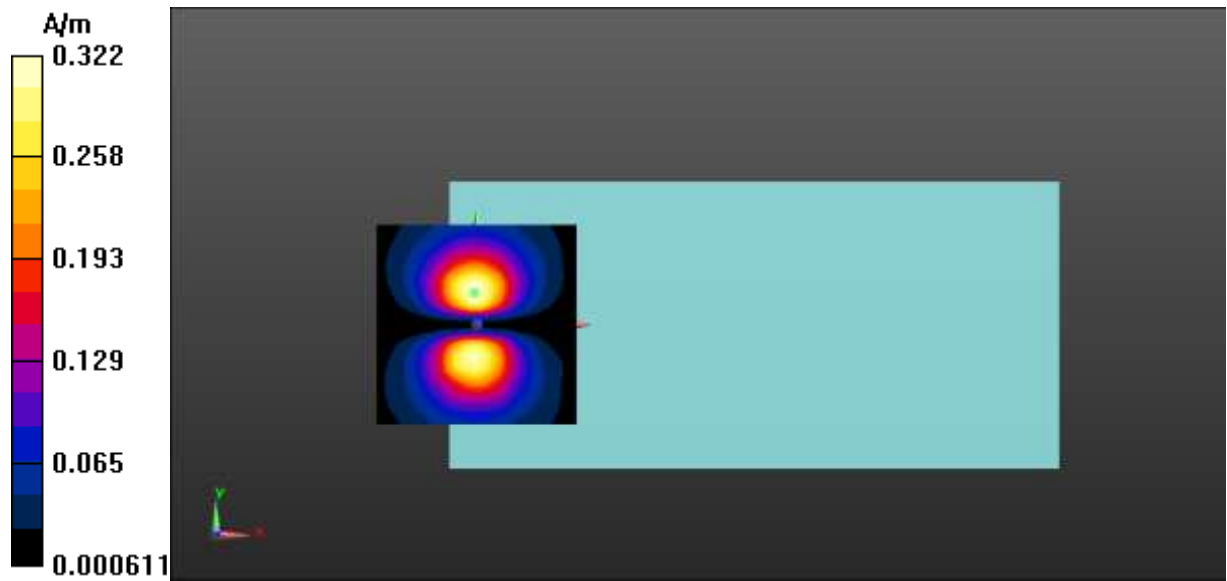
Fig A.16 T-Coil LTE-Band 5
