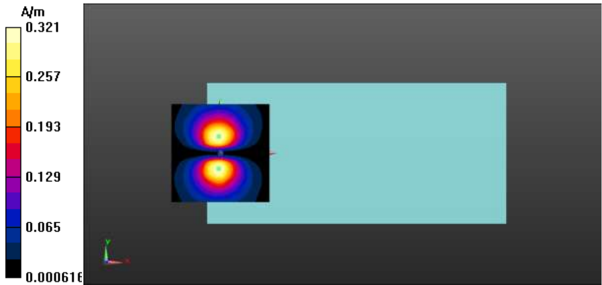
Fig A.12 T-Coil LTE-Band 2
