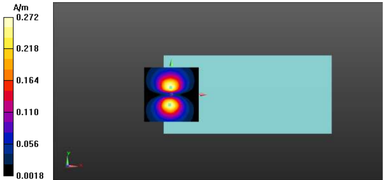
Fig A.4 T-Coil GSM 1900
