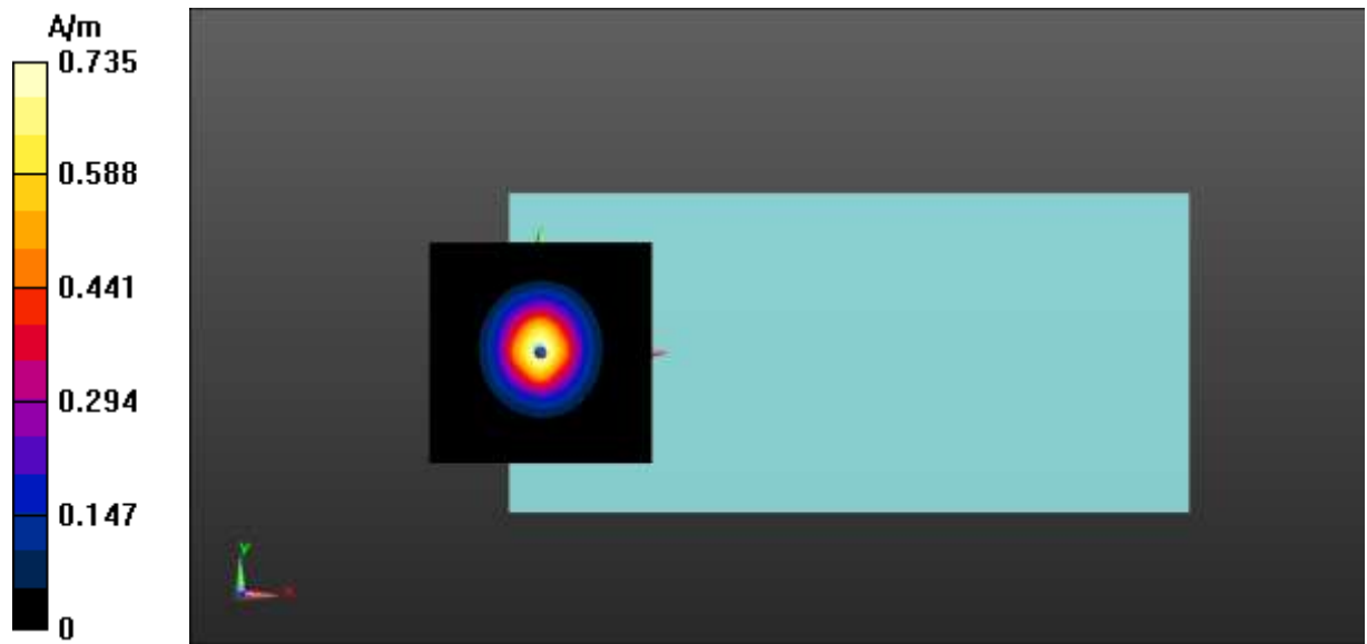
Fig A.19 T-Coil LTE-Band 13
