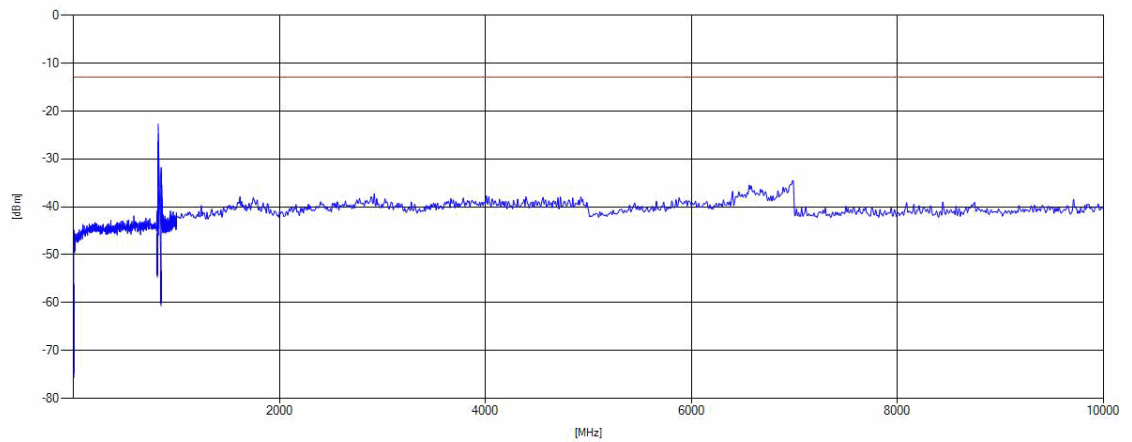
HSUPA FDD V Channel = low
