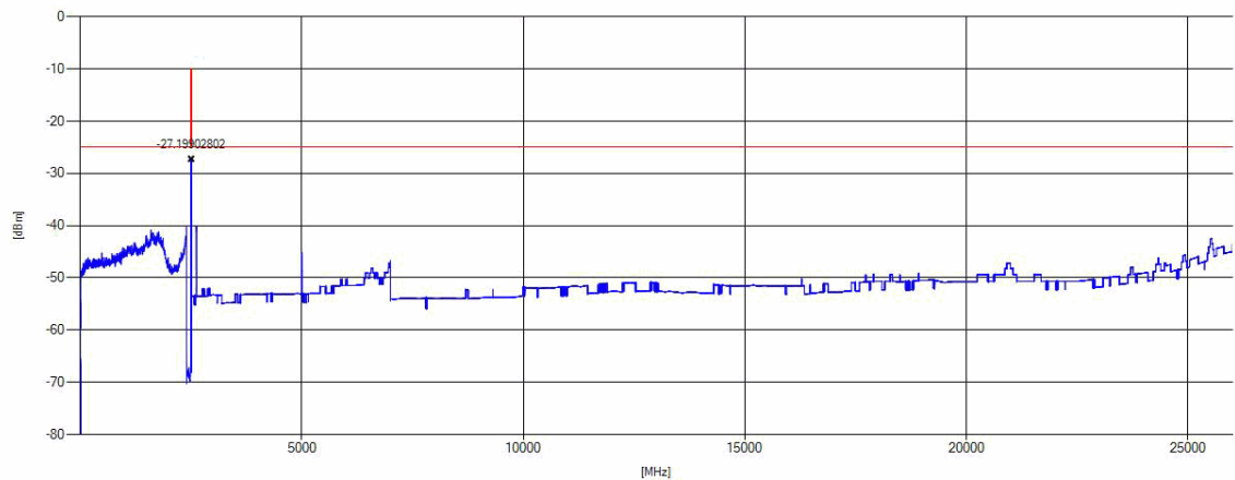
LTE eFDD7 QPSK Channel = low REMARK: compliant to FCC27.53m)4) and RSS-199 4.5
